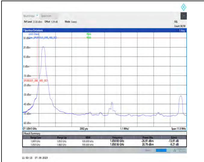
1-N25-PC3-15-10-L-1-DFT-PI2BPSK-Edge_1RB_Left-1@0-Ant2-1-seegraph-PASS-see graph
