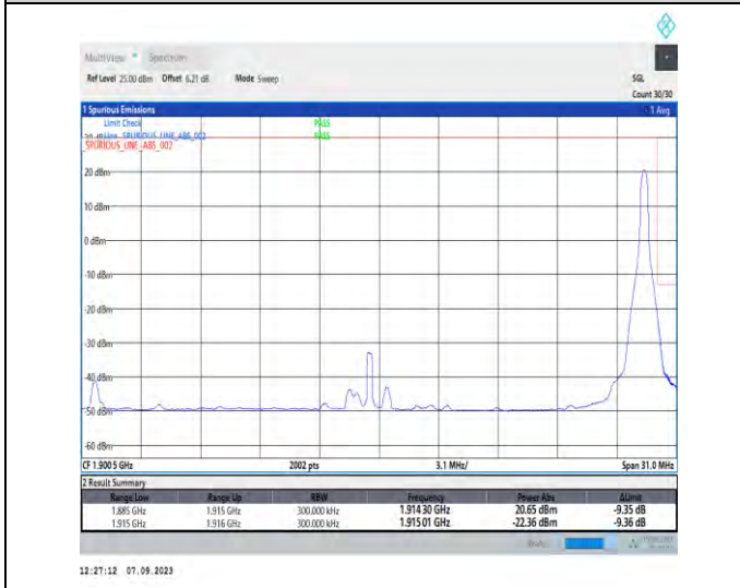
1-N25-PC3-15-30-H-5-CP-QPSK-Edge_1RB_Right-1@159-Ant2-1-seegraph-PASS-see graph
