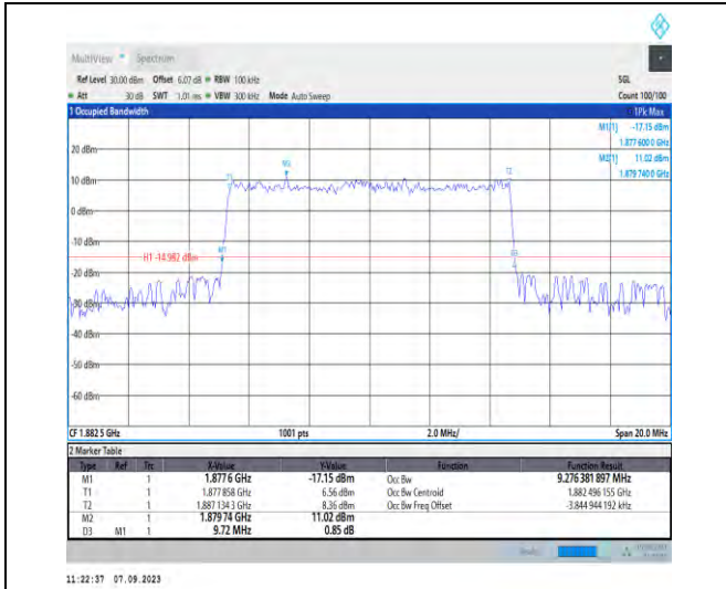
1-N25-PC3-15-10-M-8-CP-64QAM-Outer_Full-52@0 -Ant2-9.276-9.720-≤10-PASS
