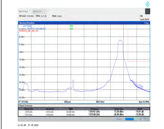
1-N25-PC3-15-5-H-5-CP-QPSK-Edge_1RB_Right-1@24-Ant2-1-seegraph-PASS-see graph
