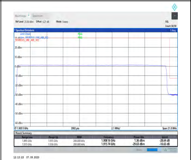
1-N25-PC3-15-20-H-6-CP-QPSK-Outer_Full-106@0-Ant2-1-seegraph-PASS-see graph
