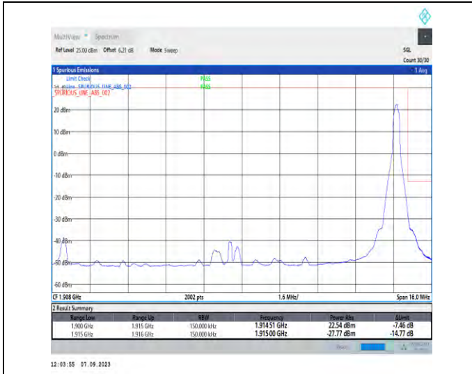
1-N25-PC3-15-15-H-2-DFT-PI2BPSK-Edge_1RB_Right-t1@78-Ant2-1-seegraph-PASS-see graph
