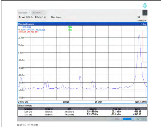
1-N25-PC3-15-25-H-2-DFT-PI2BPSK-Edge_1RB_Right-t-1@132-Ant2-1-seegraph-PASS-see graph
