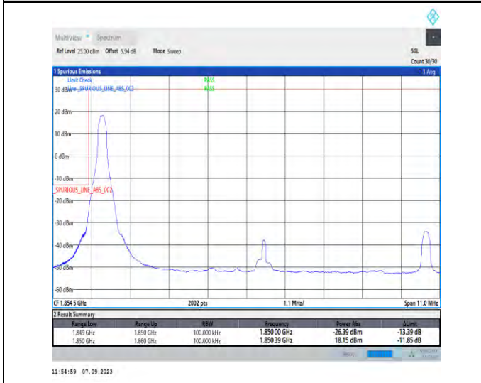
1-N25-PC3-15-10-L-4-CP-QPSK-Edge_1RB_Left-1@0-Ant2-1-seegraph-PASS-see graph
