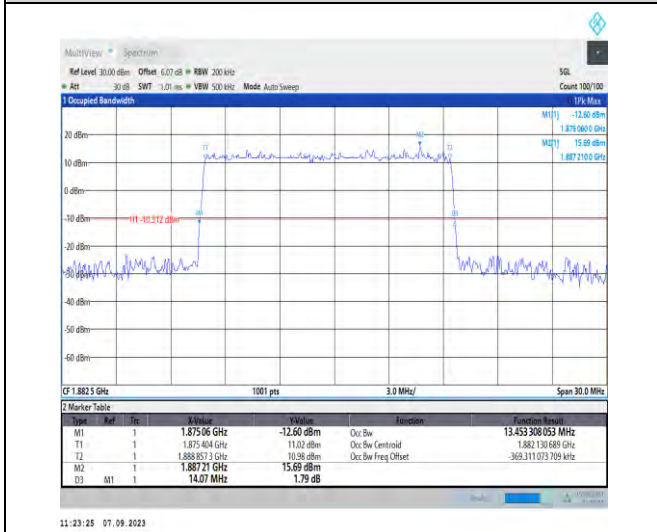
1-N25-PC3-15-15-M-1-DFT-QPSK-Outer_Full-75@0 -Ant2-13.453-14.070-≤15-PASS
