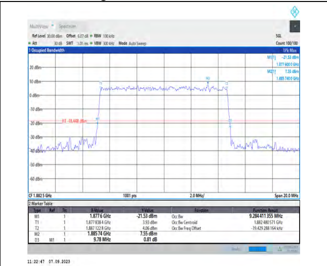
1-N25-PC3-15-10-M-9-CP-256QAM-Outer_Full-52@0 -Ant2-9.284-9.780-≤10-PASS
