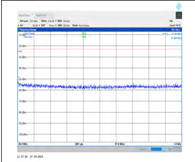
1-N25-PC3-15-40-H-1-DFT-PI2BPSK-Inner_1RB_L eft-1@1-30-1000-Ant2-31.46--51.56--23-PASS
