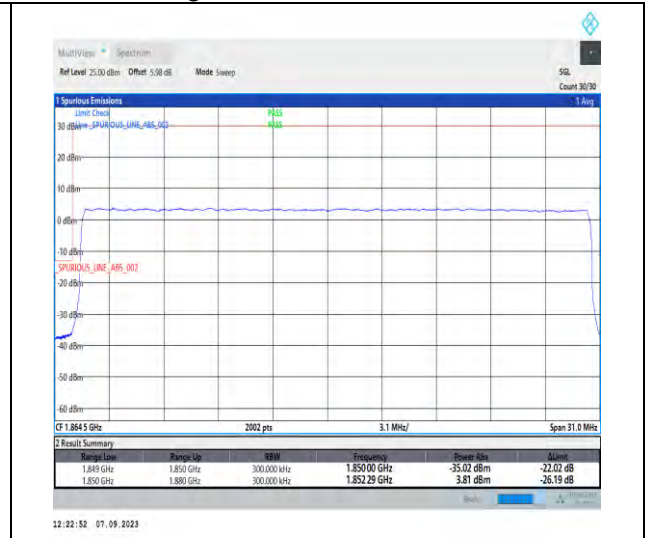
1-N25-PC3-15-30-L-3-DFT-PI2BPSK-Outer_Full-160@0-Ant2-1-seegraph-PASS-see graph
