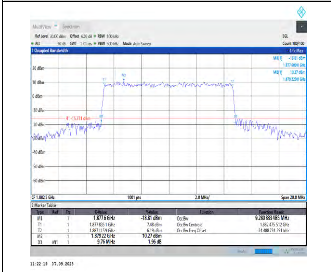
1-N25-PC3-15-10-M-6-CP-QPSK-Outer_Full-52@0- Ant2-9.281-9.760-≤10-PASS
