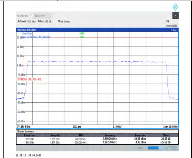
1-N25-PC3-15-20-L-3-DFT-PI2BPSK-Outer_Full-100@0-Ant2-1-seegraph-PASS-see graph
