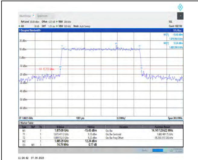
1-N25-PC3-15-15-M-7-CP-16QAM-Outer_Full-79@0 -Ant2-14.141-14.790-≤15-PASS
