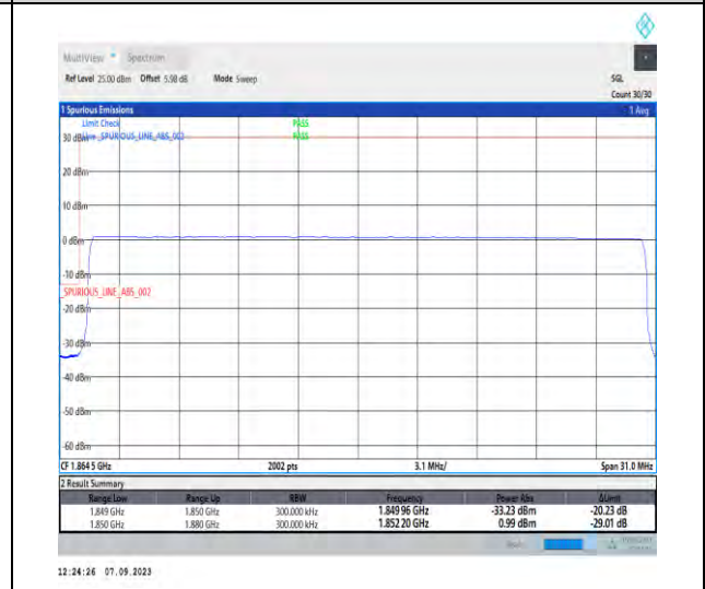
1-N25-PC3-15-30-L-6-CP-QPSK-Outer_Full-160@0-Ant2-1-seegraph-PASS-see graph
