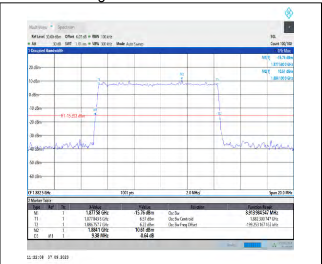
1-N25-PC3-15-10-M-5-DFT-256QAM-Outer_Full-50 @0-Ant2-8.914-9.380-≤10-PASS
