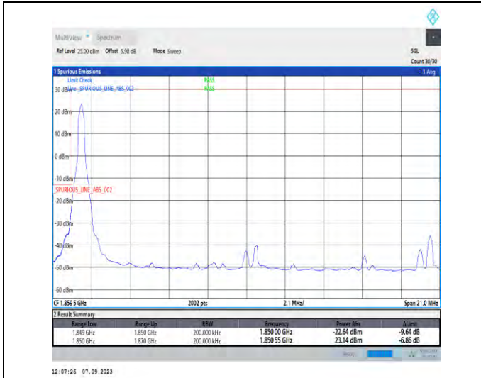
1-N25-PC3-15-20-L-1-DFT-PI2BPSK-Edge_1RB_Left-1@0-Ant2-1-seegraph-PASS-see graph
