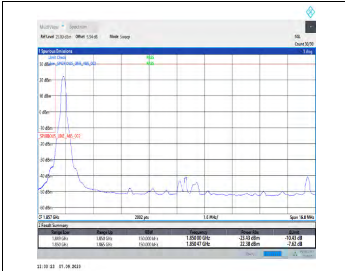
1-N25-PC3-15-15-L-1-DFT-PI2BPSK-Edge_1RB_Left-1@0-Ant2-1-seegraph-PASS-see graph
