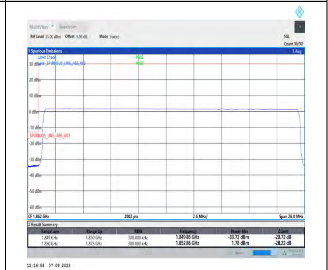
1-N25-PC3-15-25-L-6-CP-QPSK-Outer_Full-133@0-Ant2-1-seegraph-PASS-see graph
