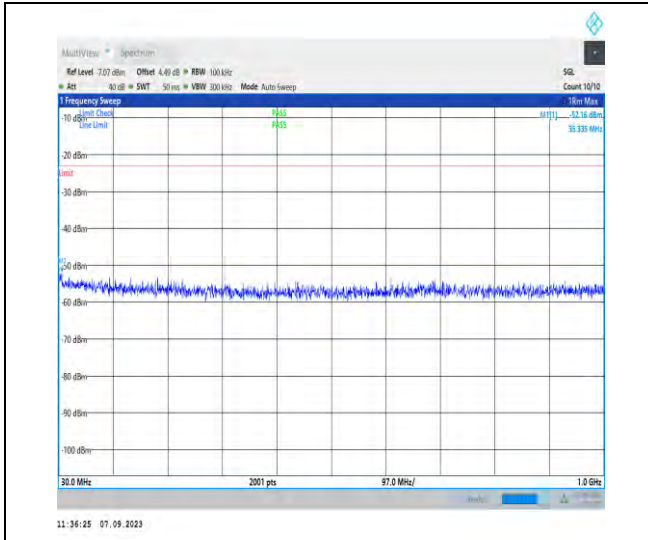
1-N25-PC3-15-40-M-1-DFT-PI2BPSK-Inner_1RB_L eft-1@1-30-1000-Ant2-35.34--52.16--23-PASS
