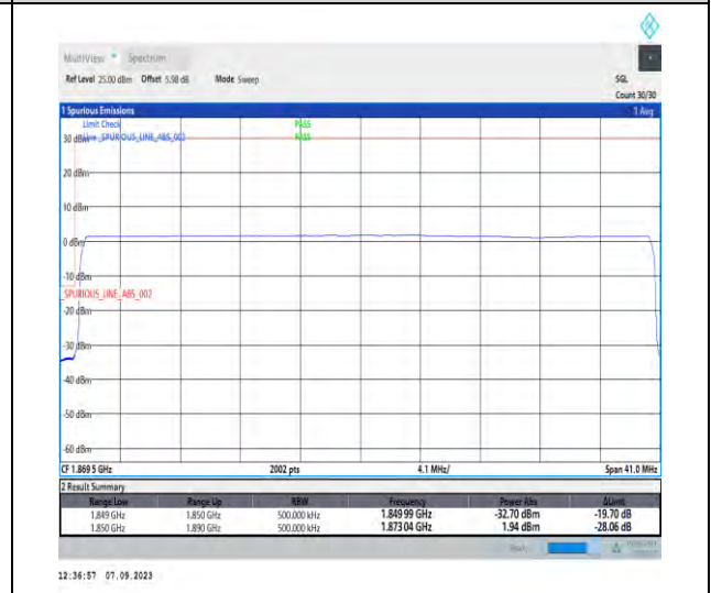
1-N25-PC3-15-40-L-6-CP-QPSK-Outer_Full-216@0-Ant2-1-seegraph-PASS-see graph
