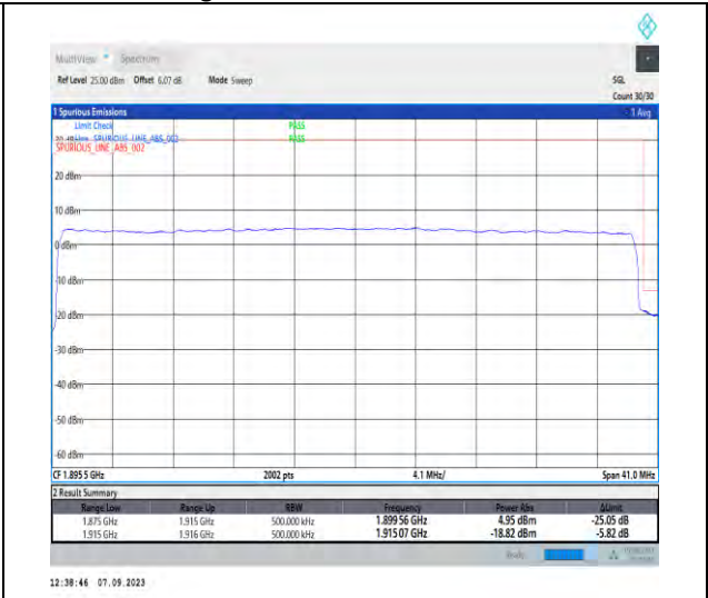
1-N25-PC3-15-40-H-3-DFT-PI2BPSK-Outer_Full-216@0-Ant2-1-seegraph-PASS-see graph
