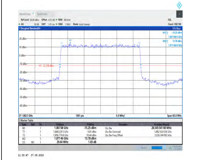
1-N25-PC3-15-30-M-2-DFT-PI2BPSK-Outer_Full-160 @0-Ant2-28.546-29.640-≤30-PASS
