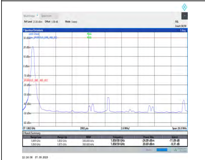
1-N25-PC3-15-25-L-4-CP-QPSK-Edge_1RB_Left-1@0-Ant2-1-seegraph-PASS-see graph
