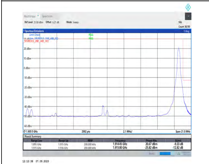
1-N25-PC3-15-20-H-5-CP-QPSK-Edge_1RB_Right-1@105-Ant2-1-seegraph-PASS-see graph
