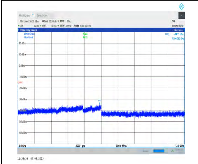
1-N25-PC3-15-40-M-1-DFT-PI2BPSK-Inner_1RB_L eft-1@1-3000-12000-Ant2-7396.05--34.71--13-PAS S
