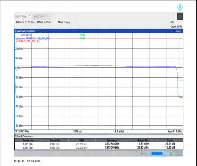
1-N25-PC3-15-40-H-6-CP-QPSK-Outer_Full-216@0-Ant2-1-seegraph-PASS-see graph
