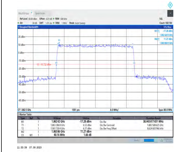
1-N25-PC3-15-40-M-5-DFT-256QAM-Outer_Full-216 @0-Ant2-38.444-40.160-≤40-PASS
