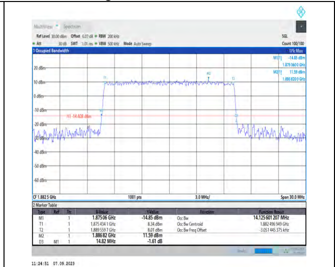
1-N25-PC3-15-15-M-8-CP-64QAM-Outer_Full-79@0 -Ant2-14.126-14.820-≤15-PASS
