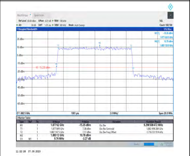
1-N25-PC3-15-10-M-7-CP-16QAM-Outer_Full-52@0- -Ant2-9.299-9.740-≤10-PASS
