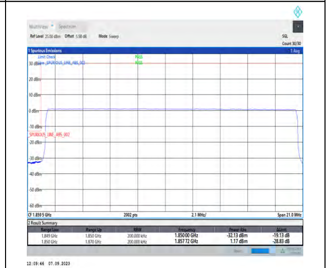
1-N25-PC3-15-20-L-6-CP-QPSK-Outer_Full-106@0-Ant2-1-seegraph-PASS-see graph
