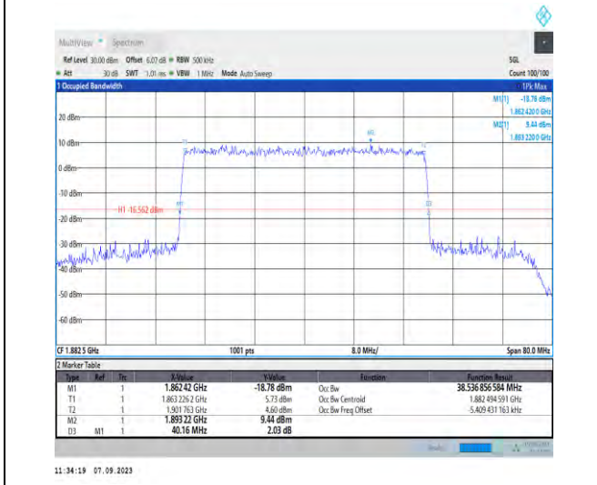
1-N25-PC3-15-40-M-9-CP-256QAM-Outer_Full-216 @0-Ant2-38.537-40.160-≤40-PASS
