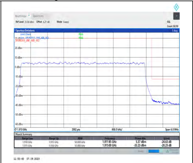
1-N25-PC3-15-5-H-3-DFT-PI2BPSK-Outer_Full-25@0-Ant2-1-seegraph-PASS-see graph
