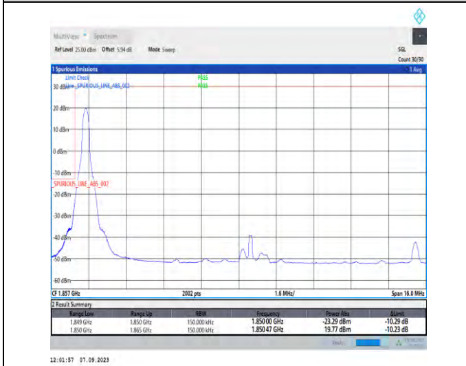
1-N25-PC3-15-15-L-4-CP-QPSK-Edge_1RB_Left-1@0-Ant2-1-seegraph-PASS-see graph
