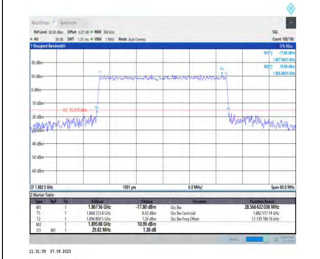
1-N25-PC3-15-30-M-6-CP-QPSK-Outer_Full-160@0 -Ant2-28.567-29.820-≤30-PASS
