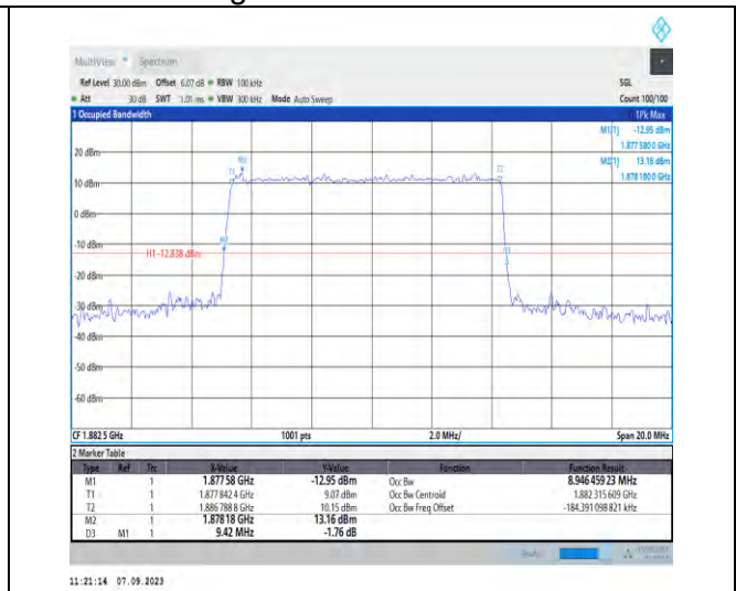
1-N25-PC3-15-10-M-1-DFT-QPSK-Outer_Full-50@0 -Ant2-8.946-9.420-≤10-PASS
