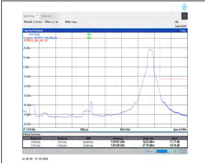
1-N25-PC3-15-5-H-2-DFT-PI2BPSK-Edge_1RB_Right-1@24-Ant2-1-seegraph-PASS-see graph
