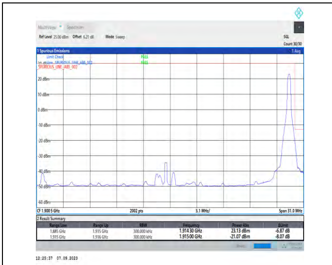
1-N25-PC3-15-30-H-2-DFT-PI2BPSK-Edge_1RB_Right-t-1@159-Ant2-1-seegraph-PASS-see graph
