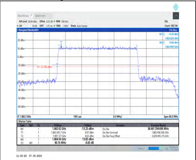
1-N25-PC3-15-40-M-4-DFT-64QAM-Outer_Full-216 @0-Ant2-38.461-40.160-≤40-PASS
