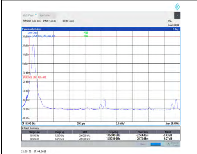
1-N25-PC3-15-20-L-4-CP-QPSK-Edge_1RB_Left-1@0-Ant2-1-seegraph-PASS-see graph
