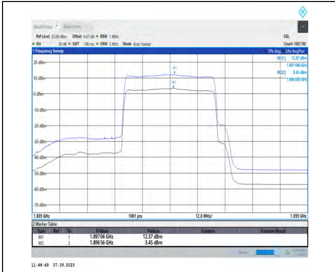
1-N25-PC3-15-40-H-1-DFT-256QAM-Outer_Full-216 @0-Ant2-8.92-100%-0.00-8.92-PASS-≤13
