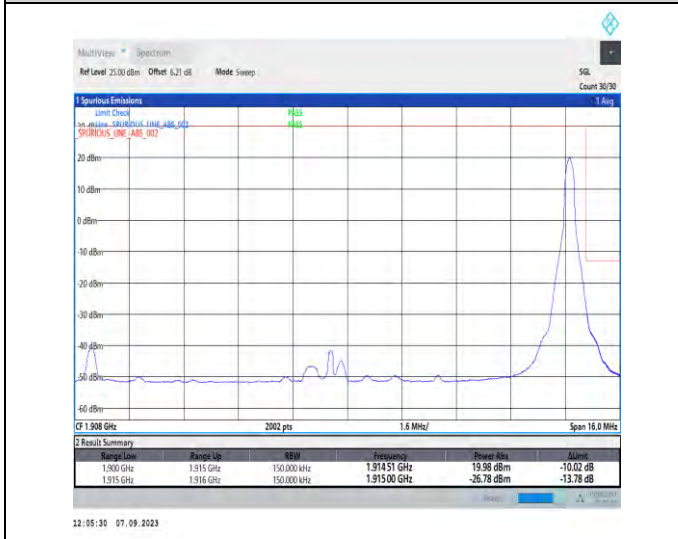
1-N25-PC3-15-15-H-5-CP-QPSK-Edge_1RB_Right-1@78-Ant2-1-seegraph-PASS-see graph
