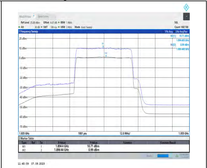
1-N25-PC3-15-40-H-2-CP-256QAM-Outer_Full-216 @0-Ant2-9.72-100%-0.00-9.72-PASS-≤13
