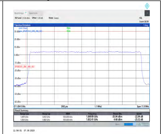
1-N25-PC3-15-10-L-3-DFT-PI2BPSK-Outer_Full-50@0-Ant2-1-seegraph-PASS-see graph
