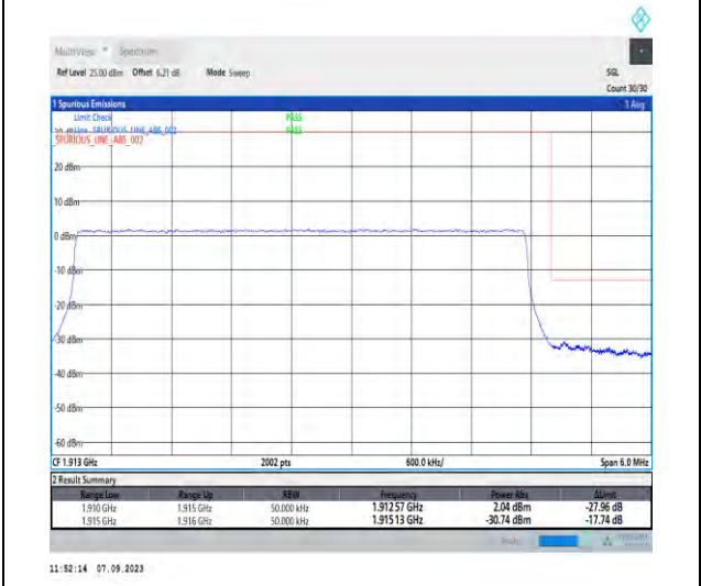
1-N25-PC3-15-5-H-6-CP-QPSK-Outer_Full-25@0-Ant2-1-seegraph-PASS-see graph
