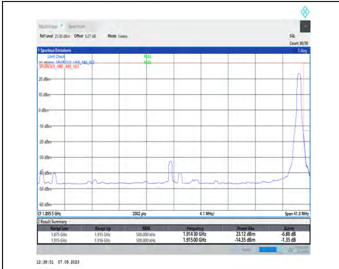
1-N25-PC3-15-40-H-2-DFT-PI2BPSK-Edge_1RB_Right-t-1@215-Ant2-1-seegraph-PASS-see graph
