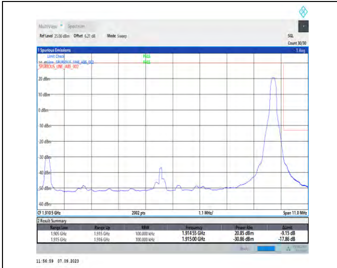
1-N25-PC3-15-10-H-2-DFT-PI2BPSK-Edge_1RB_Right-t@51-Ant2-1-seegraph-PASS-see graph
