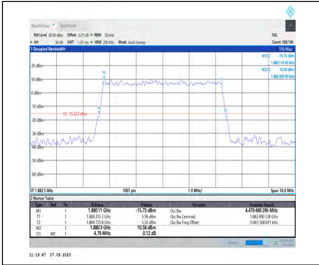
1-N25-PC3-15-5-M-5-DFT-256QAM-Outer_Full-25@0-Ant2-4.47-4.790-≤5-PASS
