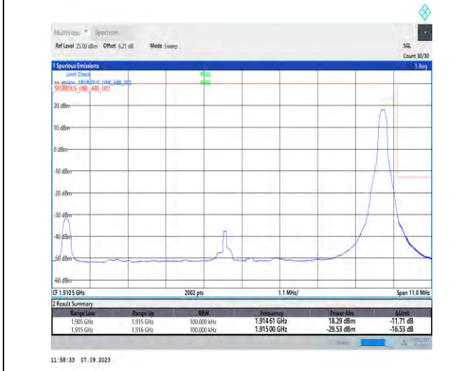
1-N25-PC3-15-10-H-5-CP-QPSK-Edge_1RB_Right-1@51-Ant2-1-seegraph-PASS-see graph
