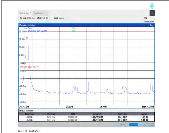
1-N25-PC3-15-25-L-1-DFT-PI2BPSK-Edge_1RB_Left-1@0-Ant2-1-seegraph-PASS-see graph
