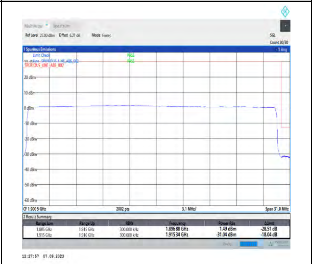
1-N25-PC3-15-30-H-6-CP-QPSK-Outer_Full-160@0-Ant2-1-seegraph-PASS-see graph
