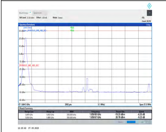
1-N25-PC3-15-30-L-4-CP-QPSK-Edge_1RB_Left-1@0-Ant2-1-seegraph-PASS-see graph
