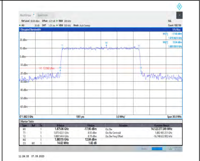
1-N25-PC3-15-15-M-6-CP-QPSK-Outer_Full-79@0- Ant2-14.122-14.820-≤15-PASS
