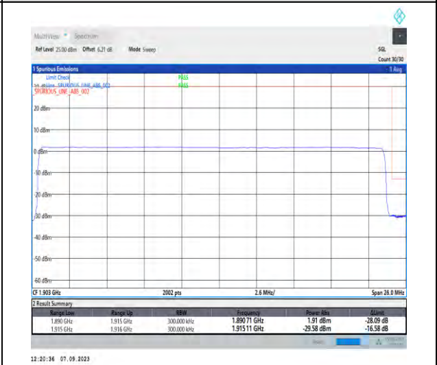
1-N25-PC3-15-25-H-6-CP-QPSK-Outer_Full-133@0-Ant2-1-seegraph-PASS-see graph
