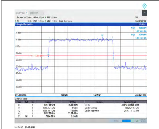
1-N25-PC3-15-30-M-4-DFT-64QAM-Outer_Full-160 @0-Ant2-28.544-29.640-≤30-PASS
