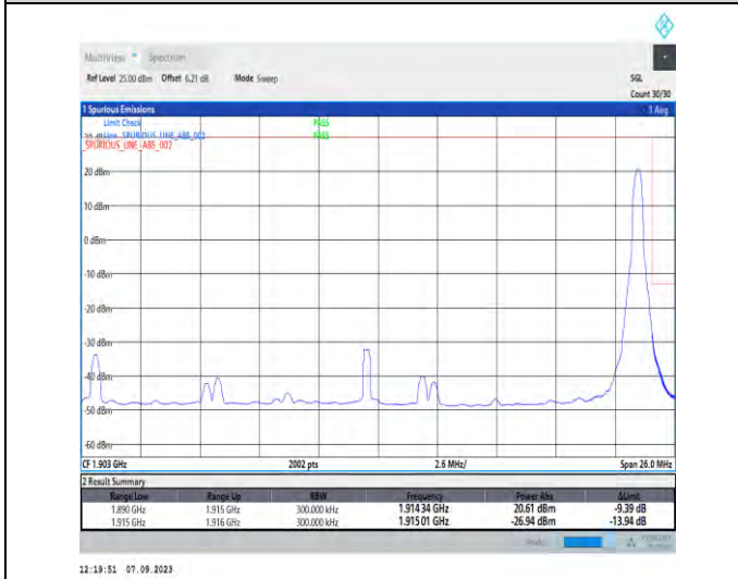
1-N25-PC3-15-25-H-5-CP-QPSK-Edge_1RB_Right-1@132-Ant2-1-seegraph-PASS-see graph
