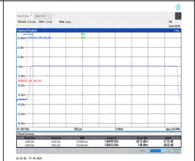
1-N25-PC3-15-15-L-6-CP-QPSK-Outer_Full-79@0-Ant2-1-seegraph-PASS-see graph
