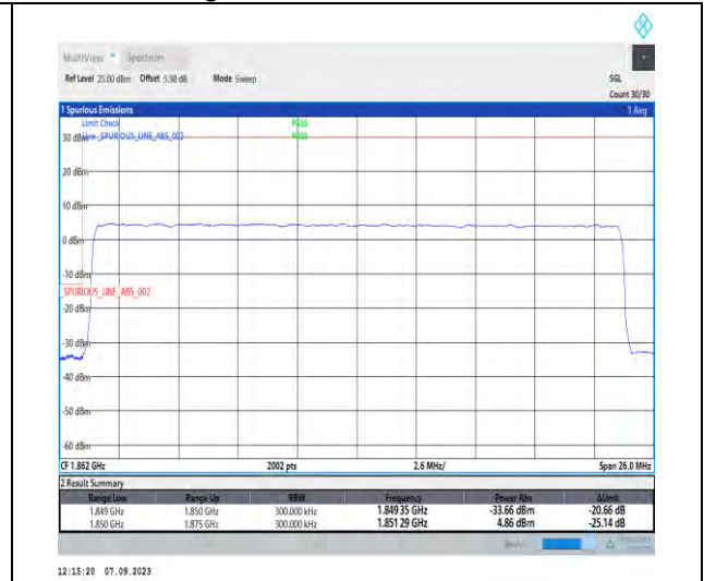
1-N25-PC3-15-25-L-3-DFT-PI2BPSK-Outer_Full-128@0-Ant2-1-seegraph-PASS-see graph
