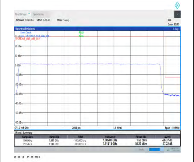
1-N25-PC3-15-10-H-6-CP-QPSK-Outer_Full-52@0-Ant2-1-seegraph-PASS-see graph
