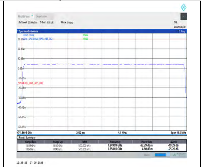
1-N25-PC3-15-40-L-3-DFT-PI2BPSK-Outer_Full-216@0-Ant2-1-seegraph-PASS-see graph
