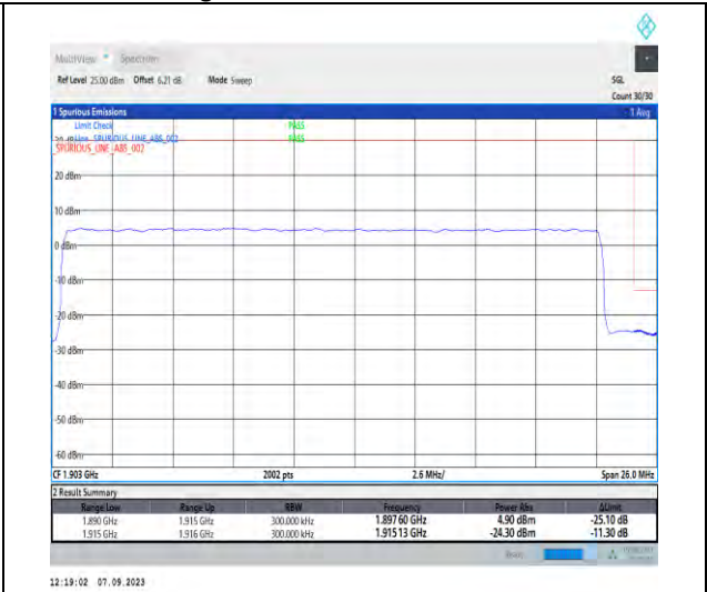
1-N25-PC3-15-25-H-3-DFT-PI2BPSK-Outer_Full-1-28@0-Ant2-1-seegraph-PASS-see graph
