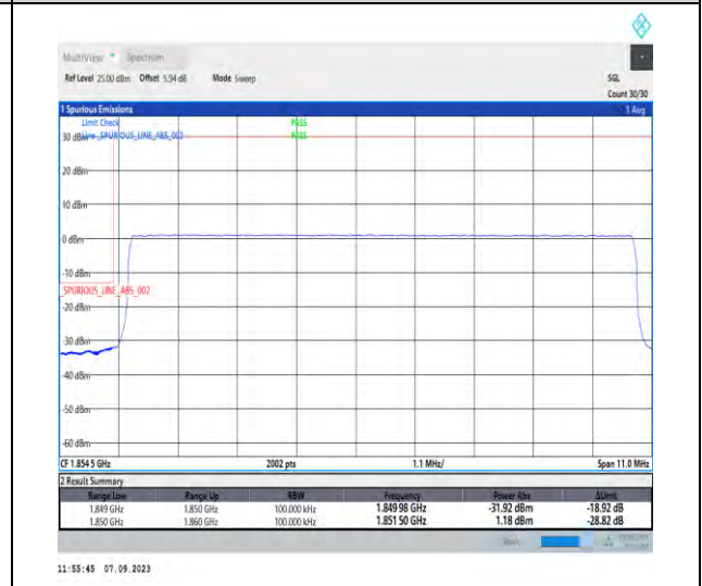
1-N25-PC3-15-10-L-6-CP-QPSK-Outer_Full-52@0-Ant2-1-seegraph-PASS-see graph
