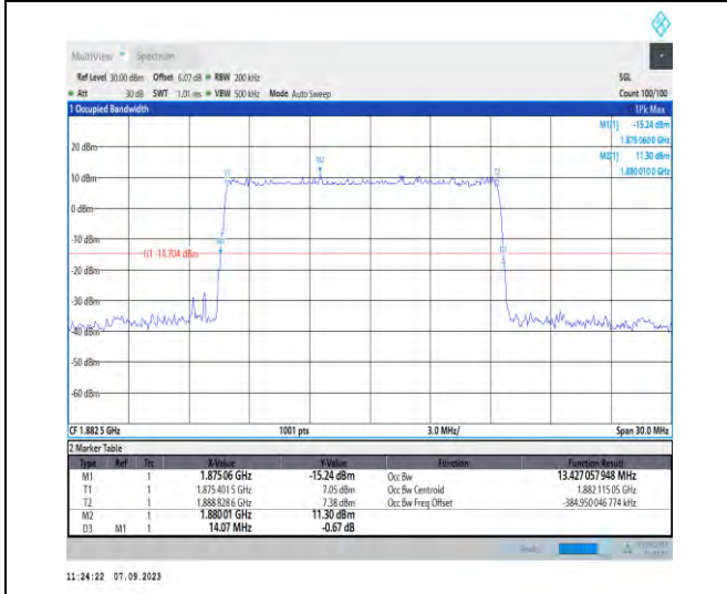
1-N25-PC3-15-15-M-5-DFT-256QAM-Outer_Full-75 @0-Ant2-13.427-14.070-≤15-PASS
