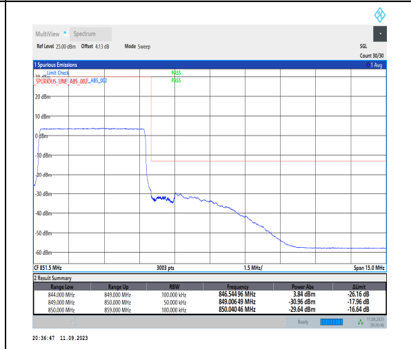
1-N5-PC3-15-5-H-6-CP-QPSK-Outer_Full-25@0-Ant1-1--PASS-see graph
