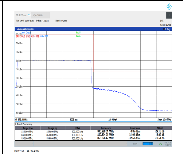
1-N5-PC3-15-10-H-6-CP-QPSK-Outer_Full-52@0-Ant1-1--PASS-see graph
