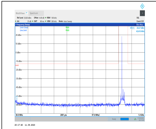
1-N5-PC3-15-20-H-1-DFT-PI2BPSK-Inner_1RB_Left -1@1-30-1000-Ant1-42.61--54.27--13-PASS
