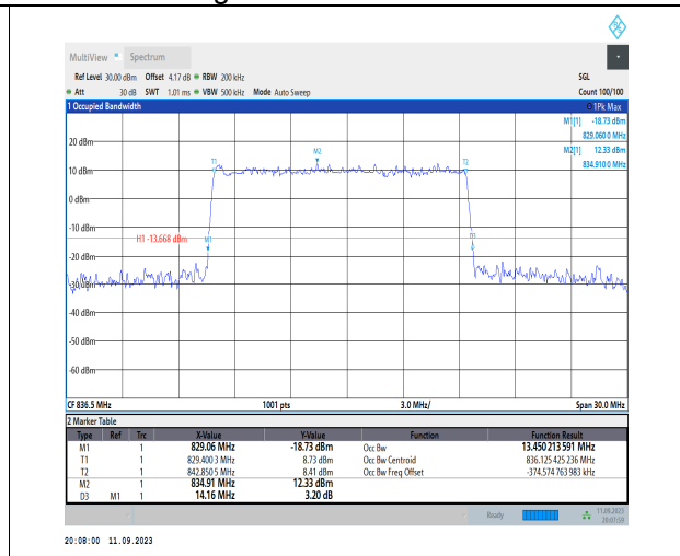
1-N5-PC3-15-15-M-4-DFT-64QAM-Outer_Full-75@0 -Ant1-13.45-14.160-≤15-PASS
