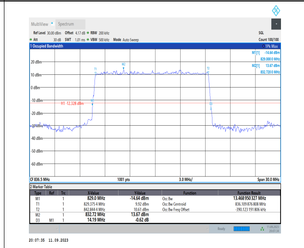
1-N5-PC3-15-15-M-2-DFT-PI2BPSK-Outer_Full-75@0-Ant1-13.469-14.190-≤15-PASS
