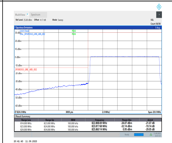
1-N5-PC3-15-10-L-6-CP-QPSK-Outer_Full-52@0- Ant1-1--PASS-see graph
