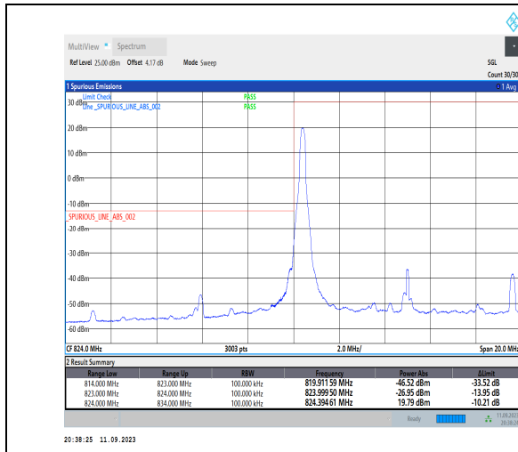
1-N5-PC3-15-10-L-1-DFT-PI2BPSK-Edge_1RB_Left-1 @0-Ant1-1--PASS-see graph
