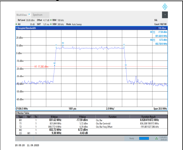
1-N5-PC3-15-10-M-5-DFT-256QAM-Outer_Full-50@0-Ant1-8.928-9.380-≤10-PASS
