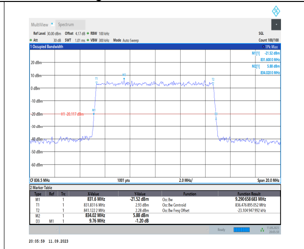
1-N5-PC3-15-10-M-9-CP-256QAM-Outer_Full-52@0-Ant1-9.291-9.760-≤10-PASS
