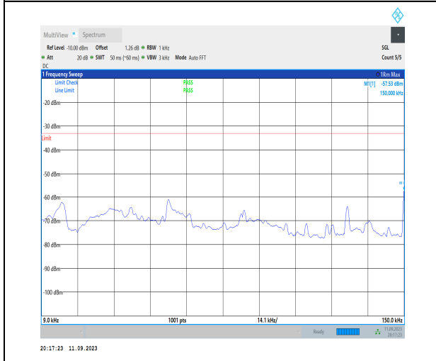
1-N5-PC3-15-20-H-1-DFT-PI2BPSK-Inner_1RB_Left -1@1-0.009-0.15-Ant1-0.15--57.53--33-PASS
