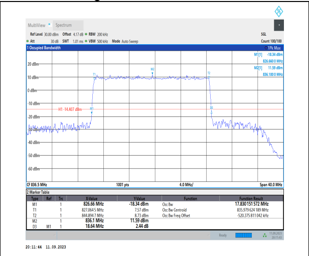
1-N5-PC3-15-20-M-3-DFT-16QAM-Outer_Full-100 @0-Ant1-17.83-18.640-≤20-PASS
