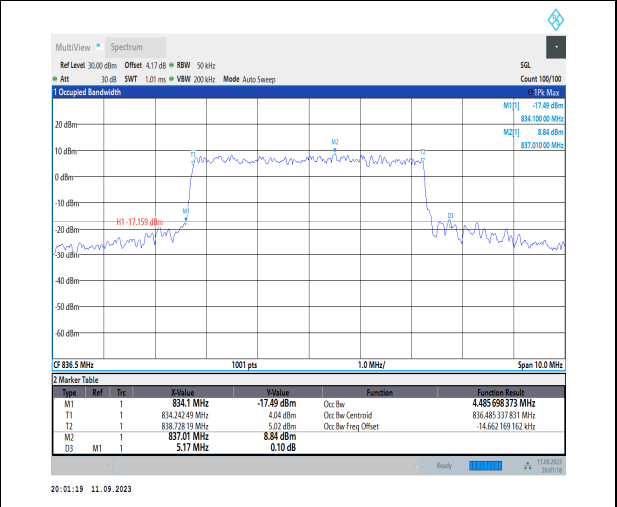
1-N5-PC3-15-5-M-8-CP-64QAM-Outer_Full-25@0-A nt1-4.486-5.170- \leq 5 -PASS
