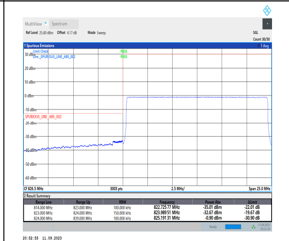
1-N5-PC3-15-15-L-6-CP-QPSK-Outer_Full-79@0- Ant1-1--PASS-see graph
