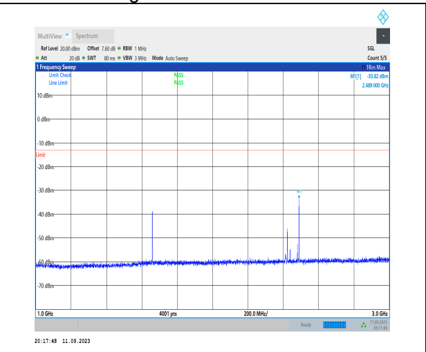
1-N5-PC3-15-20-H-1-DFT-PI2BPSK-Inner_1RB_Left -1@1-1000-3000-Ant1-2489.00--33.82--13-PASS
