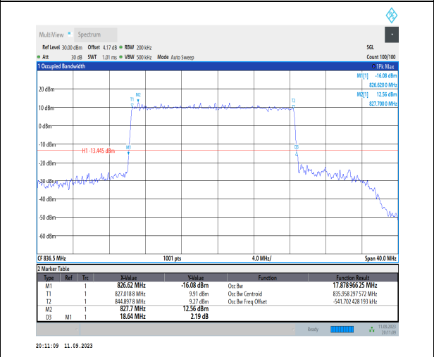
1-N5-PC3-15-20-M-1-DFT-QPSK-Outer_Full-100@0-Ant1-17.879-18.640-<math>\leq 20</math>-PASS
