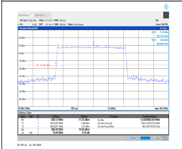
1-N5-PC3-15-15-M-5-DFT-256QAM-Outer_Full-75@0 -Ant1-13.43-14.040-≤15-PASS
