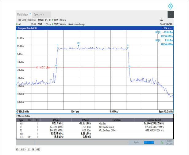
1-N5-PC3-15-20-M-5-DFT-256QAM-Outer_Full-100 @0-Ant1-17.844-18.600-≤20-PASS
