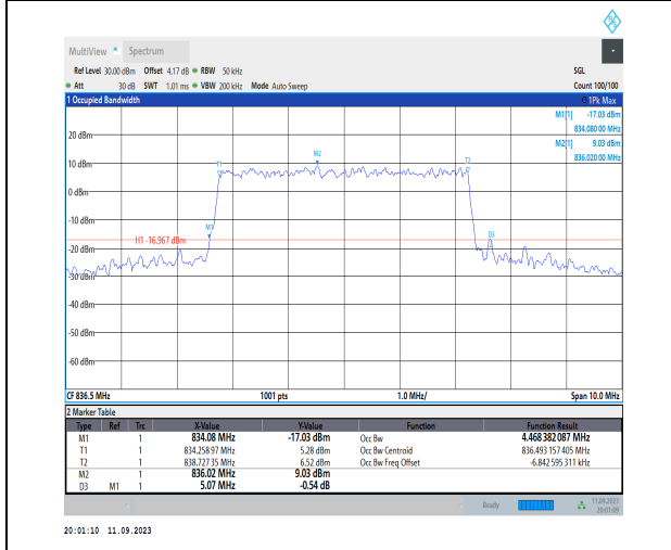
1-N5-PC3-15-5-M-7-CP-16QAM-Outer_Full-25@0-A nt1-4.468-5.070- \leq 5 -PASS
