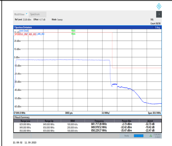
1-N5-PC3-15-20-H-6-CP-QPSK-Outer_Full-106@0-Ant1-1--PASS-see graph
