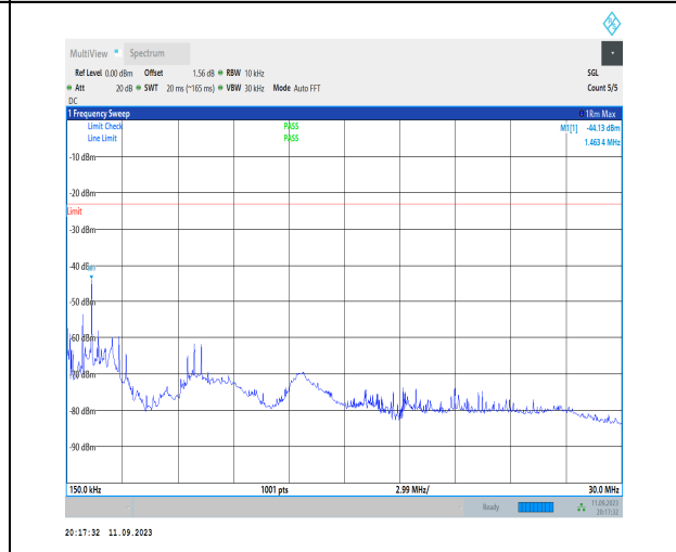
1-N5-PC3-15-20-H-1-DFT-PI2BPSK-Inner_1RB_Left -1@1-0.15-30-Ant1-1.46--44.13--23-PASS
