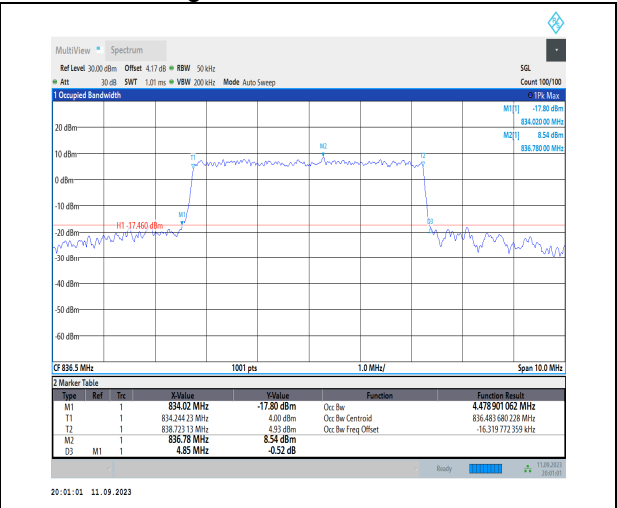
1-N5-PC3-15-5-M-6-CP-QPSK-Outer_Full-25@0-An t1-4.479-4.850- \leq 5 -PASS
