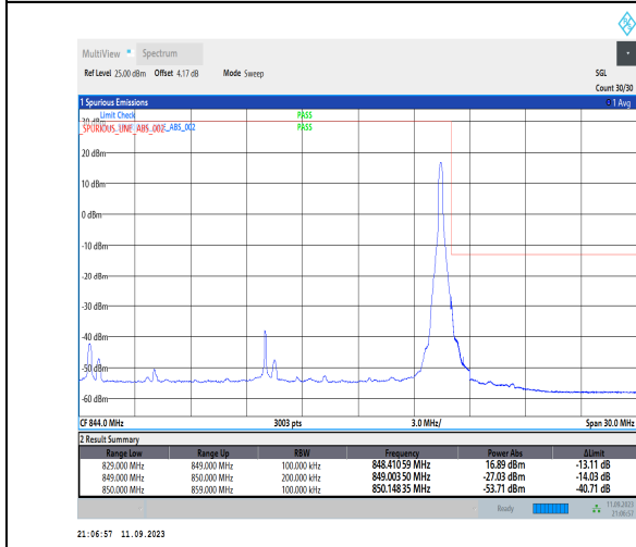
1-N5-PC3-15-20-H-5-CP-QPSK-Edge_1RB_Right-1@105-Ant1-1--PASS-see graph
