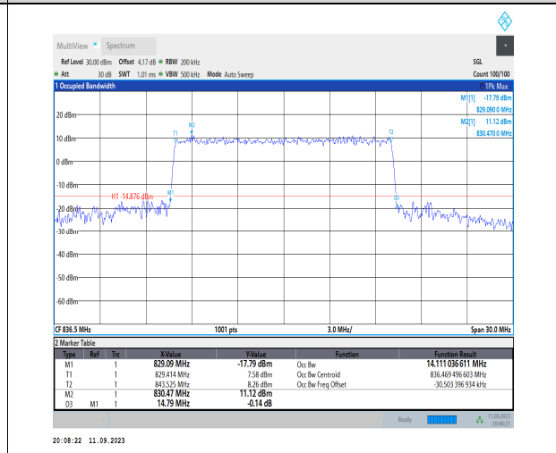
1-N5-PC3-15-15-M-6-CP-QPSK-Outer_Full-79@0-A nt1-14.111-14.790-≤15-PASS
