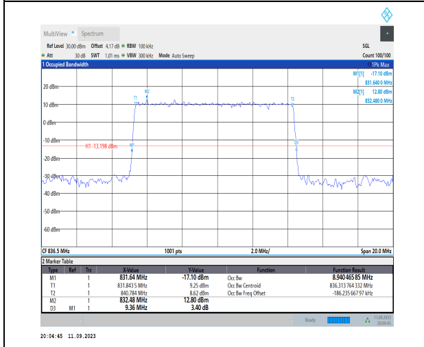
1-N5-PC3-15-10-M-2-DFT-PI2BPSK-Outer_Full-50@0-Ant1-8.94-9.360-≤10-PASS
