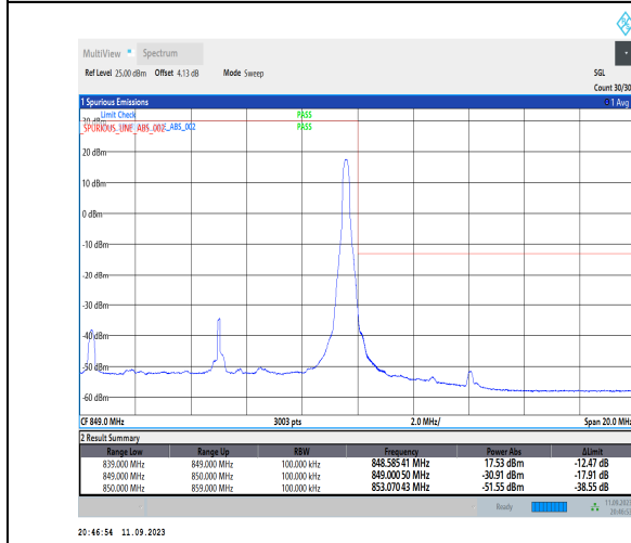
1-N5-PC3-15-10-H-5-CP-QPSK-Edge_1RB_Right-1@51-Ant1-1--PASS-see graph
