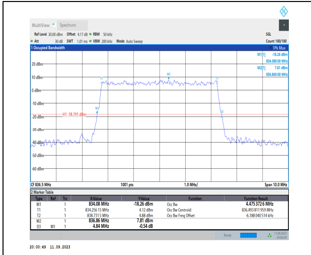
1-N5-PC3-15-5-M-5-DFT-256QAM-Outer_Full-25@0 -Ant1-4.475-4.840- \leq 5 -PASS
