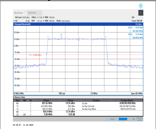
1-N5-PC3-15-10-M-1-DFT-QPSK-Outer_Full-50@0-Ant1-8.904-9.360-≤10-PASS
