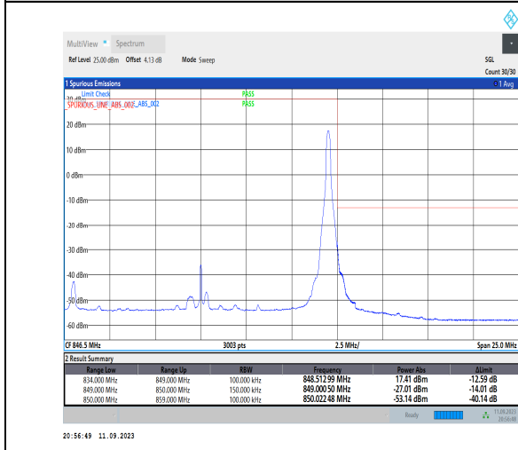
1-N5-PC3-15-15-H-5-CP-QPSK-Edge_1RB_Right-1@78-Ant1-1--PASS-see graph
