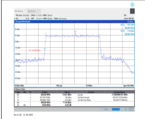
1-N5-PC3-15-20-M-4-DFT-64QAM-Outer_Full-100 @0-Ant1-17.859-18.640-≤20-PASS
