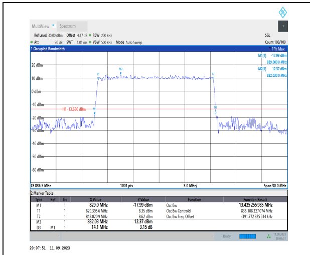
1-N5-PC3-15-15-M-3-DFT-16QAM-Outer_Full-75@0 -Ant1-13.425-14.100-≤15-PASS
