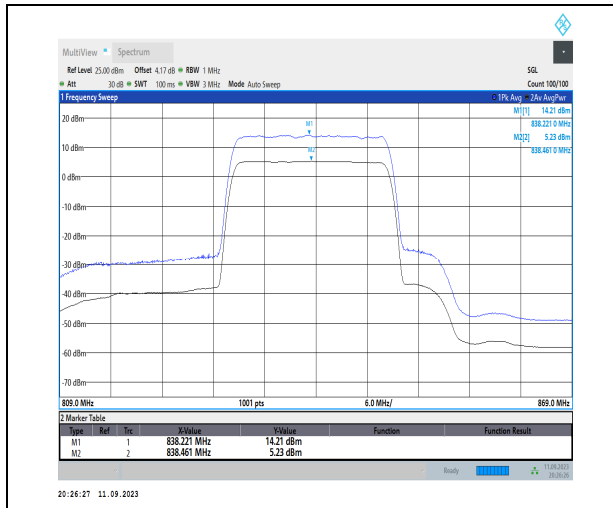
1-N5-PC3-15-20-H-1-DFT-256QAM-Outer_Full-100 @0-Ant1-8.98-100%-0.00-8.98-PASS-≤13
