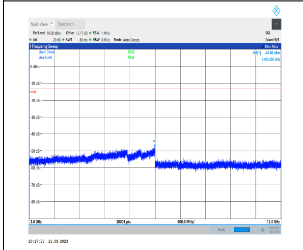
1-N5-PC3-15-20-H-1-DFT-PI2BPSK-Inner_1RB_Left -1@1-3000-12000-Ant1-7475.25--47.88--13-PASS
