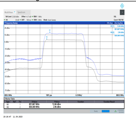
1-N5-PC3-15-20-H-2-CP-256QAM-Outer_Full-106@ 0-Ant1-9.88-100%-0.00-9.88-PASS-≤13
