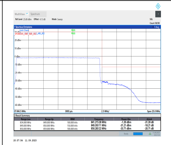
1-N5-PC3-15-15-H-6-CP-QPSK-Outer_Full-79@0-Ant1-1--PASS-see graph
