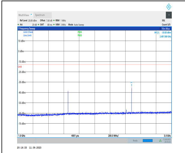
1-N5-PC3-15-20-M-1-DFT-PI2BPSK-Inner_1RB_Left -1@1-1000-3000-Ant1-2481.50--33.83--13-PASS
