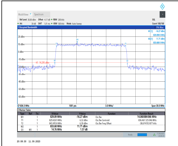
1-N5-PC3-15-15-M-7-CP-16QAM-Outer_Full-79@0-Ant1-14.069-14.760-<math>\leq 15</math>-PASS
