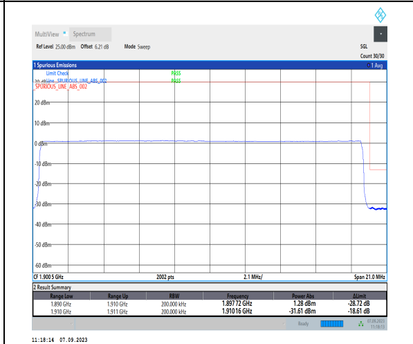
1-N2-PC3-15-20-H-6-CP-QPSK-Outer_Full-106@0-Ant2-1-seegraph-PASS-see graph
