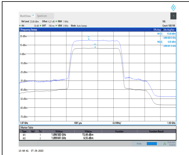
1-N2-PC3-15-20-H-1-DFT-256QAM-Outer_Full-100 @0-Ant2-8.89-100%-0.00-8.89-PASS-≤13
