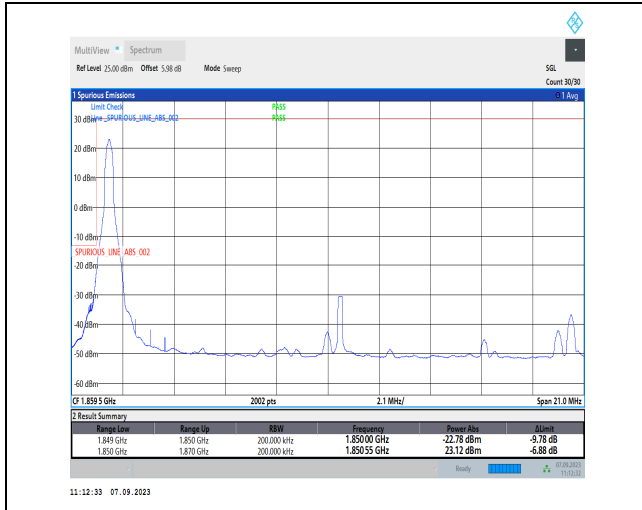
1-N2-PC3-15-20-L-1-DFT-PI2BPSK-Edge_1RB_Left-1@0-Ant2-1-seegraph-PASS-see graph
