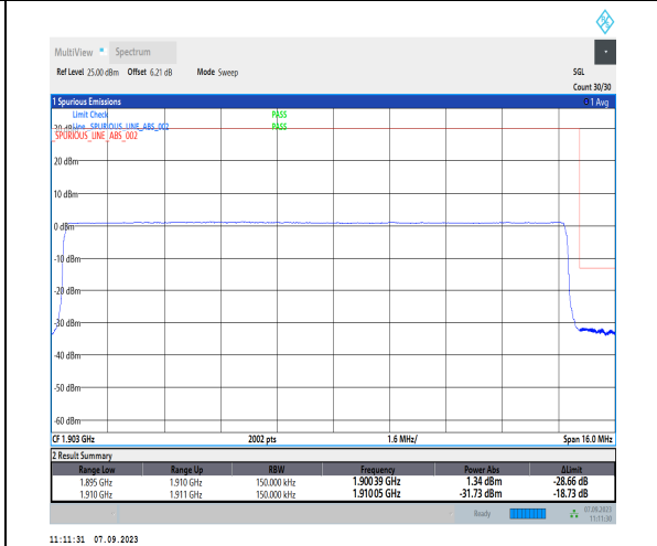
1-N2-PC3-15-15-H-6-CP-QPSK-Outer_Full-79@0-Ant2-1-seegraph-PASS-see graph
