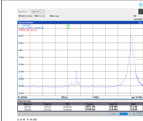
1-N2-PC3-15-15-H-5-CP-QPSK-Edge_1RB_Right-1@78-Ant2-1-seegraph-PASS-see graph
