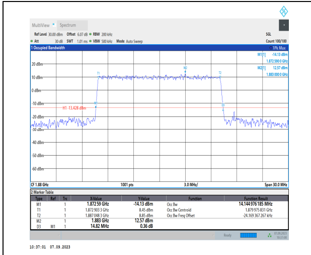
1-N2-PC3-15-15-M-7-CP-16QAM-Outer_Full-79@0-Ant2-14.145-14.820-<=15-PASS
