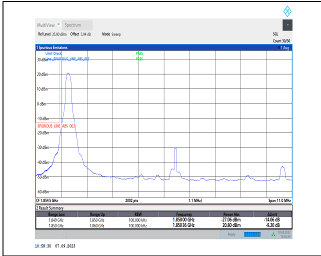
1-N2-PC3-15-10-L-1-DFT-PI2BPSK-Edge_1RB_Left-1 @0-Ant2-1-seegraph-PASS-see graph
