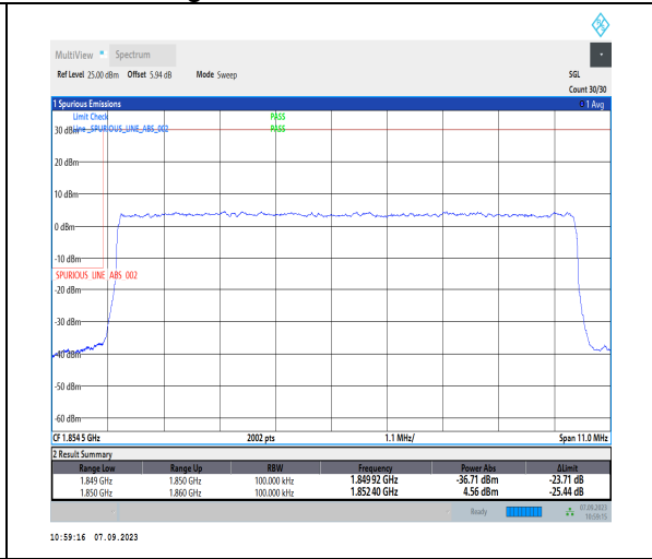
1-N2-PC3-15-10-L-3-DFT-PI2BPSK-Outer_Full-50 @0-Ant2-1-seegraph-PASS-see graph
