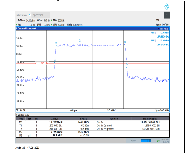
1-N2-PC3-15-15-M-4-DFT-64QAM-Outer_Full-75@0 -Ant2-13.429-14.100-≤15-PASS
