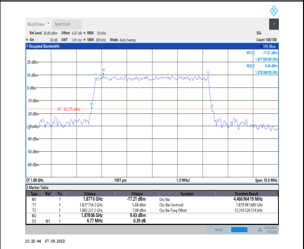
1-N2-PC3-15-5-M-8-CP-64QAM-Outer_Full-25@0-A nt2-4.467-4.770- \leq 5 -PASS
