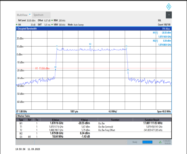
1-N2-PC3-15-20-M-1-DFT-QPSK-Outer_Full-100@0-Ant2-17.881-18.640-<=20-PASS
