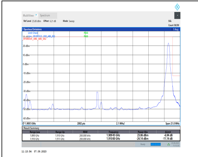
1-N2-PC3-15-20-H-2-DFT-PI2BPSK-Edge_1RB_Right-1@105-Ant2-1-seegraph-PASS-see graph
