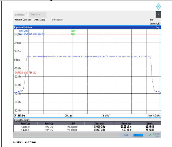
1-N2-PC3-15-15-L-3-DFT-PI2BPSK-Outer_Full-75 @0-Ant2-1-seegraph-PASS-see graph
