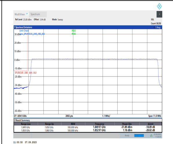
1-N2-PC3-15-10-L-6-CP-QPSK-Outer_Full-52 @0-Ant2-1-seegraph-PASS-see graph
