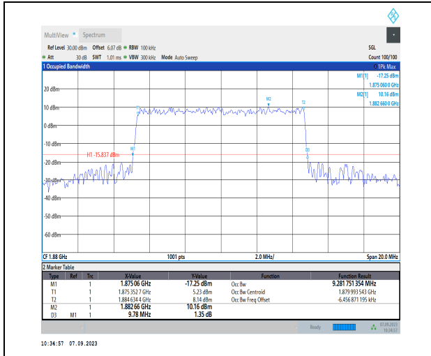
1-N2-PC3-15-10-M-8-CP-64QAM-Outer_Full-52@0-Ant2-9.282-9.780-<math>\leq 10</math>-PASS
