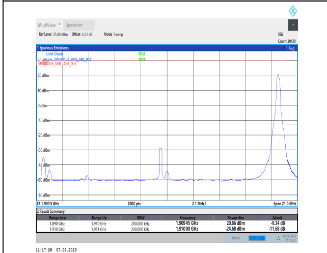
1-N2-PC3-15-20-H-5-CP-QPSK-Edge_1RB_Right-1@105-Ant2-1-seegraph-PASS-see graph
