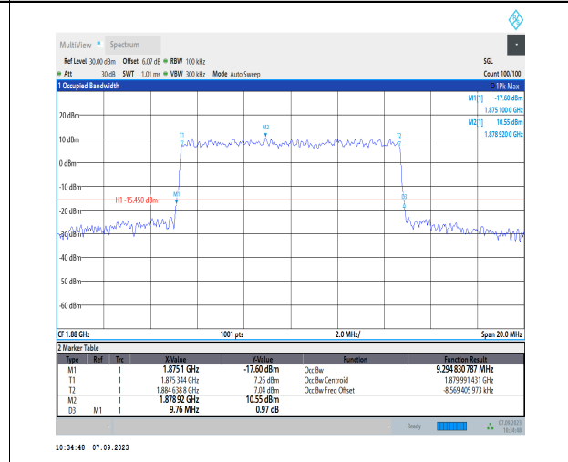
1-N2-PC3-15-10-M-7-CP-16QAM-Outer_Full-52@0-Ant2-9.295-9.760-≤10-PASS
