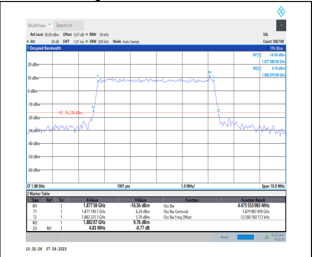
1-N2-PC3-15-5-M-6-CP-QPSK-Outer_Full-25@0-An t2-4.476-4.830- \leq 5 -PASS
