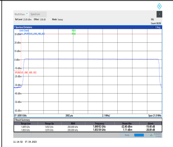
1-N2-PC3-15-20-L-6-CP-QPSK-Outer_Full-106@0-Ant2-1-seegraph-PASS-see graph
