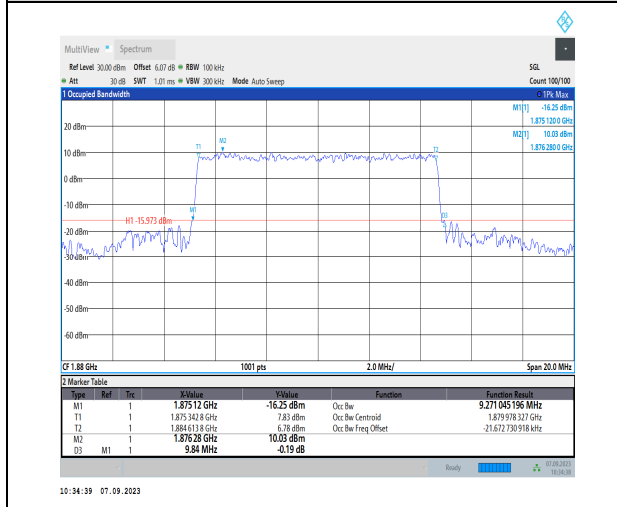
1-N2-PC3-15-10-M-6-CP-QPSK-Outer_Full-52@0-Ant2-9.271-9.840-≤10-PASS
