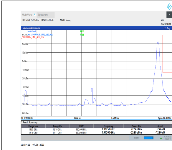
1-N2-PC3-15-15-H-2-DFT-PI2BPSK-Edge_1RB_Right-1@78-Ant2-1-seegraph-PASS-see graph
