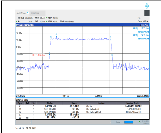
1-N2-PC3-15-15-M-3-DFT-16QAM-Outer_Full-75@0 -Ant2-13.417-14.130-≤15-PASS
