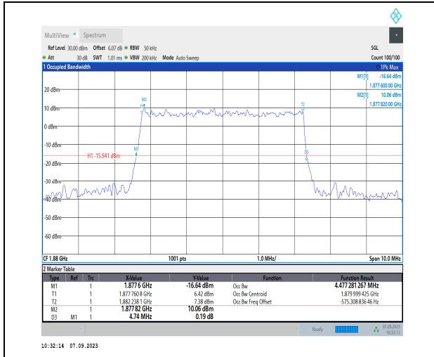
1-N2-PC3-15-5-M-5-DFT-256QAM-Outer_Full-25@0 -Ant2-4.477-4.740- \leq 5 -PASS
