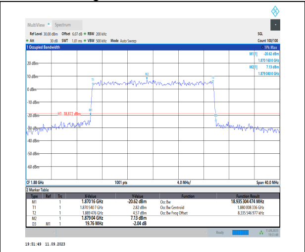
1-N2-PC3-15-20-M-7-CP-16QAM-Outer_Full-106@0-Ant2-18.935-19.760-≤20-PASS
