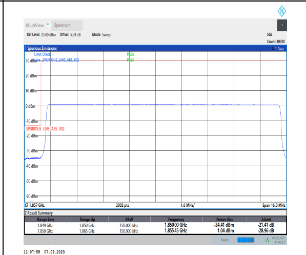
1-N2-PC3-15-15-L-6-CP-QPSK-Outer_Full-79 @0-Ant2-1-seegraph-PASS-see graph
