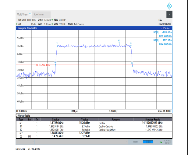
1-N2-PC3-15-15-M-6-CP-QPSK-Outer_Full-79@0-A nt2-14.151-14.790-≤15-PASS
