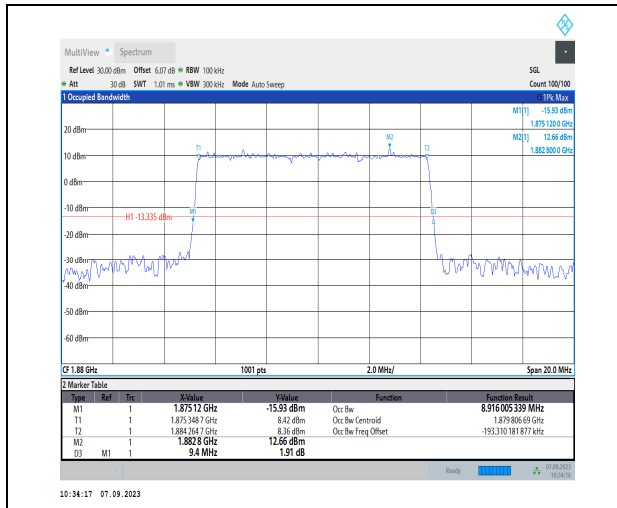
1-N2-PC3-15-10-M-4-DFT-64QAM-Outer_Full-50@0-Ant2-8.916-9.400-≤10-PASS
