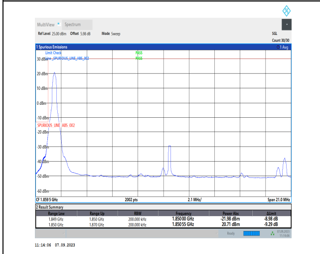
1-N2-PC3-15-20-L-4-CP-QPSK-Edge_1RB_Left-1@0-Ant2-1-seegraph-PASS-see graph
