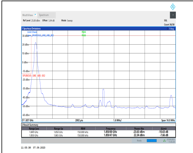
1-N2-PC3-15-15-L-1-DFT-PI2BPSK-Edge_1RB_Left-1 @0-Ant2-1-seegraph-PASS-see graph
