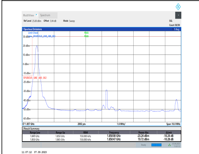
1-N2-PC3-15-15-L-4-CP-QPSK-Edge_1RB_Left-1 @0-Ant2-1-seegraph-PASS-see graph
