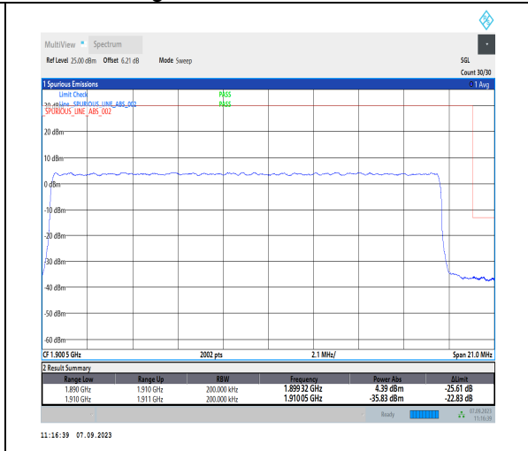
1-N2-PC3-15-20-H-3-DFT-PI2BPSK-Outer_Full-100@0-Ant2-1-seegraph-PASS-see graph
