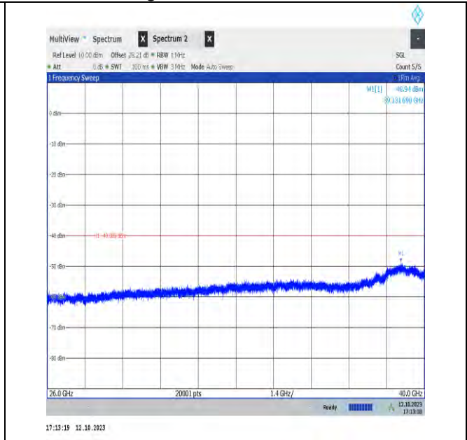
NTVN_N48_PC3_30_40_M_TID1_NS_01_26000_40000_#1
