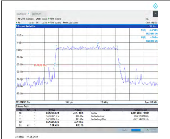
1-N48-PC3-30-10-M-9-CP-256QAM-Outer_Full-24@ 0-Ant5-8.585-9.140-≤10-PASS
