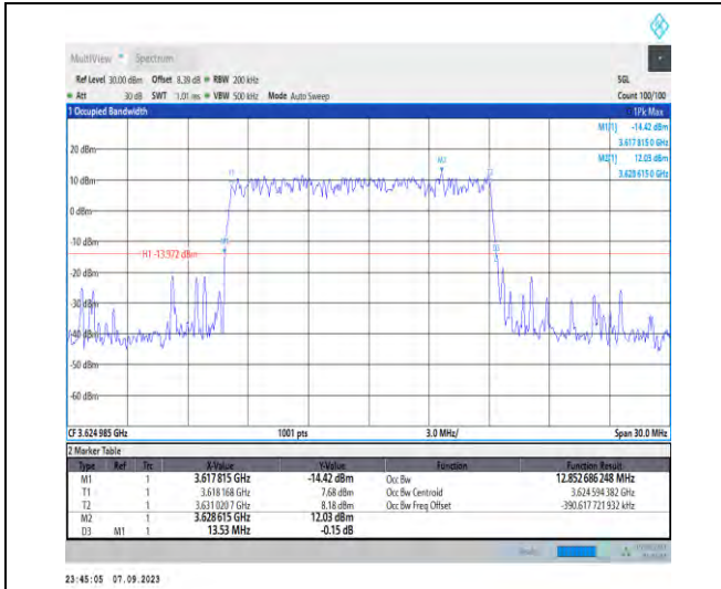
1-N48-PC3-30-15-M-4-DFT-64QAM-Outer_Full-36@ 0-Ant5-12.853-13.530-≤15-PASS
