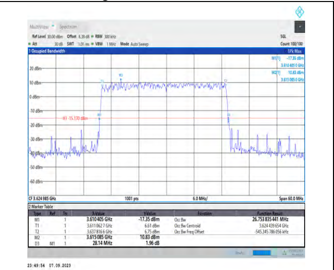
1-N48-PC3-30-30-M-3-DFT-16QAM-Outer_Full-75 @0-Ant5-26.754-28.140-≤30-PASS
