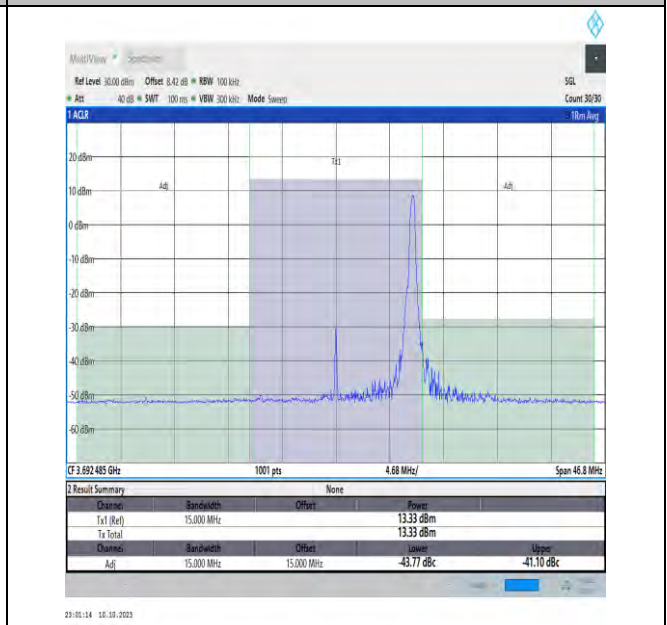
NTVN_N48_PC3_30_15_H_TID18_#1_-15_15
