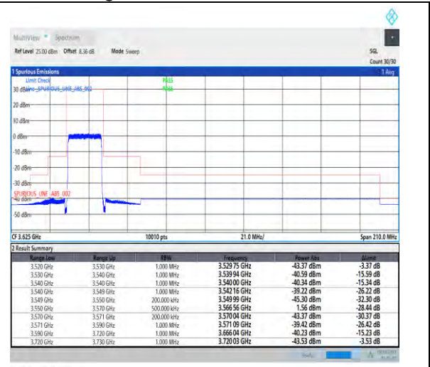
1-N48-PC3-30-20-L-3-DFT-PI2BPSK-Outer_Full-50@0-Ant5-1--PASS-see graph
