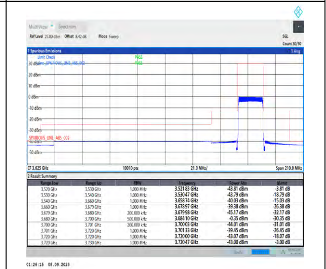
1-N48-PC3-30-20-H-6-CP-QPSK-Outer_Full-51@0-Ant5-1--PASS-see graph
