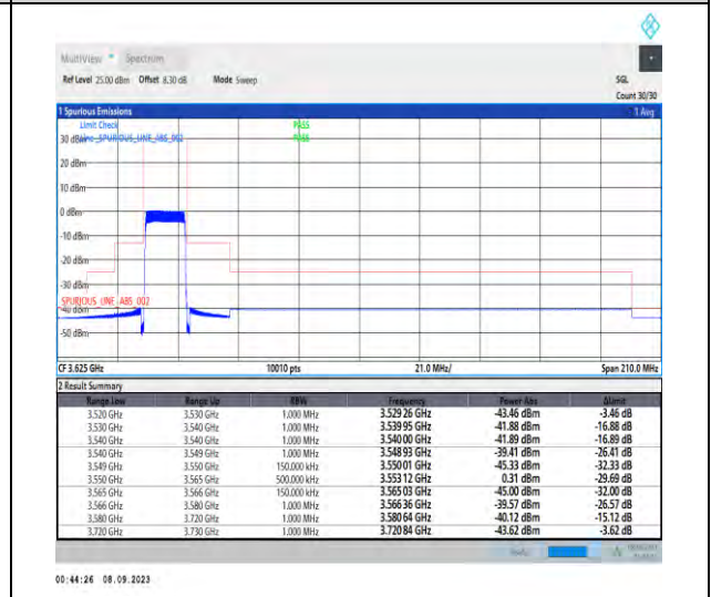
1-N48-PC3-30-15-L-6-CP-QPSK-Outer_Full-38@0-Ant5-1--PASS-see graph
