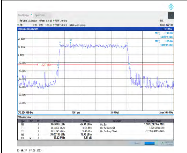
1-N48-PC3-30-15-M-2-DFT-PI2BPSK-Outer_Full-36@ 0-Ant5-12.875-13.620-≤15-PASS
