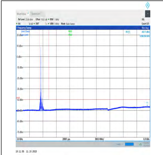
NTNV_N48_PC3_30_40_L_TID1_NS_01_3000_6000_#1
