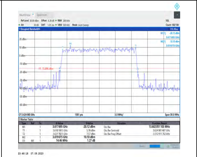
1-N48-PC3-30-15-M-7-CP-16QAM-Outer_Full-38@0- Ant5-13.602-14.460-≤15-PASS
