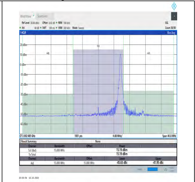
NTVN_N48_PC3_30_15_H_TID3_#1_-15_15
