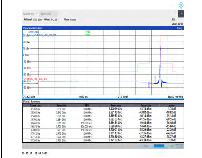
1-N48-PC3-30-15-H-5-CP-QPSK-Edge_1RB_Right-1@37-Ant5-1--PASS-see graph
