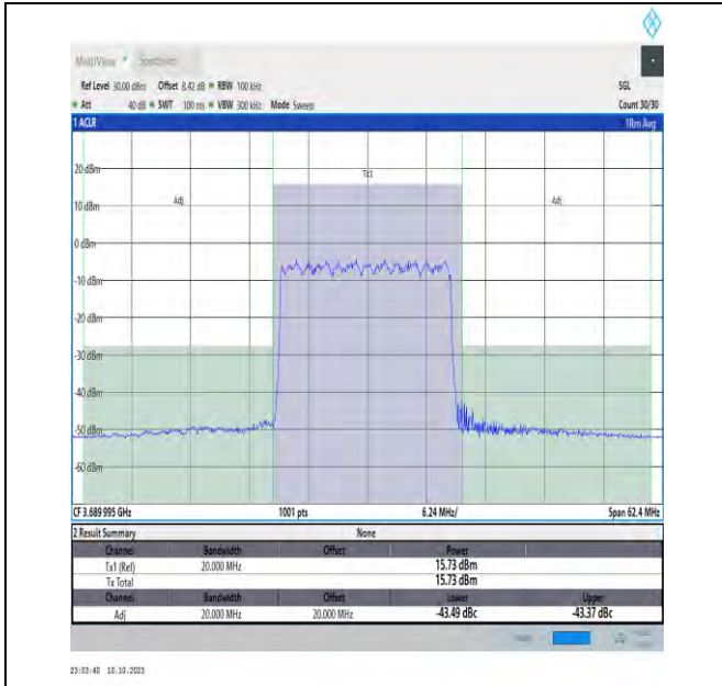
NTVN_N48_PC3_30_20_H_TID1_#1_-20_20
