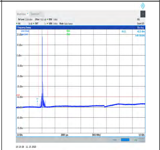
NTNV_N48_PC3_30_40_M_TID1_NS_01_3000_6000_#1
