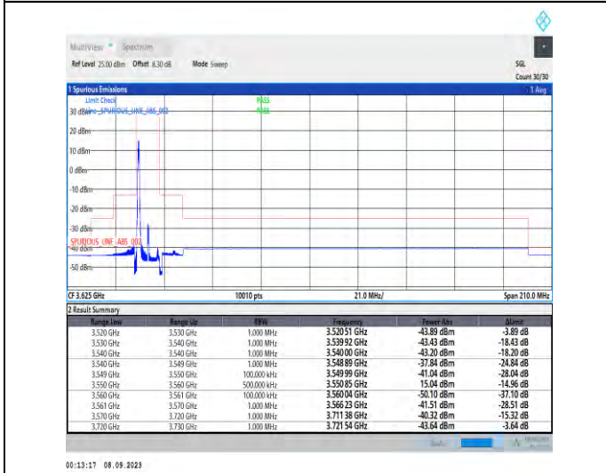
1-N48-PC3-30-10-L-4-CP-QPSK-Edge_1RB_Left-1@0-Ant5-1--PASS-see graph
