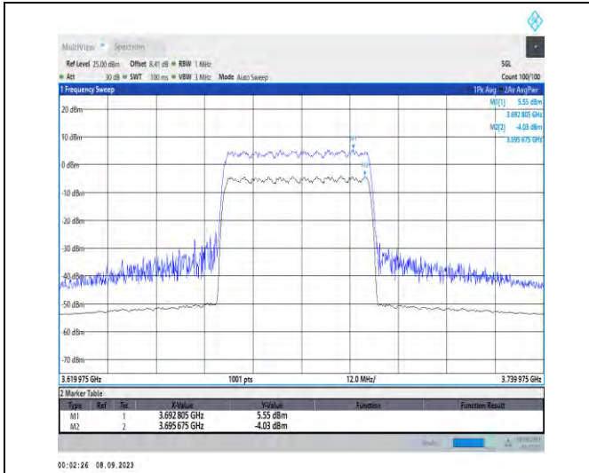
1-N48-PC3-30-40-H-1-DFT-256QAM-Outer_Full-100 @0-Ant5-9.58-100%-0.00-9.58-PASS≤13
