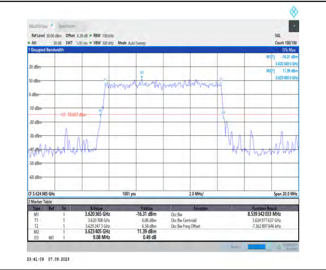
1-N48-PC3-30-10-M-4-DFT-64QAM-Outer_Full-24@0 -Ant5-8.539-9.080-≤10-PASS
