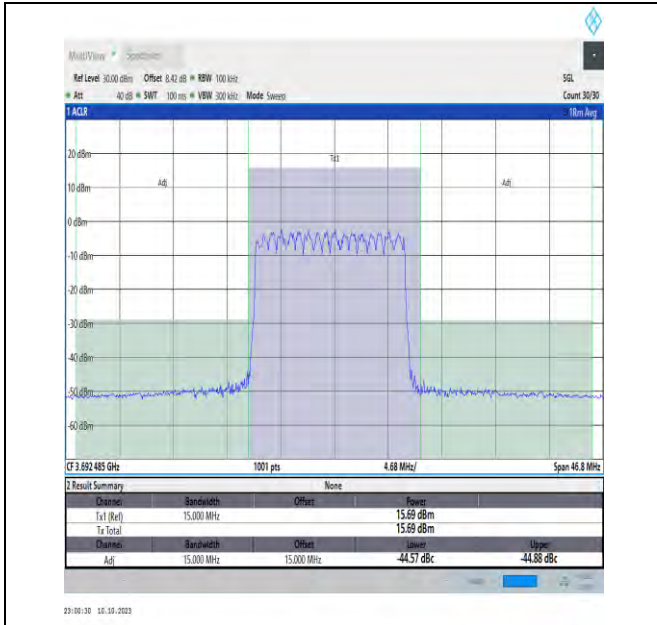
NTVN_N48_PC3_30_15_H_TID1_#1_-15_15
