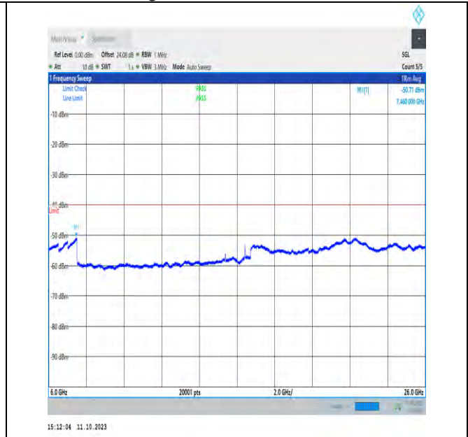
NTNV_N48_PC3_30_40_L_TID1_NS_01_6000_26000_#1
