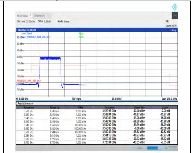
1-N48-PC3-30-30-L-3-DFT-PI2BPSK-Outer_Full-75@0-Ant5-1--PASS-see graph
