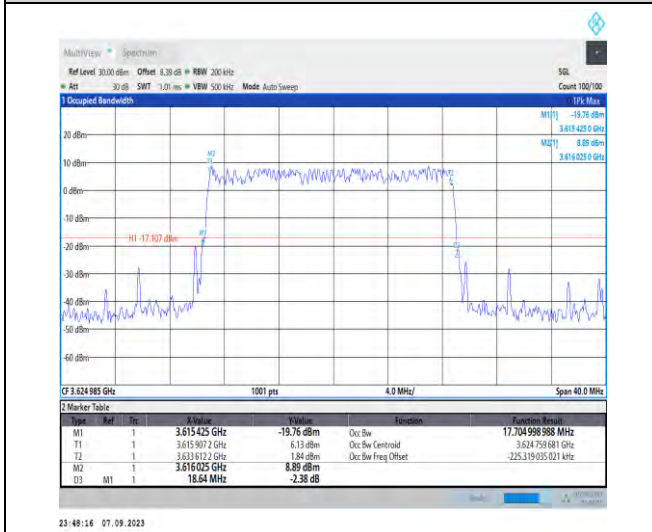
1-N48-PC3-30-20-M-5-DFT-256QAM-Outer_Full-50@ 0-Ant5-17.705-18.640-≤20-PASS
