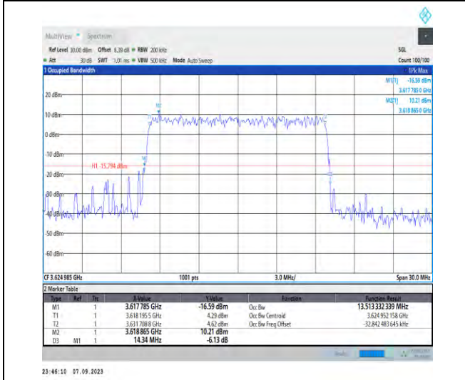
1-N48-PC3-30-15-M-6-CP-QPSK-Outer_Full-38@0- Ant5-13.513-14.340-≤15-PASS
