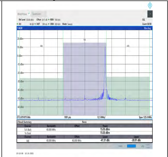
NTVN_N48_PC3_30_40_H_TID3_#1_-40_40
