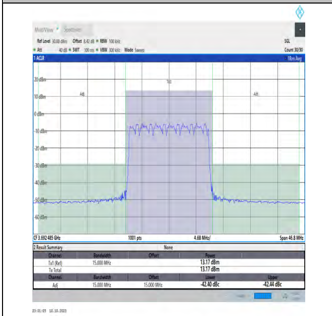
NTVN_N48_PC3_30_15_H_TID16_#1_-15_15
