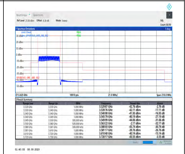
1-N48-PC3-30-30-L-6-CP-QPSK-Outer_Full-78@0-Ant5-1--PASS-see graph
