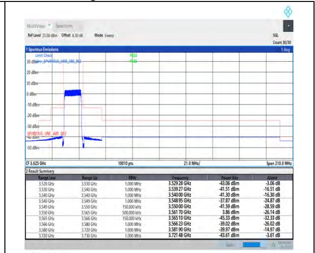
1-N48-PC3-30-15-L-3-DFT-PI2BPSK-Outer_Full-36@0-Ant5-1--PASS-see graph
