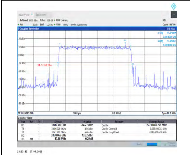
1-N48-PC3-30-40-M-3-DFT-16QAM-Outer_Full-100@0-Ant5-35.74-37.680-≤40-PASS
