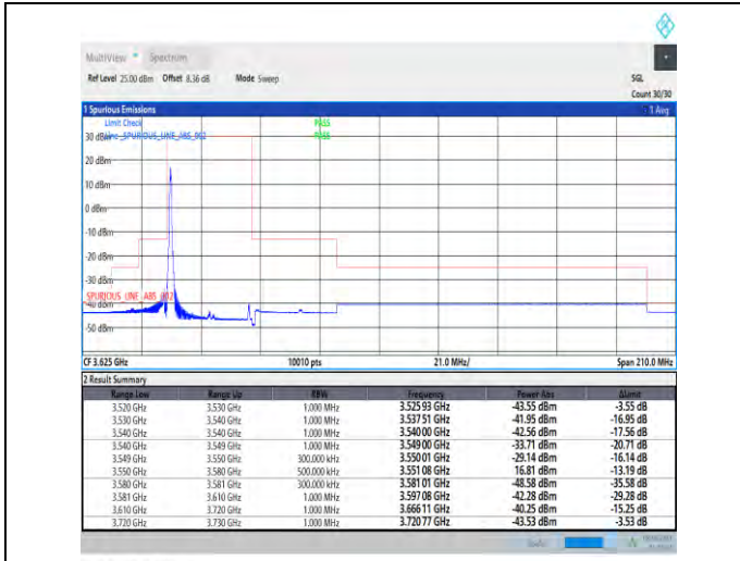
1-N48-PC3-30-30-L-1-DFT-PI2BPSK-Edge_1RB_Left-1@0-Ant5-1--PASS-see graph
