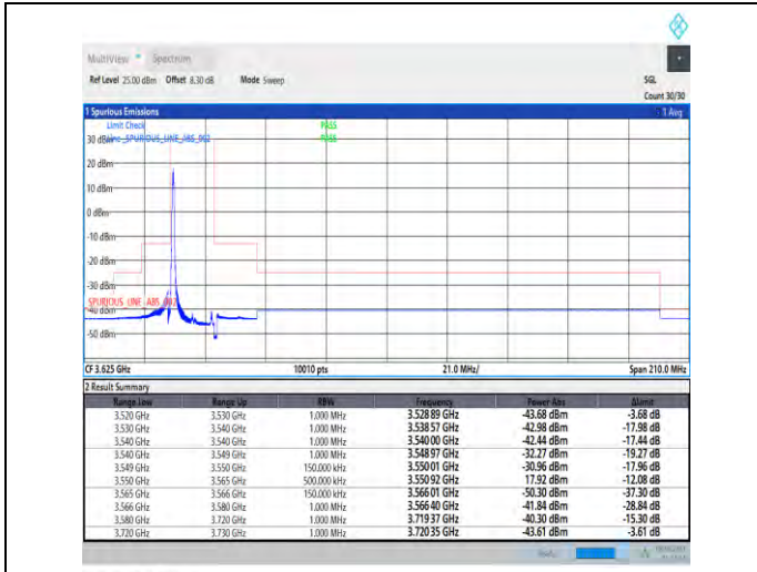
1-N48-PC3-30-15-L-1-DFT-PI2BPSK-Edge_1RB_Left-1@0-Ant5-1--PASS-see graph
