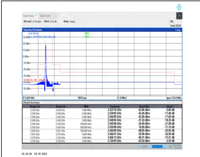
1-N48-PC3-30-10-L-1-DFT-PI2BPSK-Edge_1RB_Left-1@0-Ant5-1--PASS-see graph
