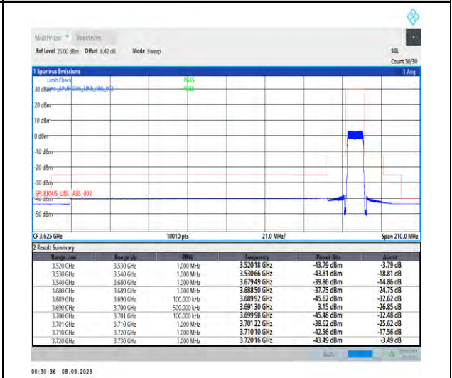
1-N48-PC3-30-10-H-6-CP-QPSK-Outer_Full-24@0-Ant5-1--PASS-see graph
