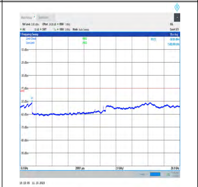
NTNV_N48_PC3_30_40_H_TID1_NS_01_6000_26000_#
