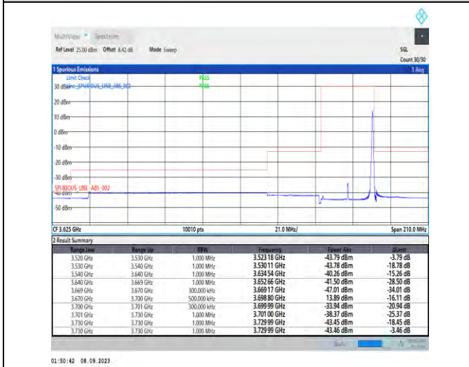
1-N48-PC3-30-30-H-5-CP-QPSK-Edge_1RB_Right-1@77-Ant5-1--PASS-see graph
