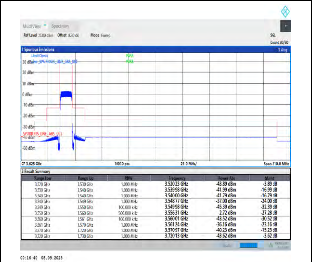
1-N48-PC3-30-10-L-6-CP-QPSK-Outer_Full-24@0-Ant5-1--PASS-see graph
