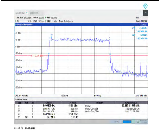
1-N48-PC3-30-40-M-1-DFT-QPSK-Outer_Full-100@0-Ant5-35.837-37.200-≤40-PASS
