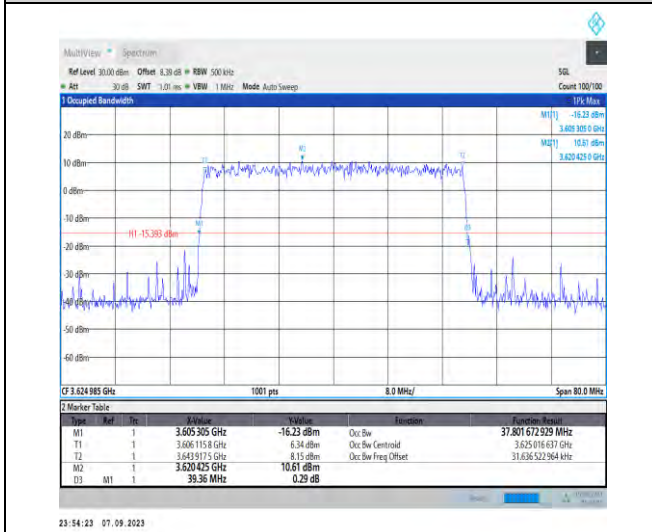
1-N48-PC3-30-40-M-7-CP-16QAM-Outer_Full-106@0-Ant5-37.802-39.360-≤40-PASS
