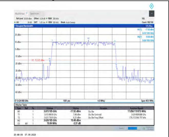
1-N48-PC3-30-20-M-4-DFT-64QAM-Outer_Full-50@ 0-Ant5-17.856-19.040-≤20-PASS
