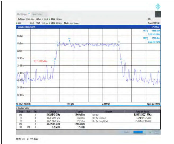
1-N48-PC3-30-10-M-1-DFT-QPSK-Outer_Full-24@0 -Ant5-8.554-9.200-≤10-PASS
