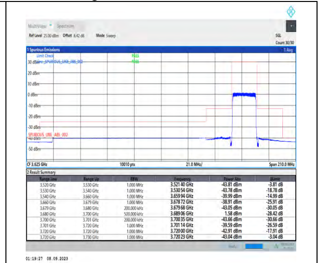
1-N48-PC3-30-20-H-3-DFT-PI2BPSK-Outer_Full-50@0-Ant5-1--PASS-see graph
