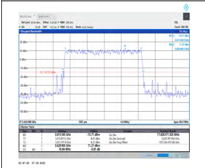
1-N48-PC3-30-20-M-1-DFT-QPSK-Outer_Full-50@0 -Ant5-17.828-18.840-≤20-PASS
