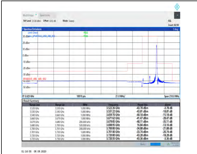
1-N48-PC3-30-20-H-2-DFT-PI2BPSK-Edge_1RB_Right-t-1@50-Ant5-1--PASS-see graph
