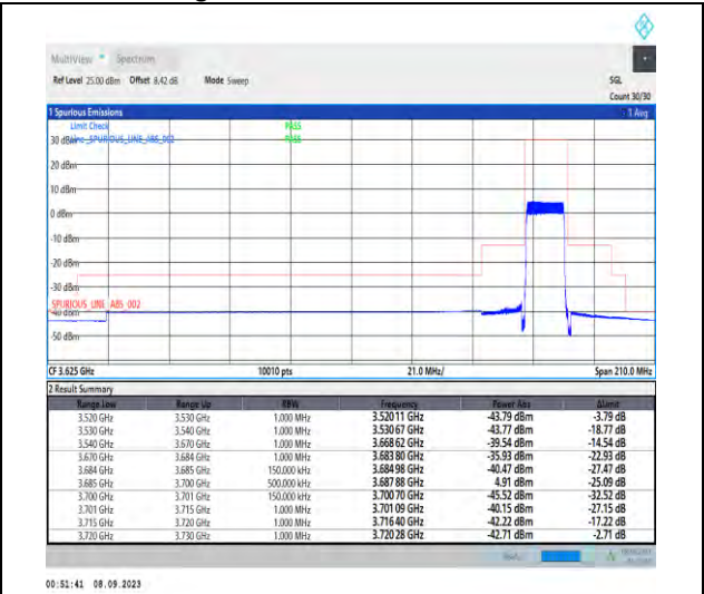
1-N48-PC3-30-15-H-3-DFT-PI2BPSK-Outer_Full-36@0-Ant5-1--PASS-see graph
