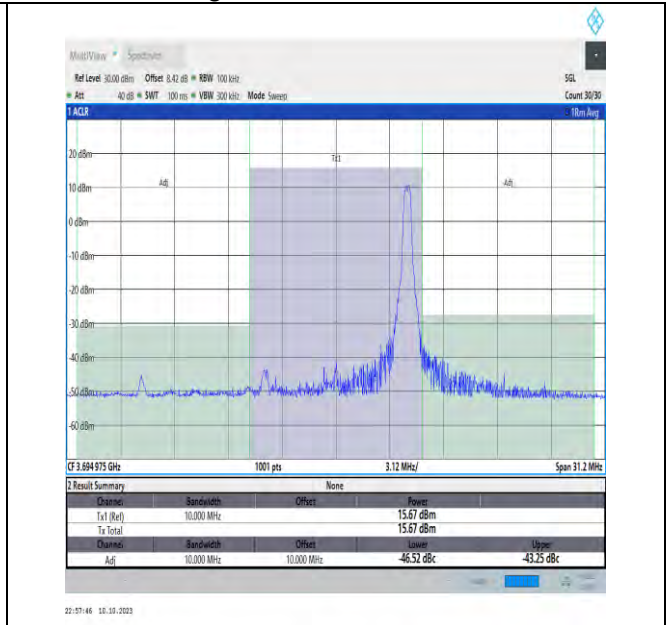
NTVN_N48_PC3_30_10_H_TID3_#1_-10_10
