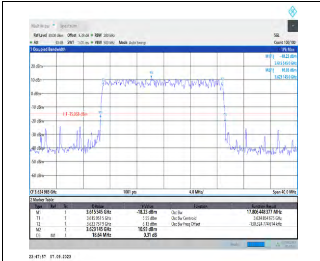
1-N48-PC3-30-20-M-3-DFT-16QAM-Outer_Full-50@ 0-Ant5-17.806-18.640-≤20-PASS
