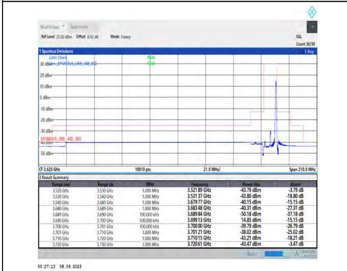
1-N48-PC3-30-10-H-5-CP-QPSK-Edge_1RB_Right-1@23-Ant5-1--PASS-see graph
