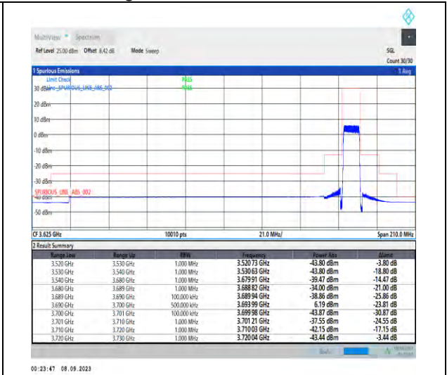
1-N48-PC3-30-10-H-3-DFT-PI2BPSK-Outer_Full-24@0-Ant5-1--PASS-see graph
