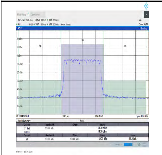
NTVN_N48_PC3_30_10_H_TID16_#1_-10_10
