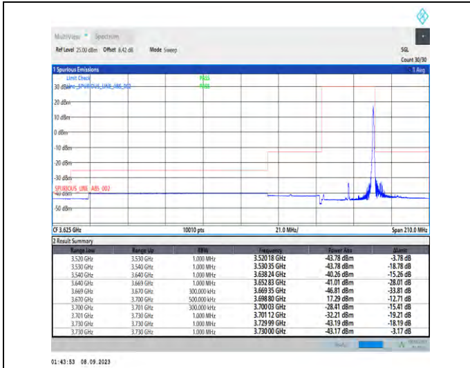
1-N48-PC3-30-30-H-2-DFT-PI2BPSK-Edge_1RB_Right-t-1@77-Ant5-1--PASS-see graph
