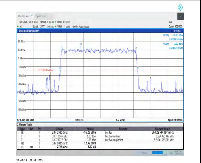
1-N48-PC3-30-30-M-1-DFT-QPSK-Outer_Full-75@0 -Ant5-26.823-27.900-≤30-PASS
