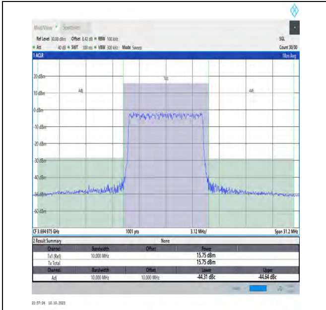
NTVN_N48_PC3_30_10_H_TID1_#1_-10_10
