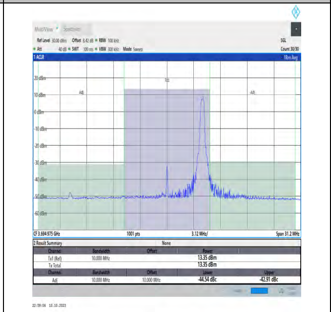
NTVN_N48_PC3_30_10_H_TID18_#1_-10_10
