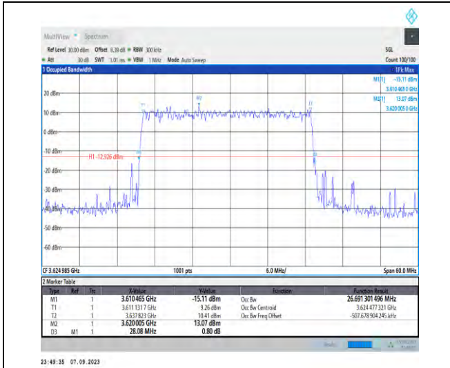
1-N48-PC3-30-30-M-2-DFT-PI2BPSK-Outer_Full-75 @0-Ant5-26.691-28.080-≤30-PASS
