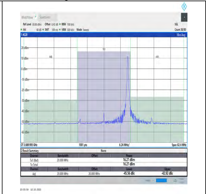
NTVN_N48_PC3_30_20_H_TID3_#1_-20_20
