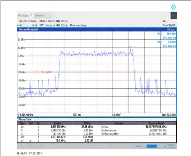
1-N48-PC3-30-20-M-9-CP-256QAM-Outer_Full-51@0 0-Ant5-18.188-19.000-≤20-PASS
