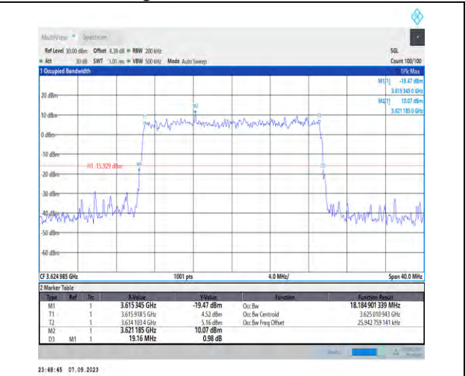
1-N48-PC3-30-20-M-8-CP-64QAM-Outer_Full-51@0 -Ant5-18.185-19.160-≤20-PASS
