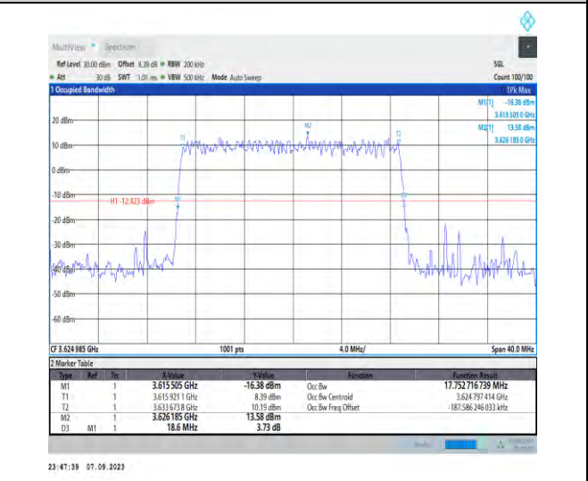
1-N48-PC3-30-20-M-2-DFT-PI2BPSK-Outer_Full-50@0 -Ant5-17.753-18.600-≤20-PASS
