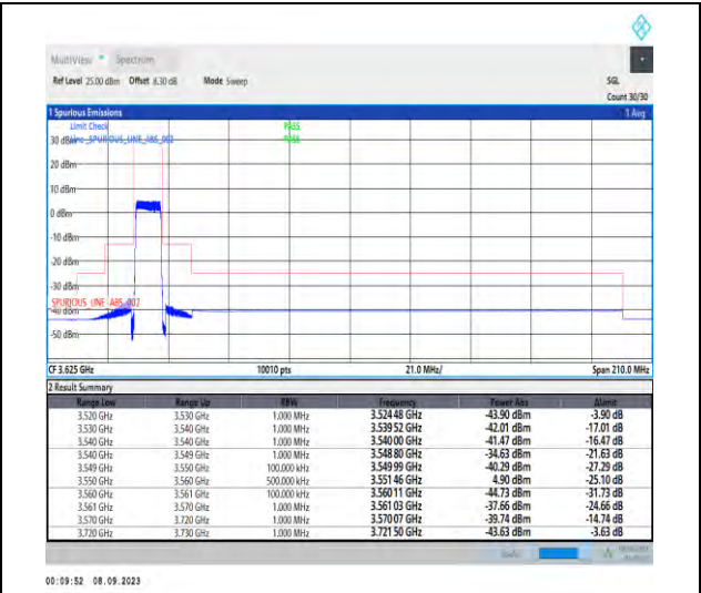
1-N48-PC3-30-10-L-3-DFT-PI2BPSK-Outer_Full-24@0-Ant5-1--PASS-see graph
