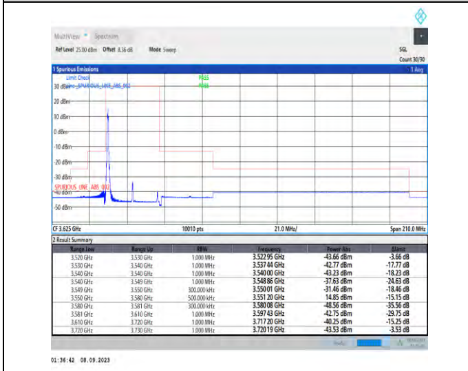
1-N48-PC3-30-30-L-4-CP-QPSK-Edge_1RB_Left-1@0-Ant5-1--PASS-see graph
