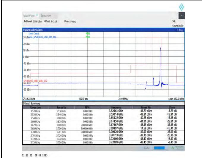
1-N48-PC3-30-20-H-5-CP-QPSK-Edge_1RB_Right-1@50-Ant5-1--PASS-see graph
