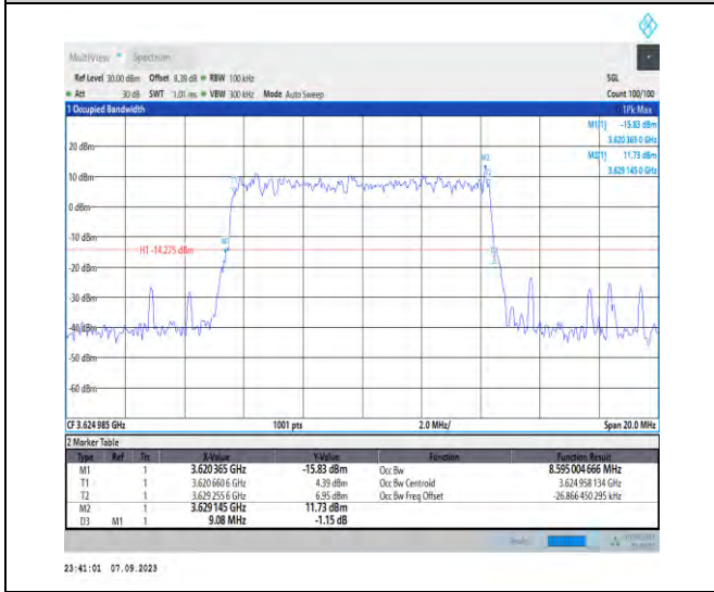
1-N48-PC3-30-10-M-3-DFT-16QAM-Outer_Full-24@0 -Ant5-8.595-9.080-≤10-PASS
