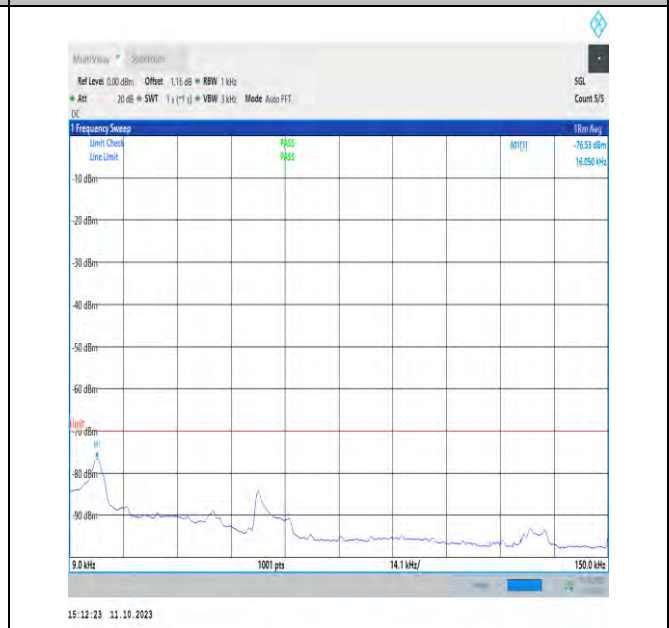
NTNV_N48_PC3_30_40_M_TID1_NS_01_0.009_0.15_#1
