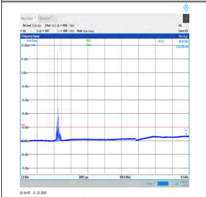
NTNV_N48_PC3_30_40_H_TID1_NS_01_3000_6000_#1
