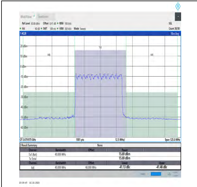
NTVN_N48_PC3_30_40_H_TID1_#1_-40_40
