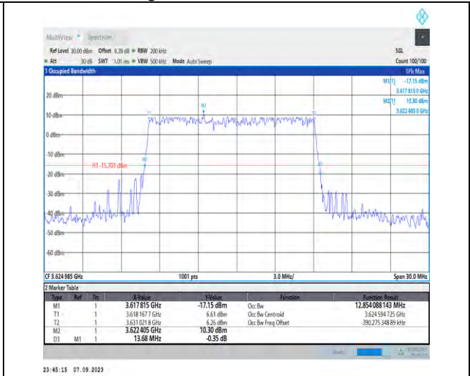
1-N48-PC3-30-15-M-5-DFT-256QAM-Outer_Full-36@ 0-Ant5-12.854-13.680-≤15-PASS
