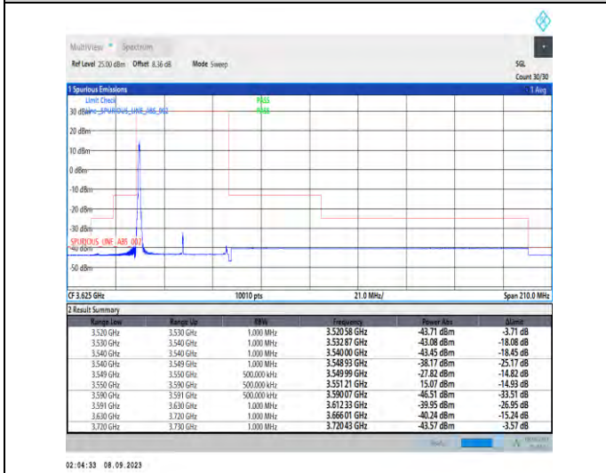
1-N48-PC3-30-40-L-4-CP-QPSK-Edge_1RB_Left-1@0-Ant5-1--PASS-see graph
