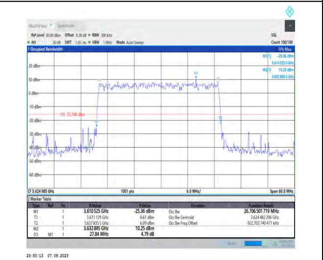
1-N48-PC3-30-30-M-5-DFT-256QAM-Outer_Full-75 @0-Ant5-26.707-27.840-≤30-PASS
