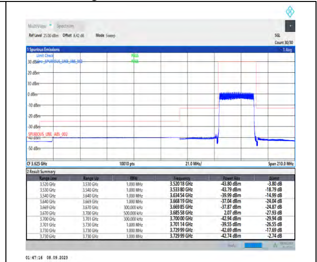
1-N48-PC3-30-30-H-3-DFT-PI2BPSK-Outer_Full-75@0-Ant5-1--PASS-see graph
