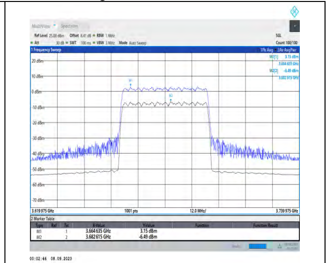
1-N48-PC3-30-40-H-2-CP-256QAM-Outer_Full-106 @0-Ant5-9.64-100%-0.00-9.64-PASS≤13
