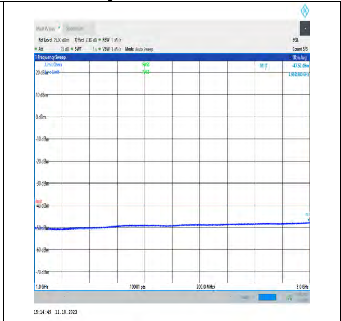
NTNV_N48_PC3_30_40_H_TID1_NS_01_1000_3000_#1
