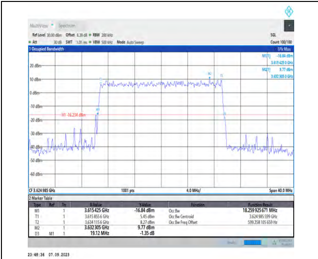
1-N48-PC3-30-20-M-7-CP-16QAM-Outer_Full-51@0 -Ant5-18.26-19.120-≤20-PASS
