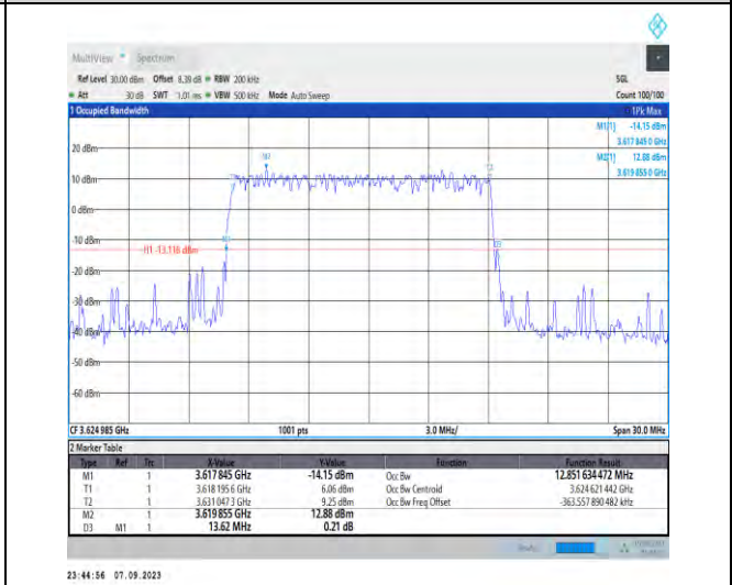
1-N48-PC3-30-15-M-3-DFT-16QAM-Outer_Full-36@ 0-Ant5-12.852-13.620-≤15-PASS
