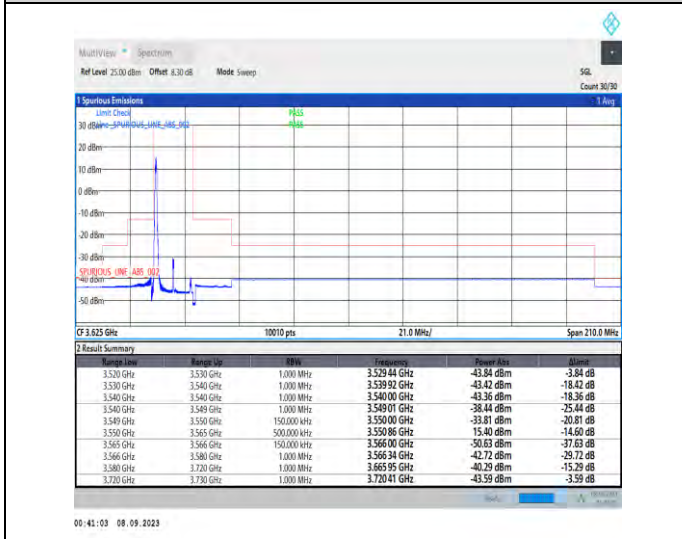
1-N48-PC3-30-15-L-4-CP-QPSK-Edge_1RB_Left-1@0-Ant5-1--PASS-see graph
