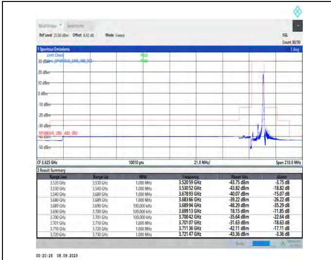
1-N48-PC3-30-10-H-2-DFT-PI2BPSK-Edge_1RB_Right-t-1@23-Ant5-1--PASS-see graph
