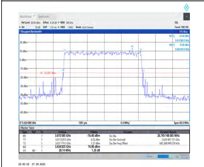
1-N48-PC3-30-30-M-4-DFT-64QAM-Outer_Full-75 @0-Ant5-26.745-28.140-≤30-PASS
