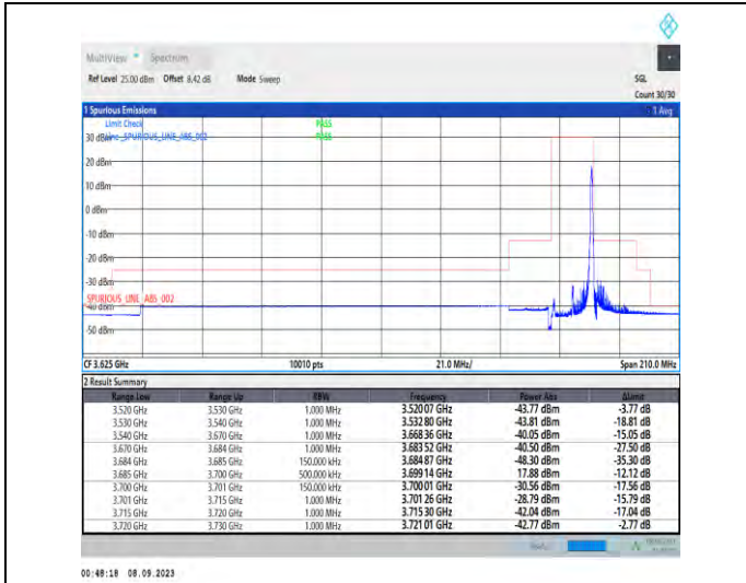
1-N48-PC3-30-15-H-2-DFT-PI2BPSK-Edge_1RB_Right-1@37-Ant5-1--PASS-see graph
