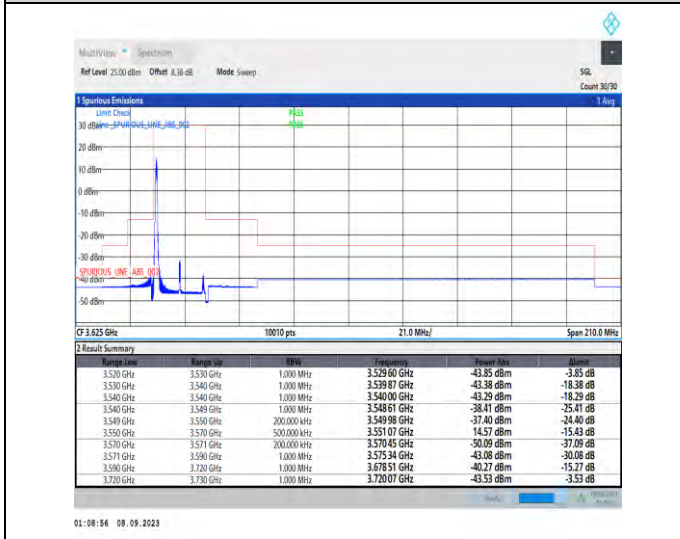
1-N48-PC3-30-20-L-4-CP-QPSK-Edge_1RB_Left-1@0-Ant5-1--PASS-see graph
