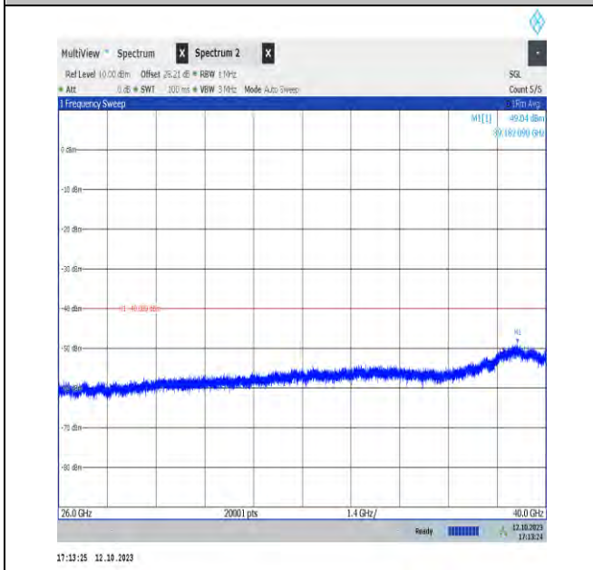
NTNV_N48_PC3_30_40_L_TID1_NS_01_26000_40000_#1
