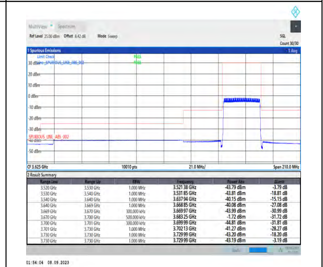
1-N48-PC3-30-30-H-6-CP-QPSK-Outer_Full-78@0-Ant5-1--PASS-see graph
