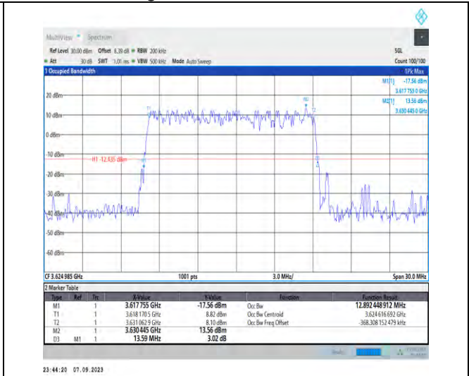
1-N48-PC3-30-15-M-1-DFT-QPSK-Outer_Full-36@ 0-Ant5-12.892-13.590-≤15-PASS
