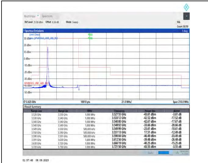
1-N48-PC3-30-40-L-1-DFT-PI2BPSK-Edge_1RB_Left-1@0-Ant5-1--PASS-see graph
