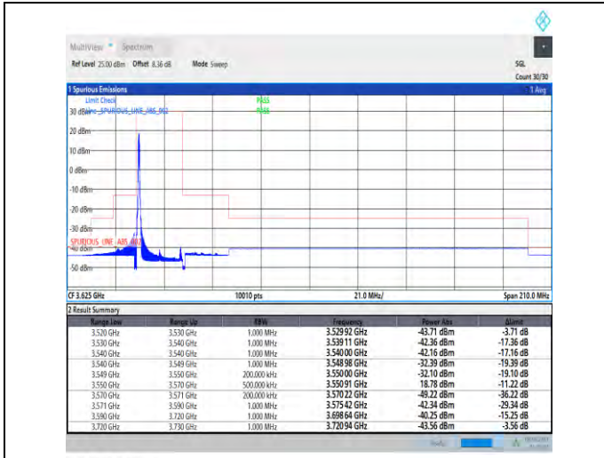
1-N48-PC3-30-20-L-1-DFT-PI2BPSK-Edge_1RB_Left-1@0-Ant5-1--PASS-see graph
