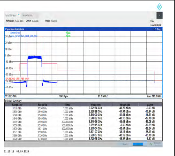
1-N48-PC3-30-20-L-6-CP-QPSK-Outer_Full-51@0-Ant5-1--PASS-see graph
