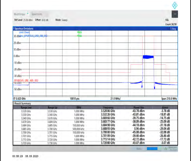
1-N48-PC3-30-15-H-6-CP-QPSK-Outer_Full-38@0-Ant5-1--PASS-see graph
