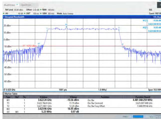
Band48-5MHz-16QAM-55990-25RB#0
