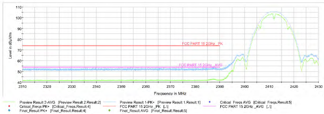
Fig.A.6.2.1 Transmitter Spurious Emission - Radiated (Power): 802.11b, ch1, 2.31 GHz – 2.43GHz
