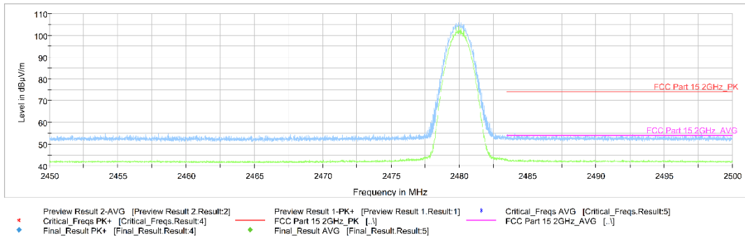
Fig.18. Frequency Band Edges: 8DPSK, Channel 78, 2.45 GHz - 2.50GHz
