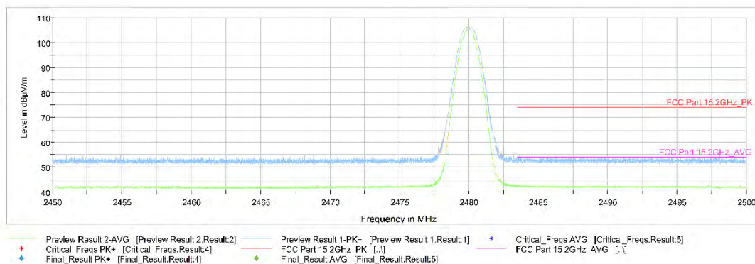
Fig.14. Frequency Band Edges: GFSK, Channel 78, Hopping Off, ch11, 2.45 GHz - 2.50GHz
