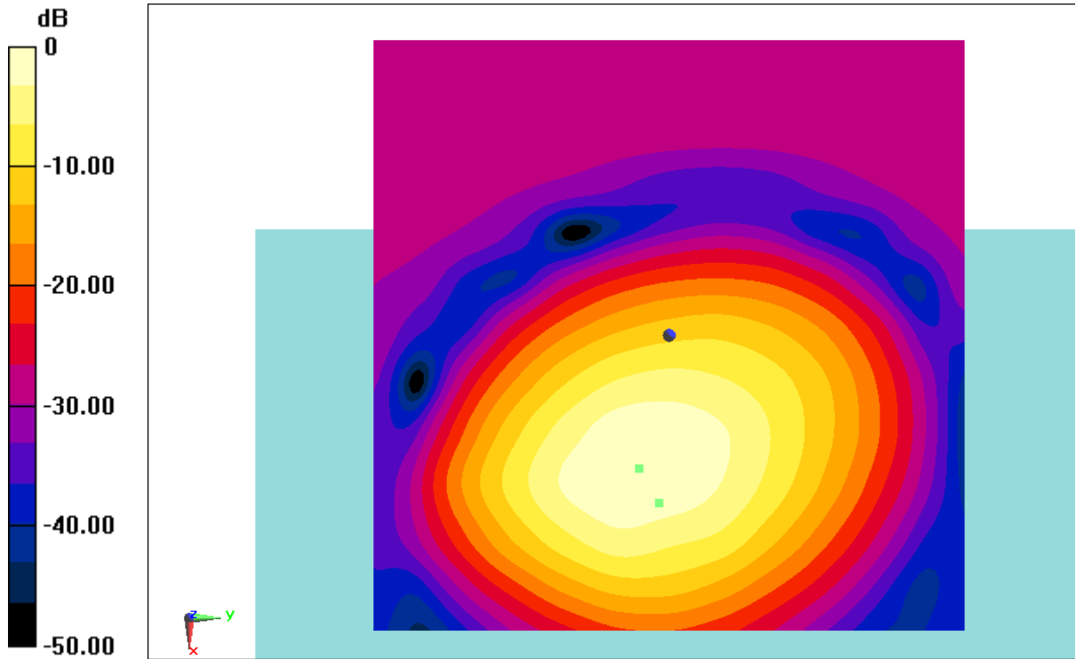
Fig B.4 T-Coil LTE B41
