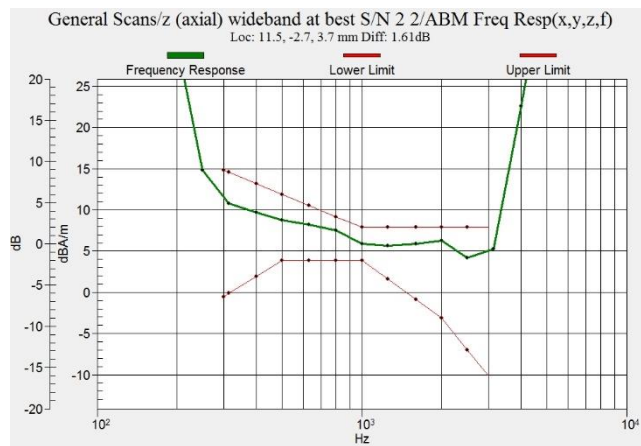
Figure C.2 Frequency Response of LTE B41 PC2
