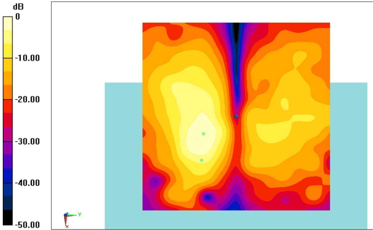
Fig B.11 T-Coil WiFi-2.4G
