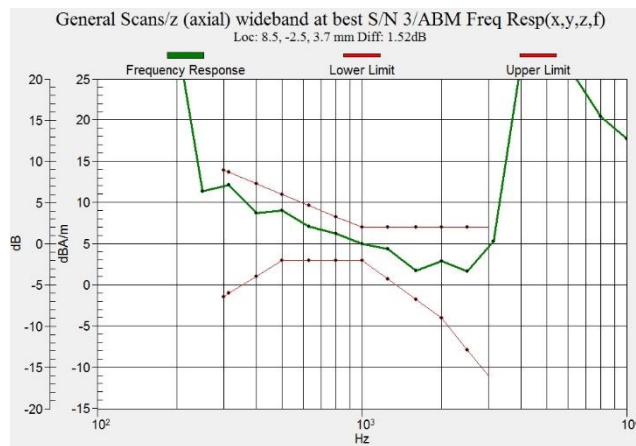
Figure C.5 Frequency Response of LTE B41 PC3 - OTT VoIP
