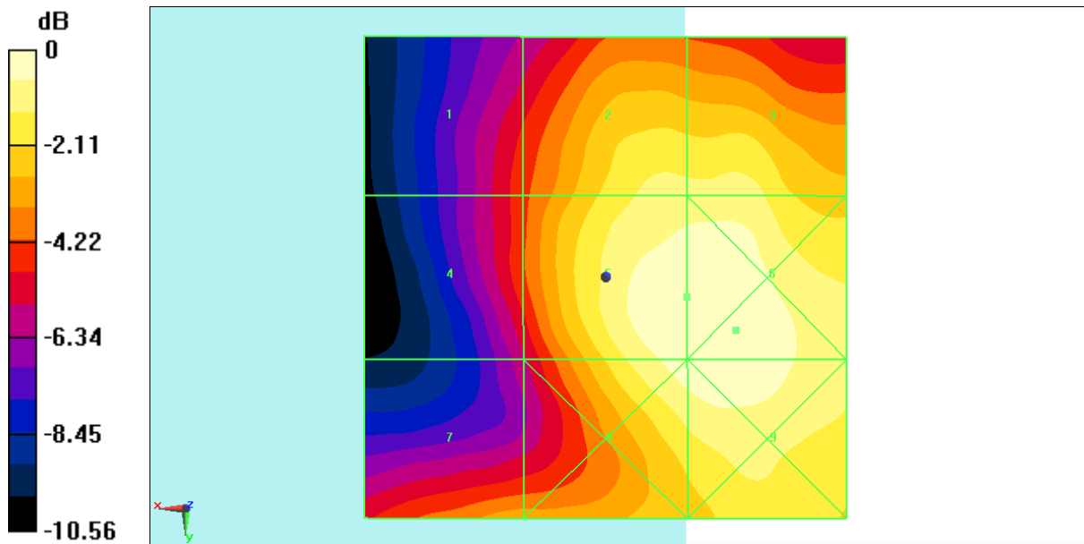
Fig B.2 HAC RF E-Field WIFI 2.4G
