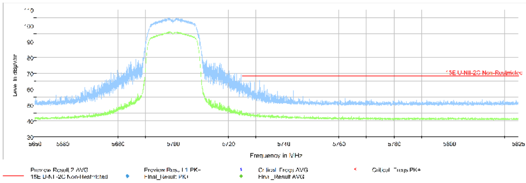
Fig.49 Band Edges (802.11ac-HT20 Ch140, 5700MHz)
