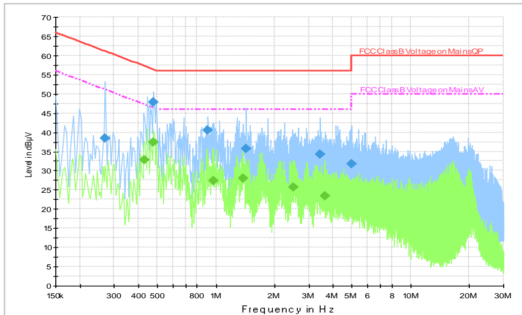
Fig.B.8.3 AC Powerline Conducted Emission- Bluetooth(Second source)
