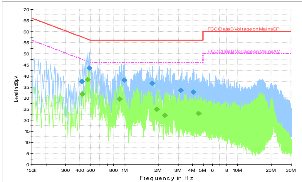
Fig.B.8.2 AC Powerline Conducted Emission-Idle(First source)
