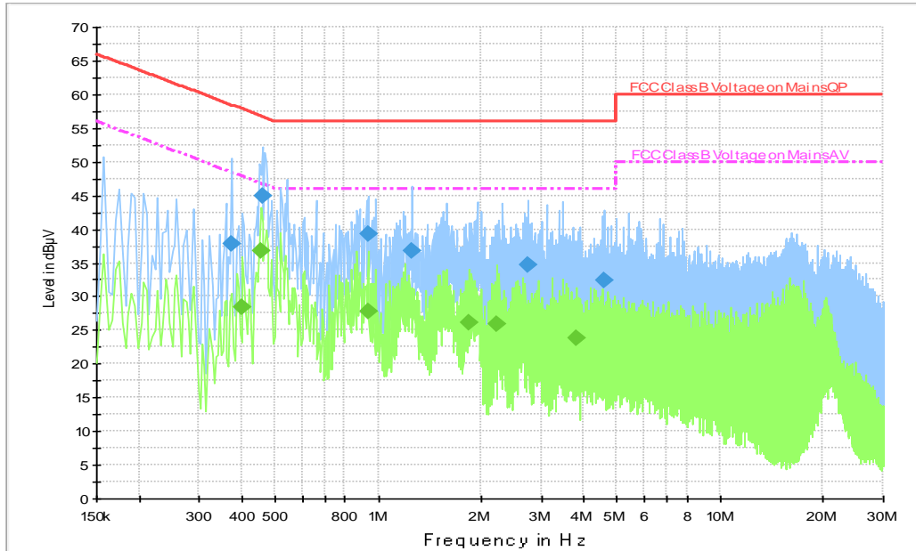
Fig.B.8.1 AC Powerline Conducted Emission- Bluetooth(First source)
