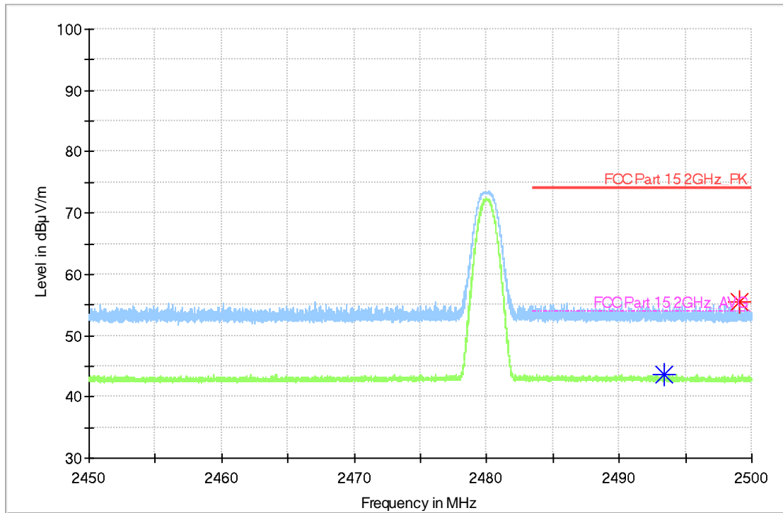
Fig.19. Frequency Band Edges: GFSK, 2480 MHz, Hopping Off , 2.45 GHz - 2.50GHz
