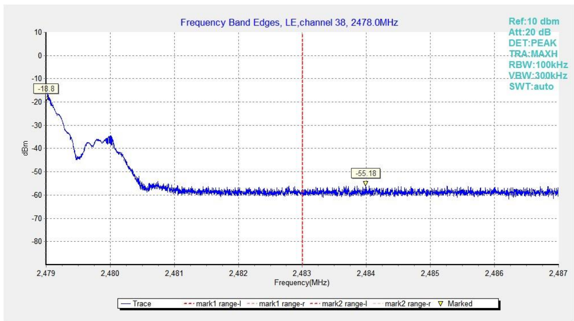
Fig.2. Frequency Band Edges: GFSK, 2478 MHz, Hopping Off
