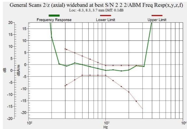
Figure C.19 Frequency Response of CDMA BC1 - OTT VoIP
