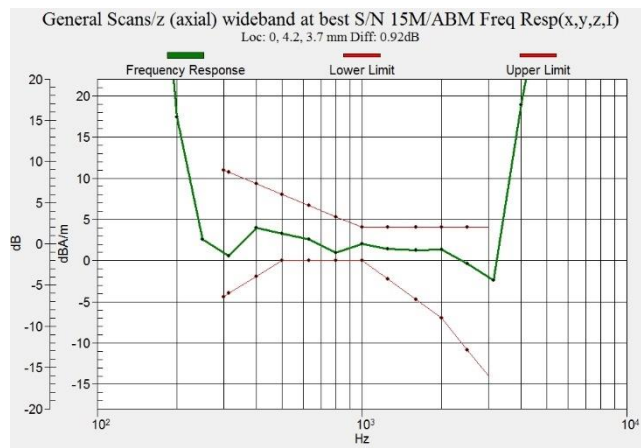
Figure C.20 Frequency Response of LTE B25 - OTT VoIP
