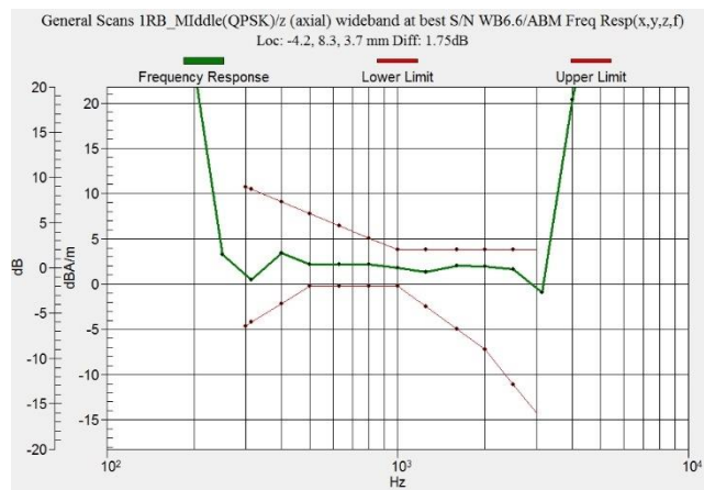
Figure C.21 Frequency Response of LTE B41 Power Class 3 - OTT VoIP
