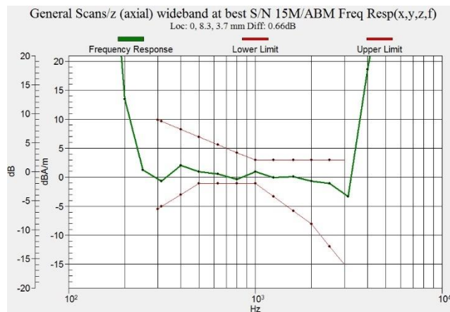
Figure C.18 Frequency Response of W1700 - OTT VoIP
