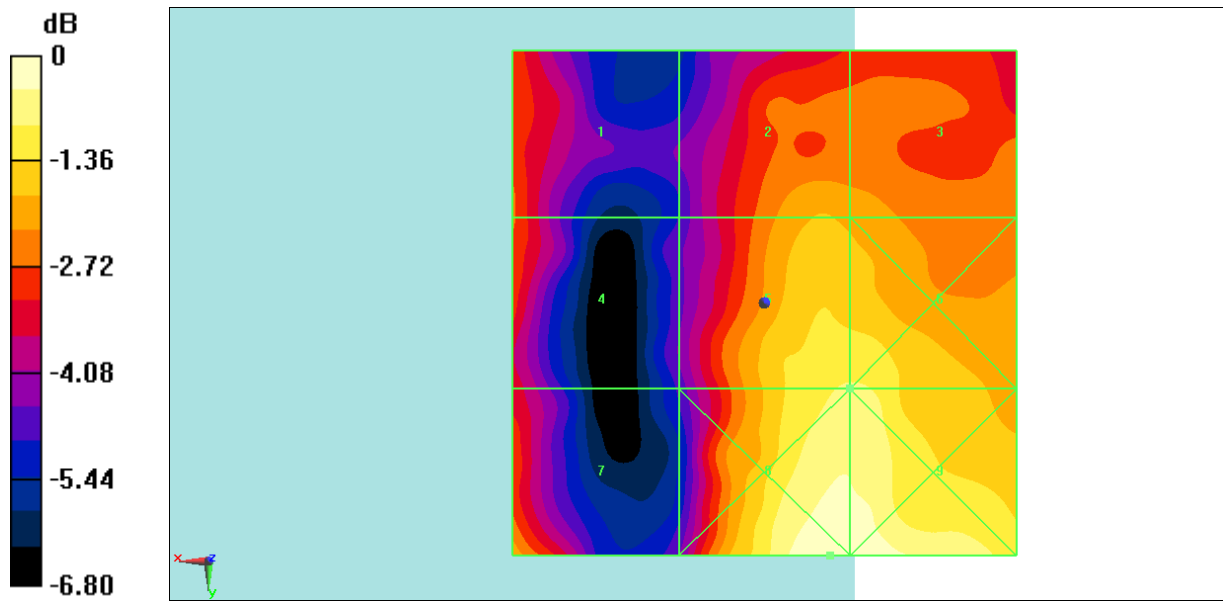
Fig B.42 HAC RF E-Field LTE Band41 Power Class 3 64QAM CH41055
