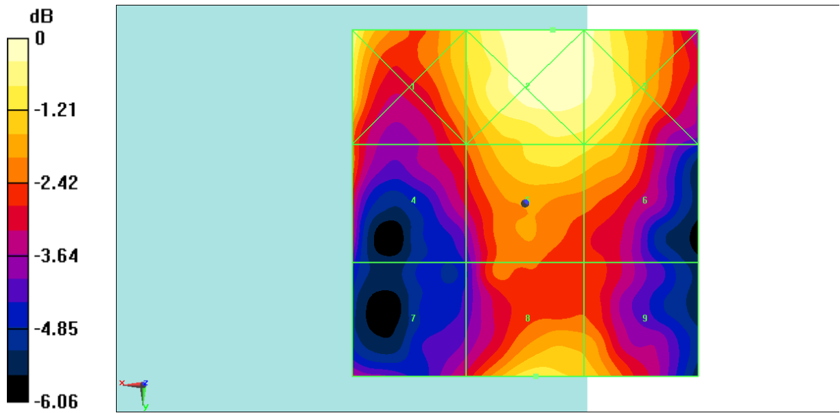
Fig B.30 HAC RF E-Field LTE Band41 Power Class 2 64QAM CH39750
