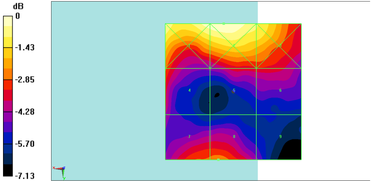
Fig B.18 HAC RF E-Field LTE Band41 Power Class 2 QPSK CH40620
