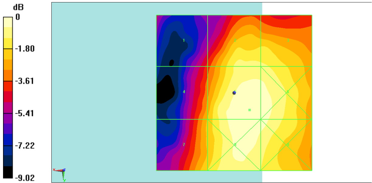
Fig B.45 HAC RF E-Field LTE Band41 Power Class 3 64QAM CH39750
