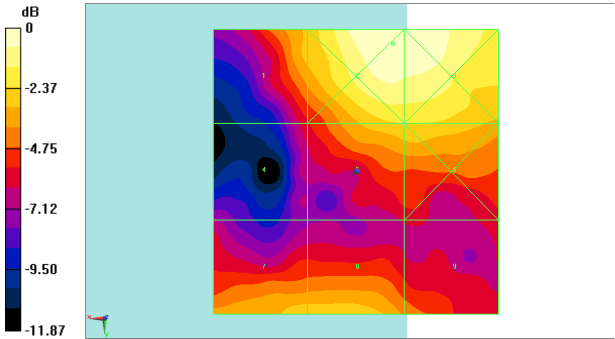
Fig B.12 HAC RF E-Field CDMA BC1 Low
