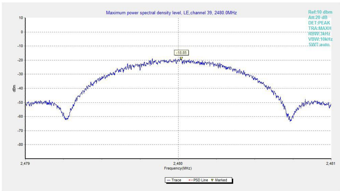
Fig.27. Maximum Power Spectral Density Level Function: GFSK, 2480 MHz
