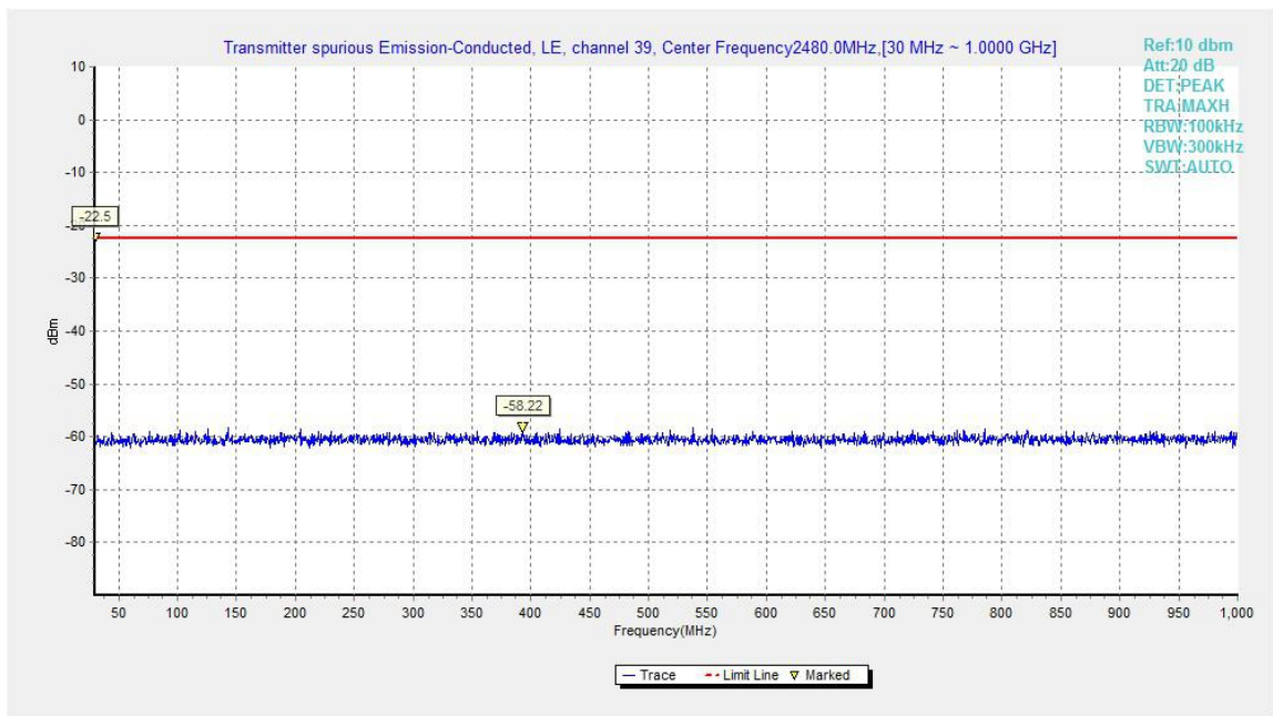
Fig.18. Transmitter Spurious Emission - Conducted: GFSK, 2480 MHz, 30MHz - 1GHz
