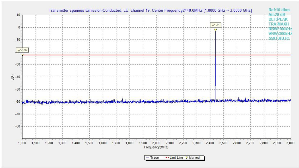
Fig.14. Transmitter Spurious Emission - Conducted: GFSK, 2440 MHz, 1GHz – 3GHz
