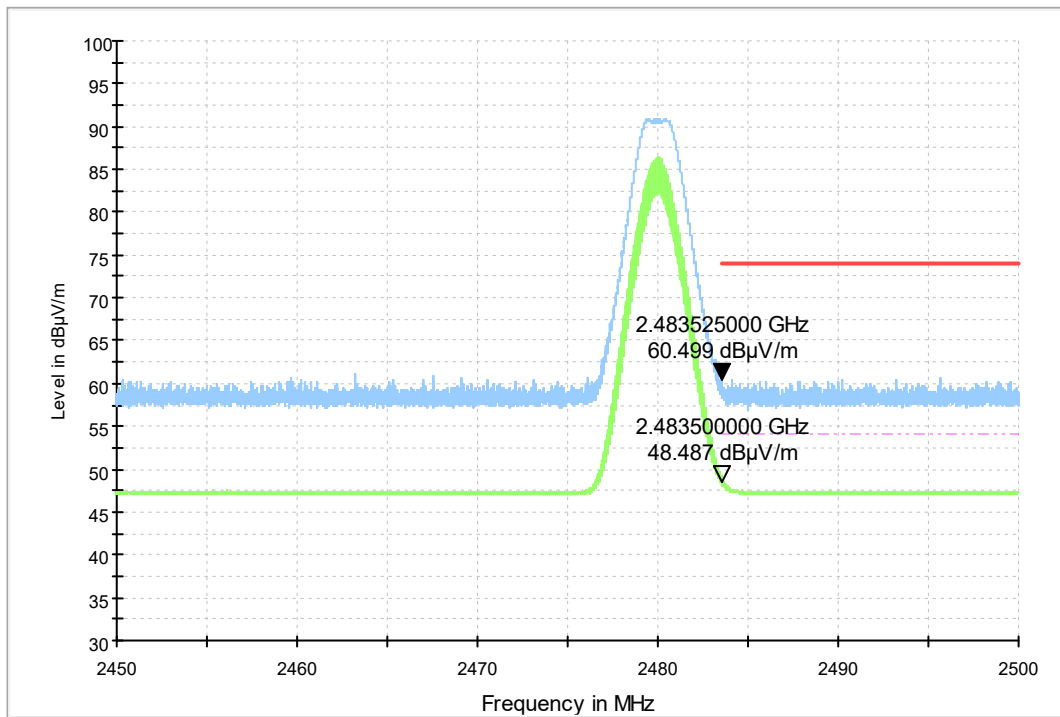
Fig.6. Frequency Band Edges: Bluetooth 5.0 GFSK, 2480 MHz, Hopping Off , 2.45 GHz - 2.50GHz
