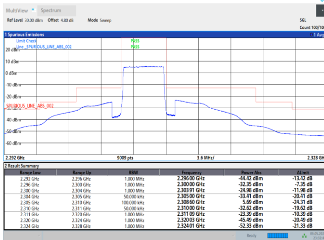
Band30-5MHz-QPSK-27685-25RB#0
