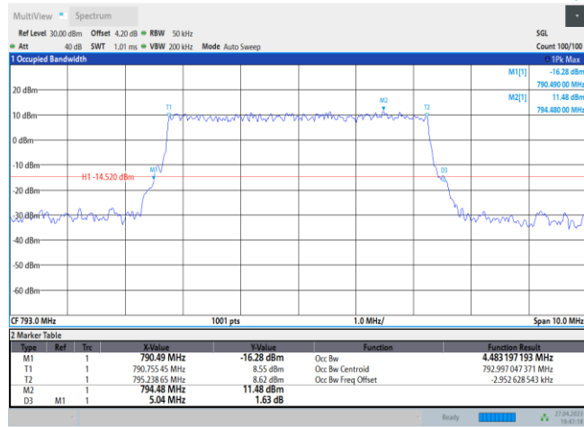
Band14-5MHz-QPSK-23330-25RB#0
