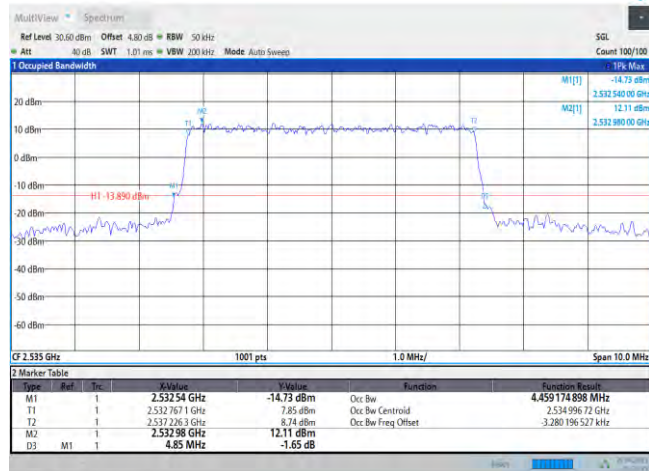
Band7-5MHz-QPSK-21100-25RB#0
