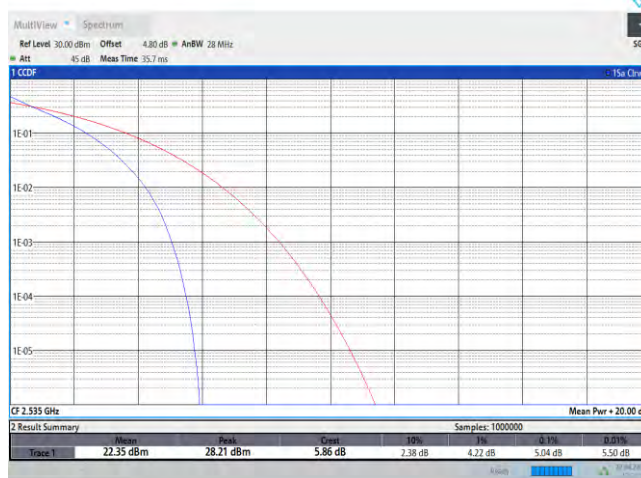
Band7-20MHz-QPSK-21100-100RB#0
