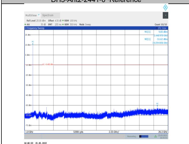
DH5-Ant2-2441-1000~26500
