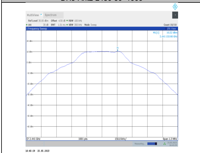
DH5-Ant2-2441-0~Reference
