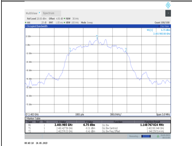
3DH5-Ant2-2402
