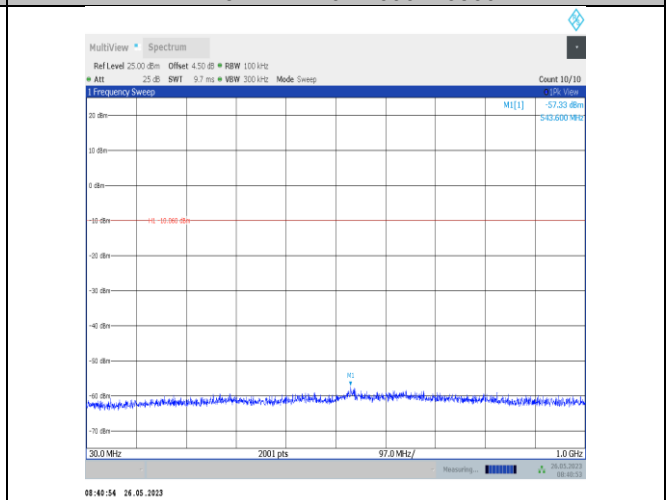
2DH5-Ant2-2441-30~1000
