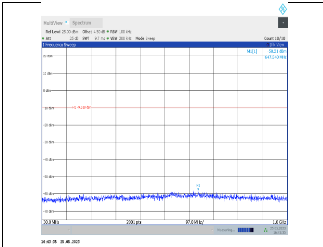
DH5-Ant2-2480-30~1000
