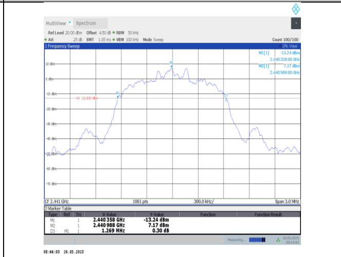
3DH5-Ant2-2441
