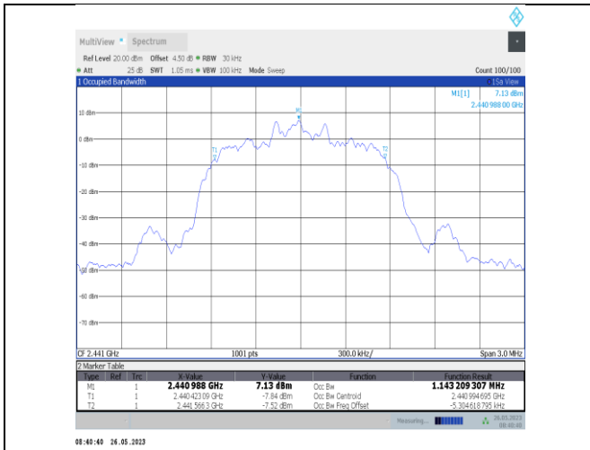
2DH5-Ant2-2441
