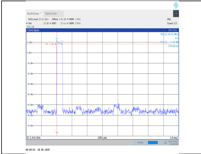
2DH1-Ant2-Hop
