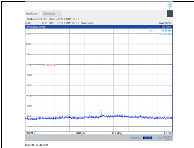
2DH5-Ant2-2402-30~1000
