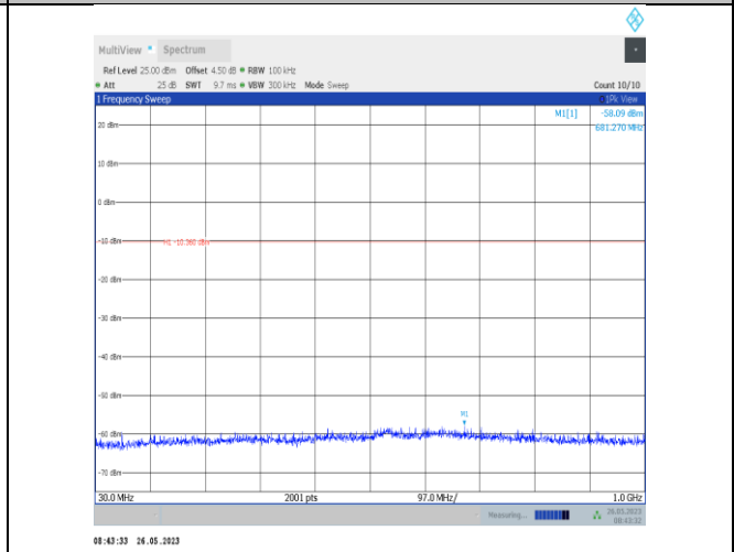
3DH5-Ant2-2402-30~1000
