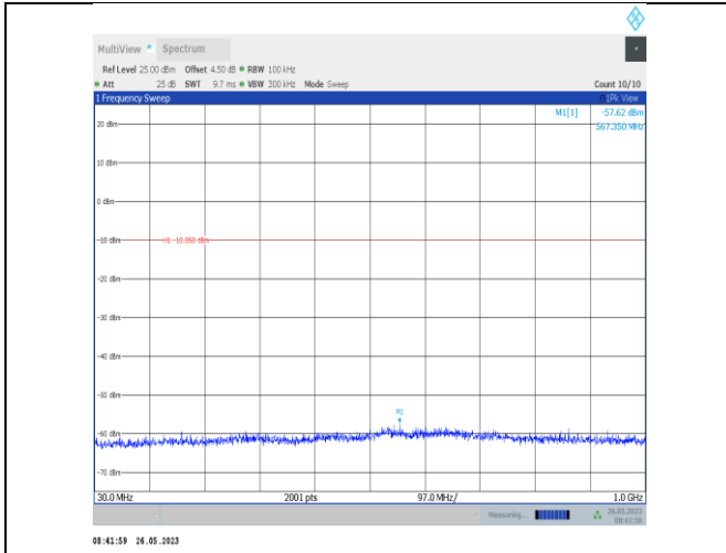
2DH5-Ant2-2480-30~1000
