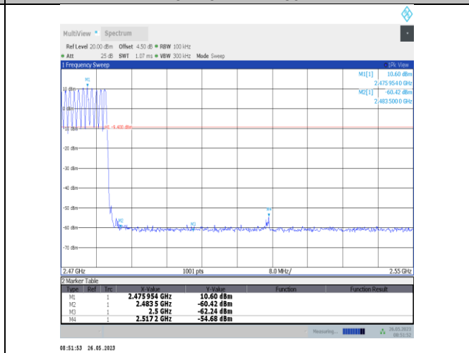
DH5-Ant2-Hop_2480
