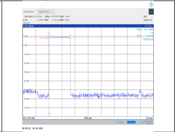
2DH3-Ant2-Hop
