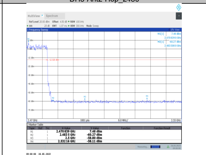
2DH5-Ant2-Hop_2480
