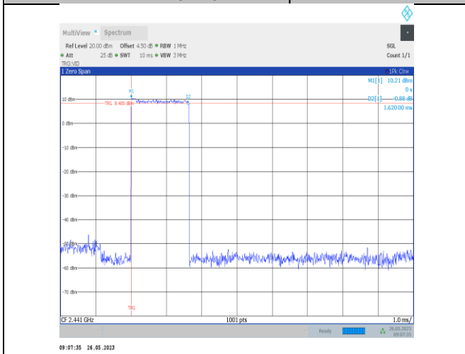
3DH3-Ant2-Hop
