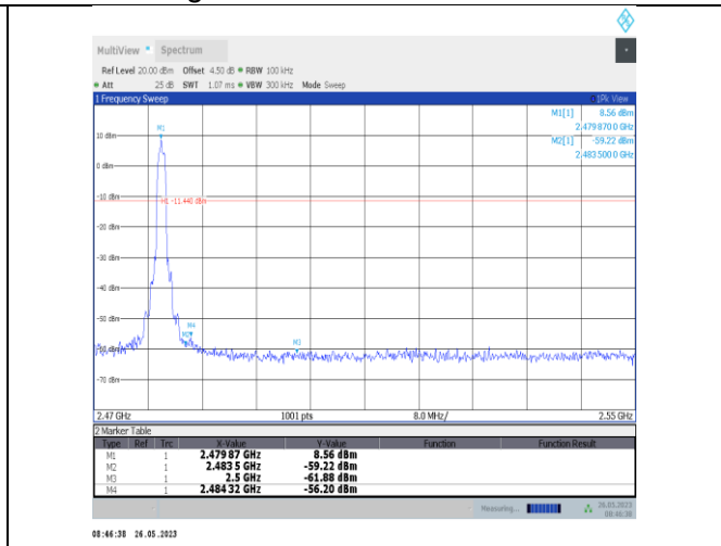
3DH5-Ant2-2480
