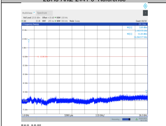
2DH5-Ant2-2441-1000~26500
