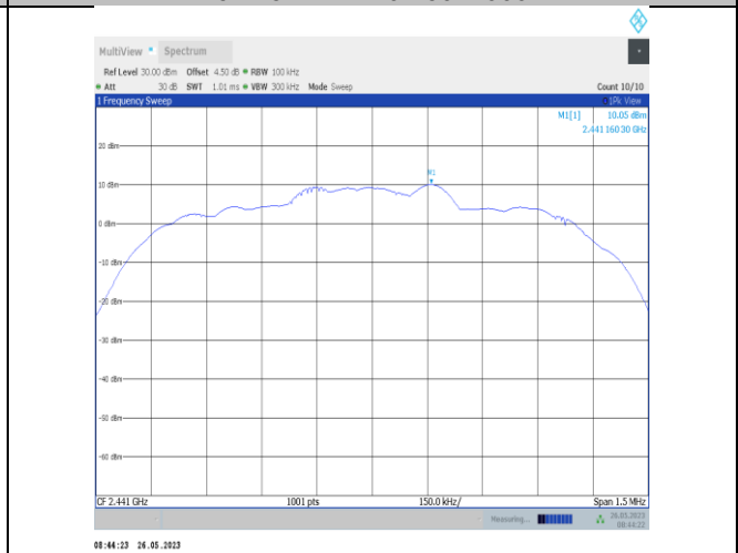
3DH5-Ant2-2441-0~Reference
