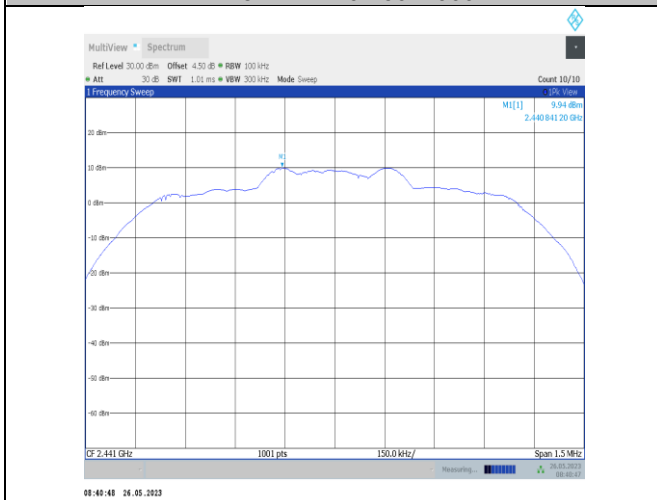
2DH5-Ant2-2441-0~Reference
