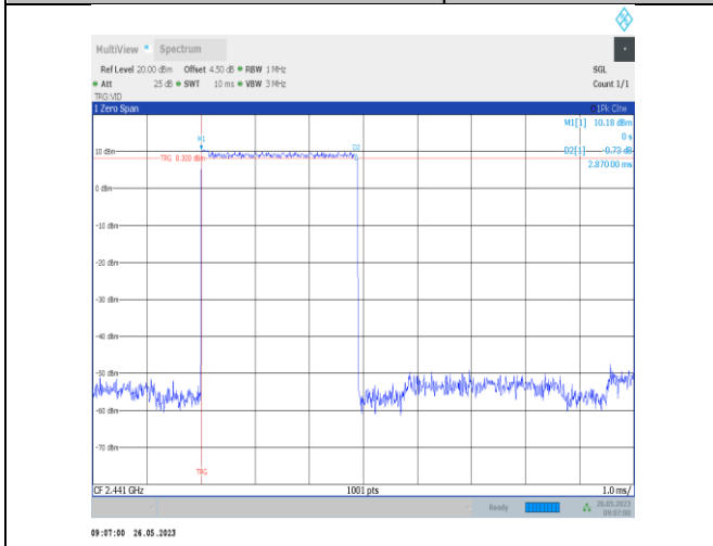
3DH5-Ant2-Hop
