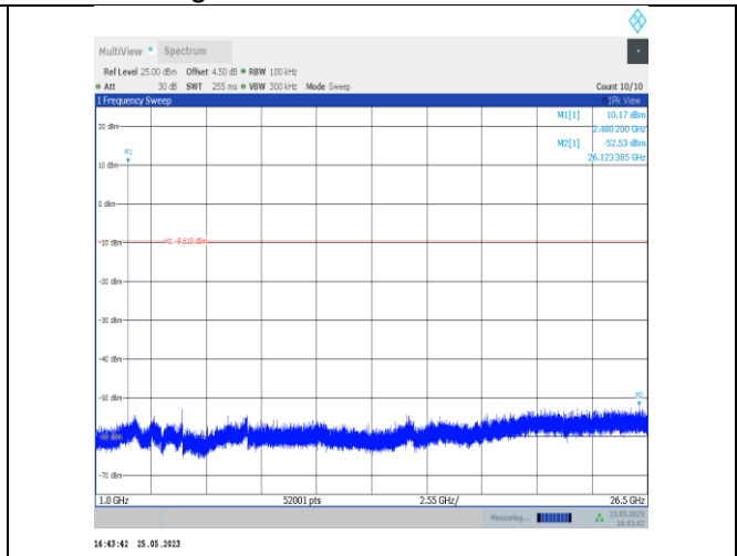
DH5-Ant2-2480-1000~26500
