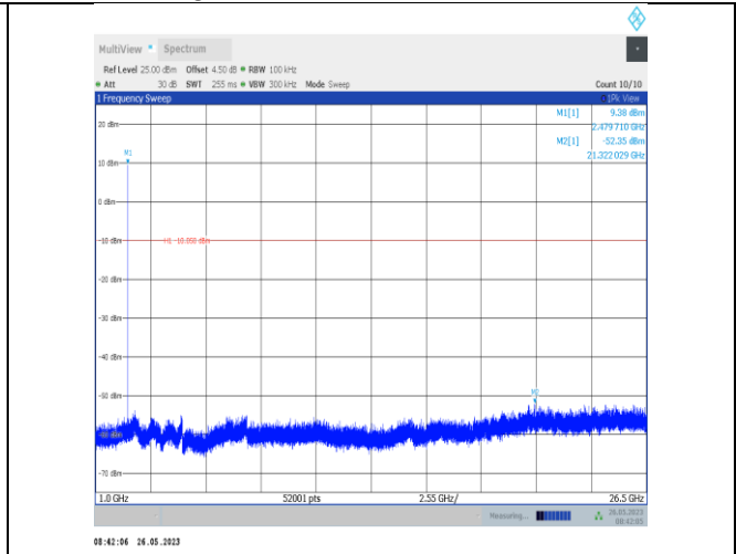
2DH5-Ant2-2480-1000~26500
