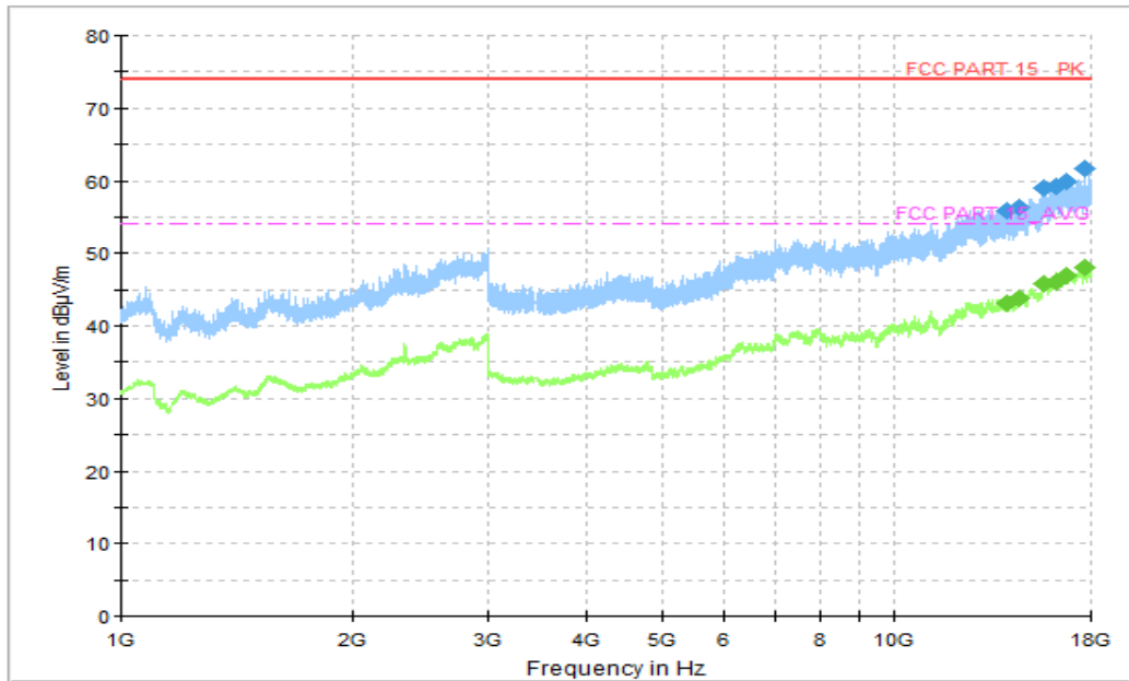
Figure A.1.32. Radiated Emission (Data Transfer: TF Card TO PC, 1GHz to 18GHz)
