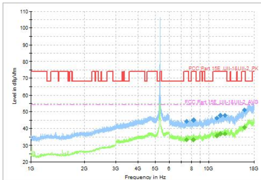
Fig. 85 Transmitter Spurious Emission (802.11a, CH64 5320MHz, 1 GHz-18 GHz)
