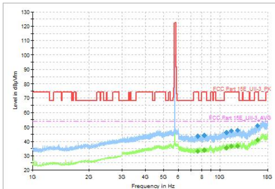
Fig. 89 Transmitter Spurious Emission (802.11a, CH149 5745MHz, 1 GHz-18 GHz)
