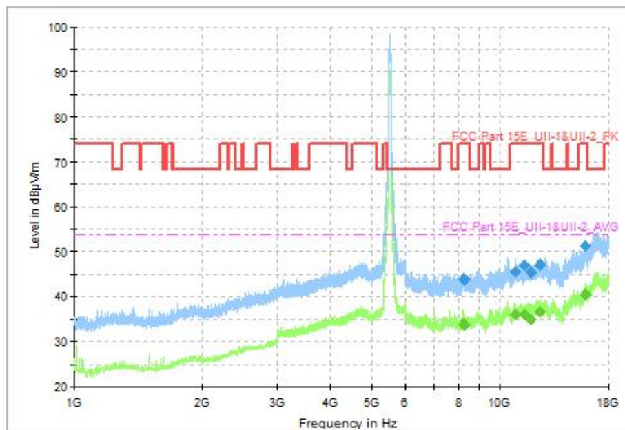
Fig. 103 Transmitter Spurious Emission (802.11ac-VHT80, CH106 5530MHz, 1 GHz-18 GHz)
