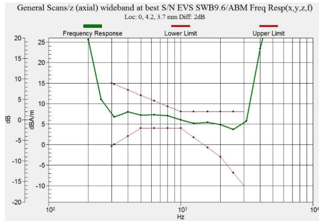
Figure C.4 Frequency Response of EPDG 1900 - OTT VoIP
