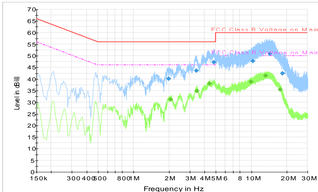
Fig.A.11.3 AC Powerline Conducted Emission- Bluetooth TN-050100U6 (Guangdong Beicom Electronics Co.,Ltd.)
