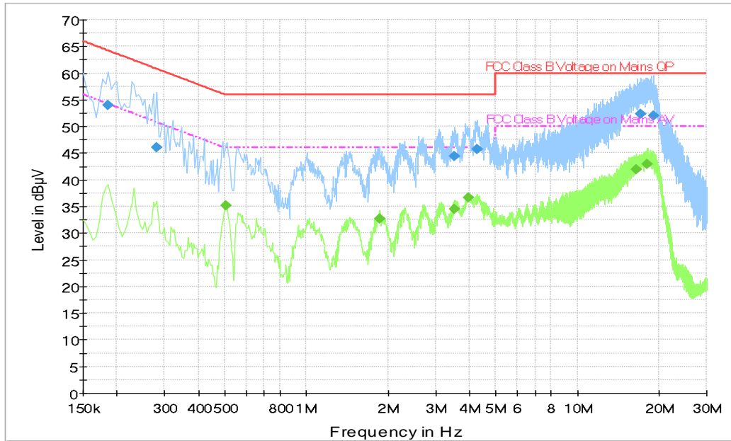
Fig.A.7.2 AC Powerline Conducted Emission-Idle TN-050100U6 (Dong Guan City GangQi Electronic CO.,Ltd.)
