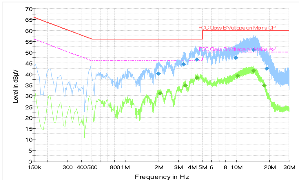
Fig.A.7.3 AC Powerline Conducted Emission-802.11b TN-050100U6 (Guangdong Beicom Electronics Co.,Ltd.)
