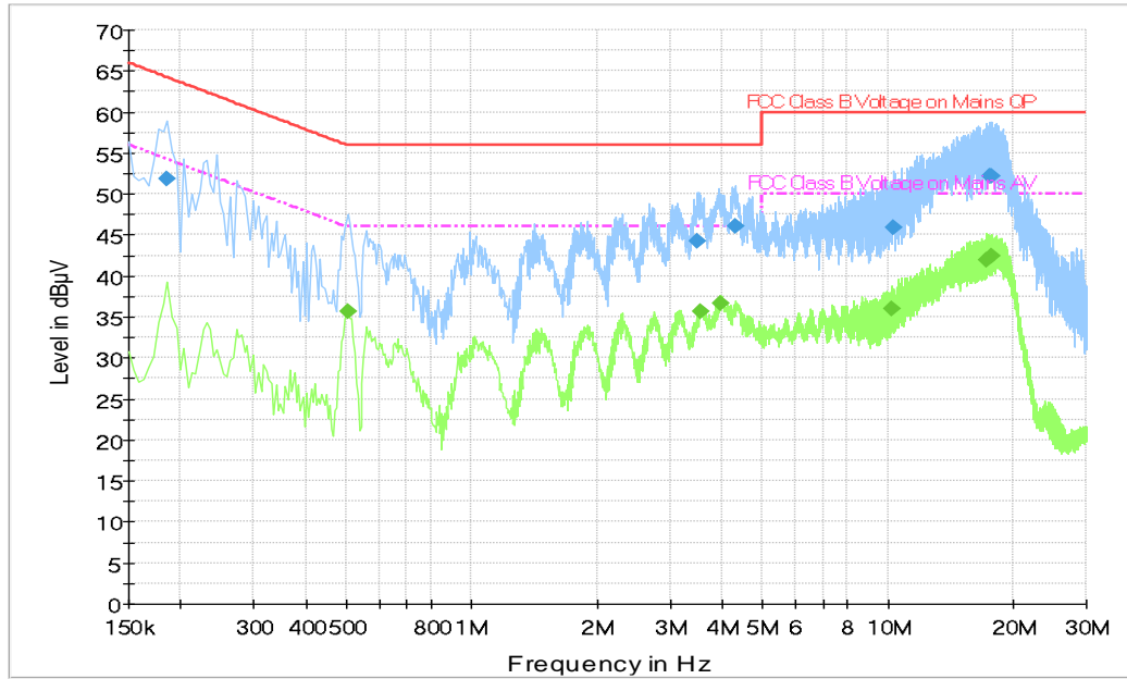
Fig.A.7.1 AC Powerline Conducted Emission-802.11b TN-050100U6 (Dong Guan City GangQi Electronic CO.,Ltd.)
