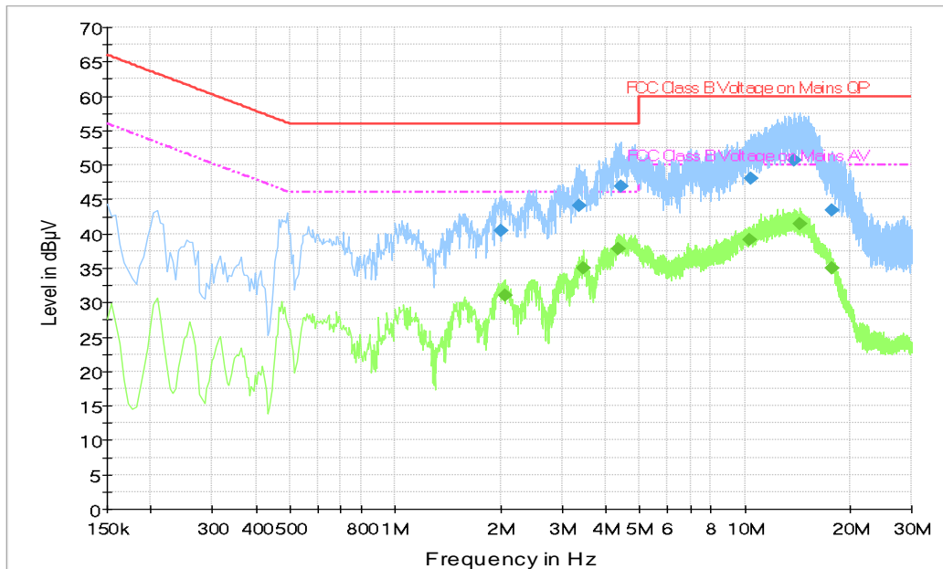
Fig.A.7.4 AC Powerline Conducted Emission-Idle TN-050100U6 (Guangdong Beicom Electronics Co.,Ltd.)
