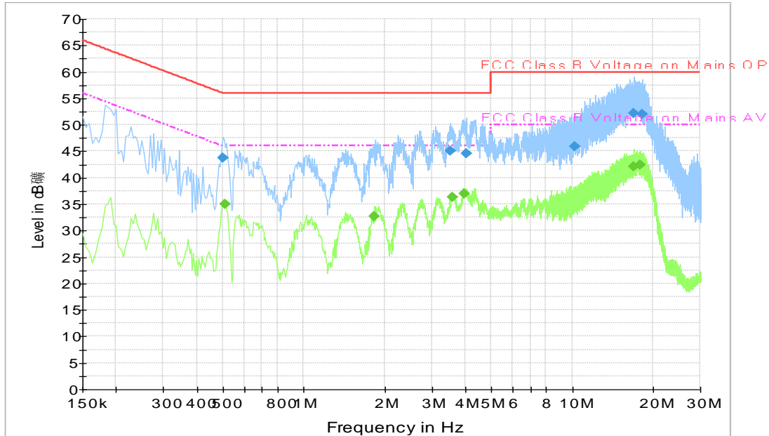
Fig.A.9.2 AC Powerline Conducted Emission-Idle TN-050100U6 (Dong Guan City GangQi Electronic CO.,Ltd.)
