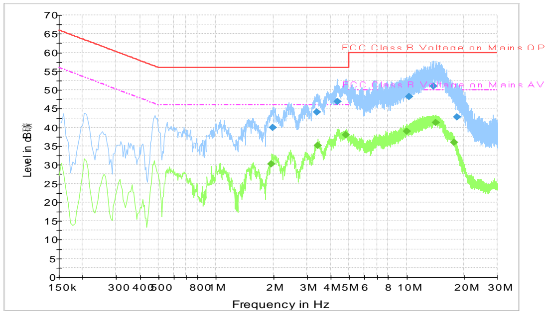
Fig.A.9.4 AC Powerline Conducted Emission-Idle TN-050100U6 (Guangdong Beicom Electronics Co.,Ltd.)
