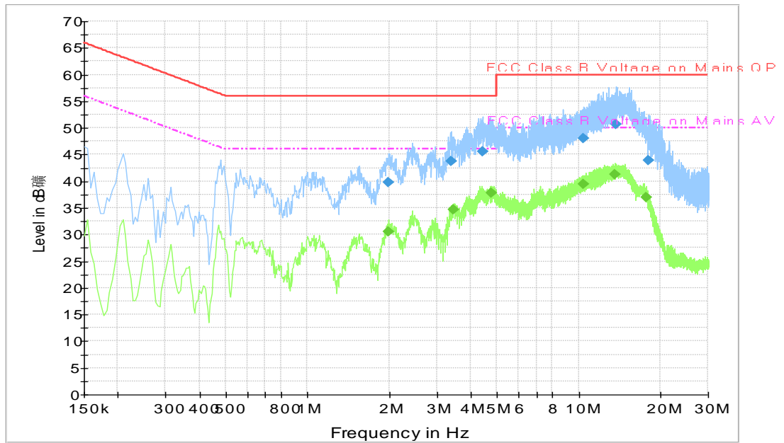
Fig.A.9.3 AC Powerline Conducted Emission- BLE TN-050100U6 (Guangdong Beicom Electronics Co.,Ltd.)
