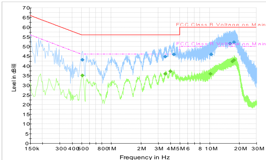
Fig.A.9.1 AC Powerline Conducted Emission- BLE TN-050100U6 (Dong Guan City GangQi Electronic CO.,Ltd.)
