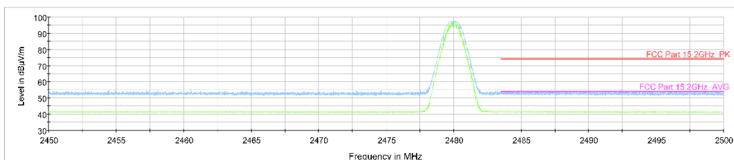
Fig.14. Frequency Band Edges: GFSK, Channel 78, Hopping Off, ch11, 2.45 GHz - 2.50GHz
