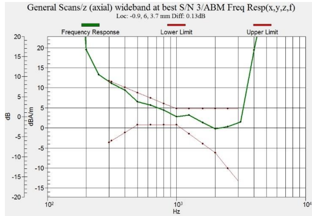
Figure C.1 Frequency Response of LTE B14
