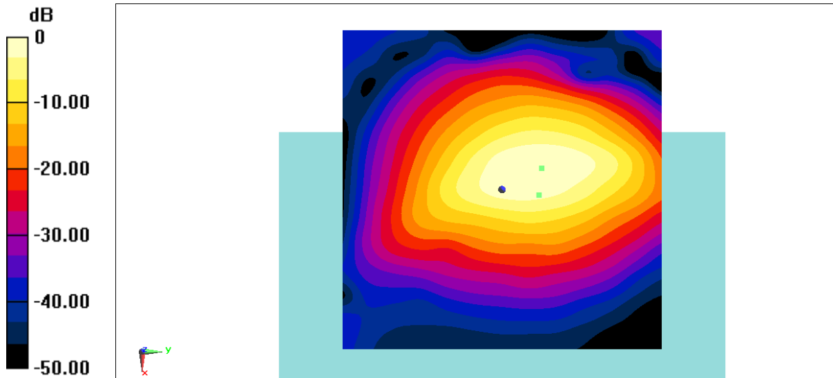
Fig B.4 T-Coil WiFi-5G
