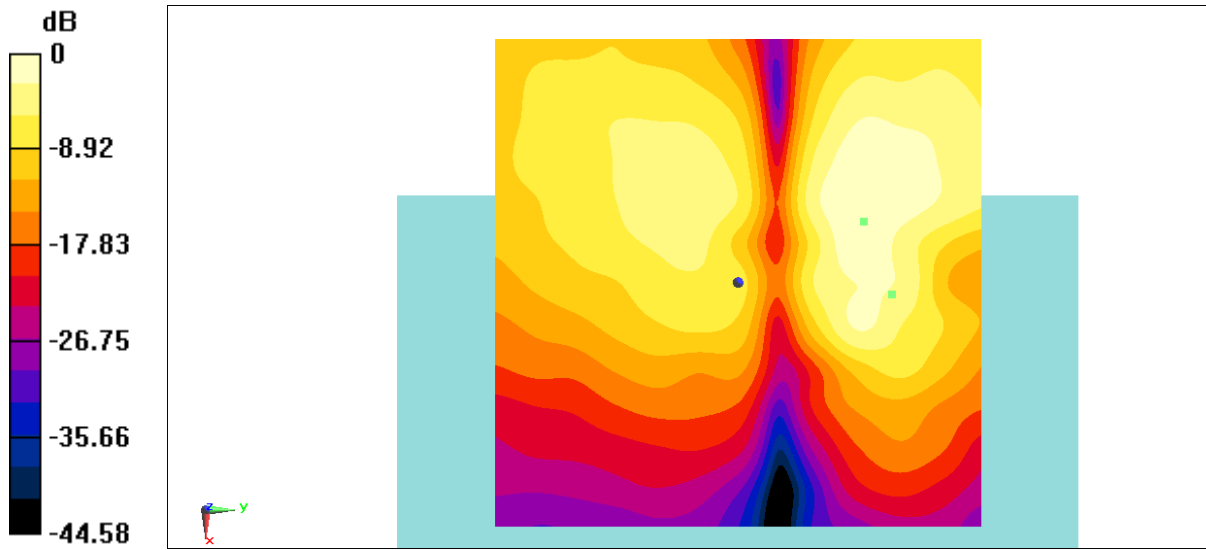
Fig B.1 T-Coil WiFi-2.4G
