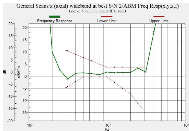
Figure C.2 Frequency Response of WiFi-5G - OTT VoIP
