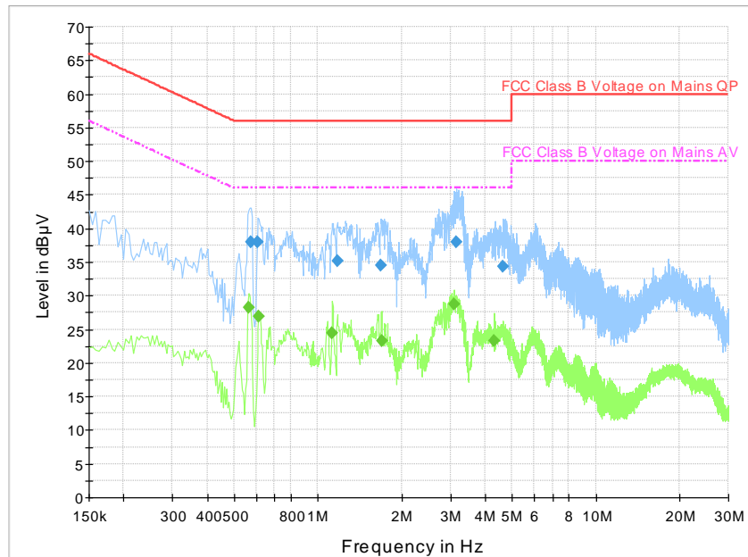
Fig.B.9.1 AC Powerline Conducted Emission-blutetooth
