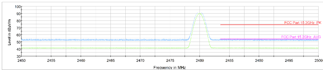
Fig.4. Frequency Band Edges: GFSK, 2480 MHz, Hopping Off, 2.45 GHz - 2.50GHz
