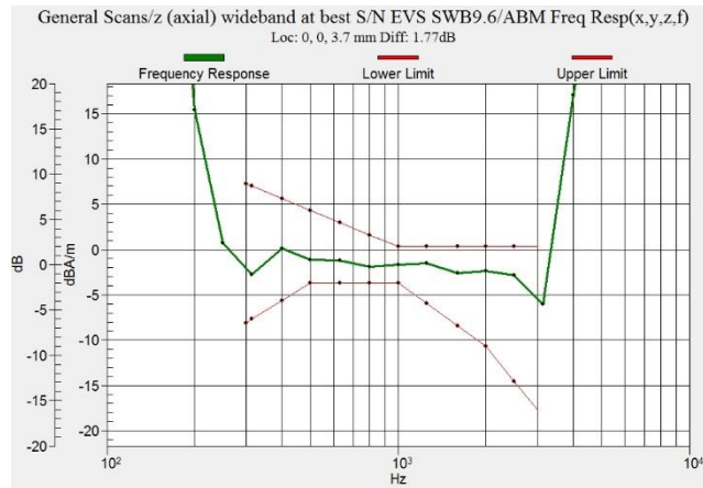
Figure C.4 Frequency Response of EPDG 850 - OTT VoIP
