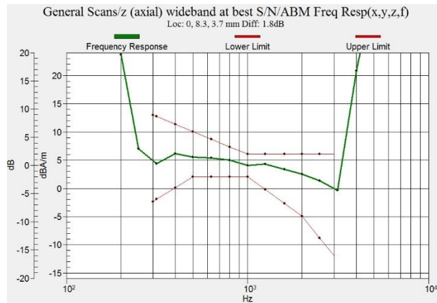
Figure C.5 Frequency Response of LTE B7 - OTT VoIP
