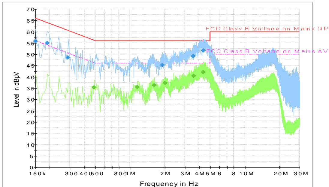
Fig.A.7.1 AC Powerline Conducted Emission- BLE
