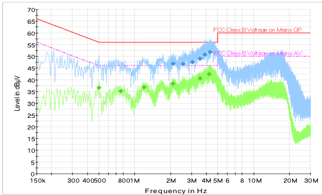
Fig.A.7.4 AC Powerline Conducted Emission-Idle
