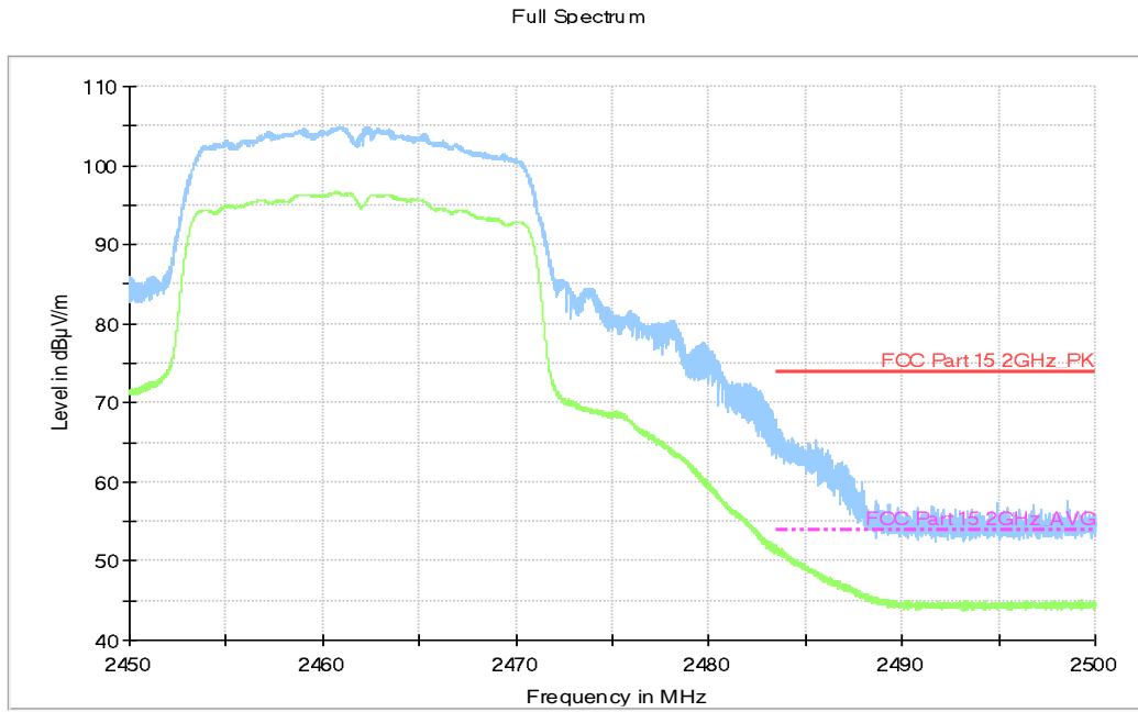
Fig.A.5.2.6 Transmitter Spurious Emission - Radiated Band edge: 802.11n-HT20, ch11, 2.45 GHz - 2.50GHz
