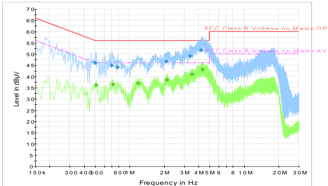
Fig.A.7.1 AC Powerline Conducted Emission- bluetooth
