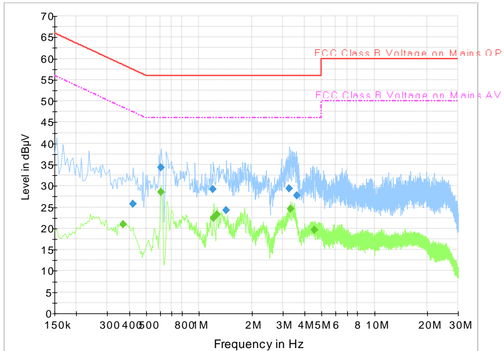
Fig.B.9.2 AC Powerline Conducted Emission-Idle
