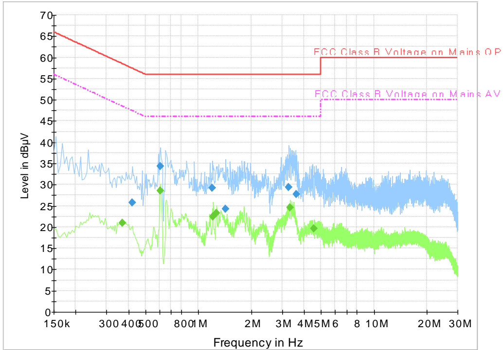
Fig.B.11.2 AC Powerline Conducted Emission-Idle
