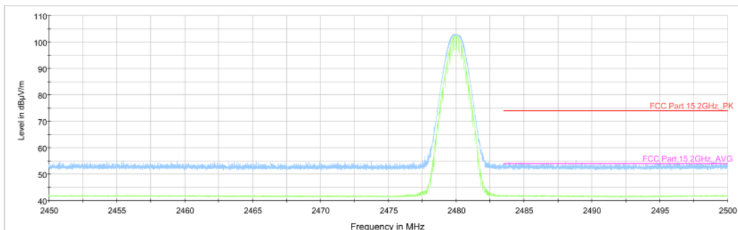
Fig.14. Frequency Band Edges: GFSK, Channel 78, Hopping Off, 2.45 GHz - 2.50GHz
