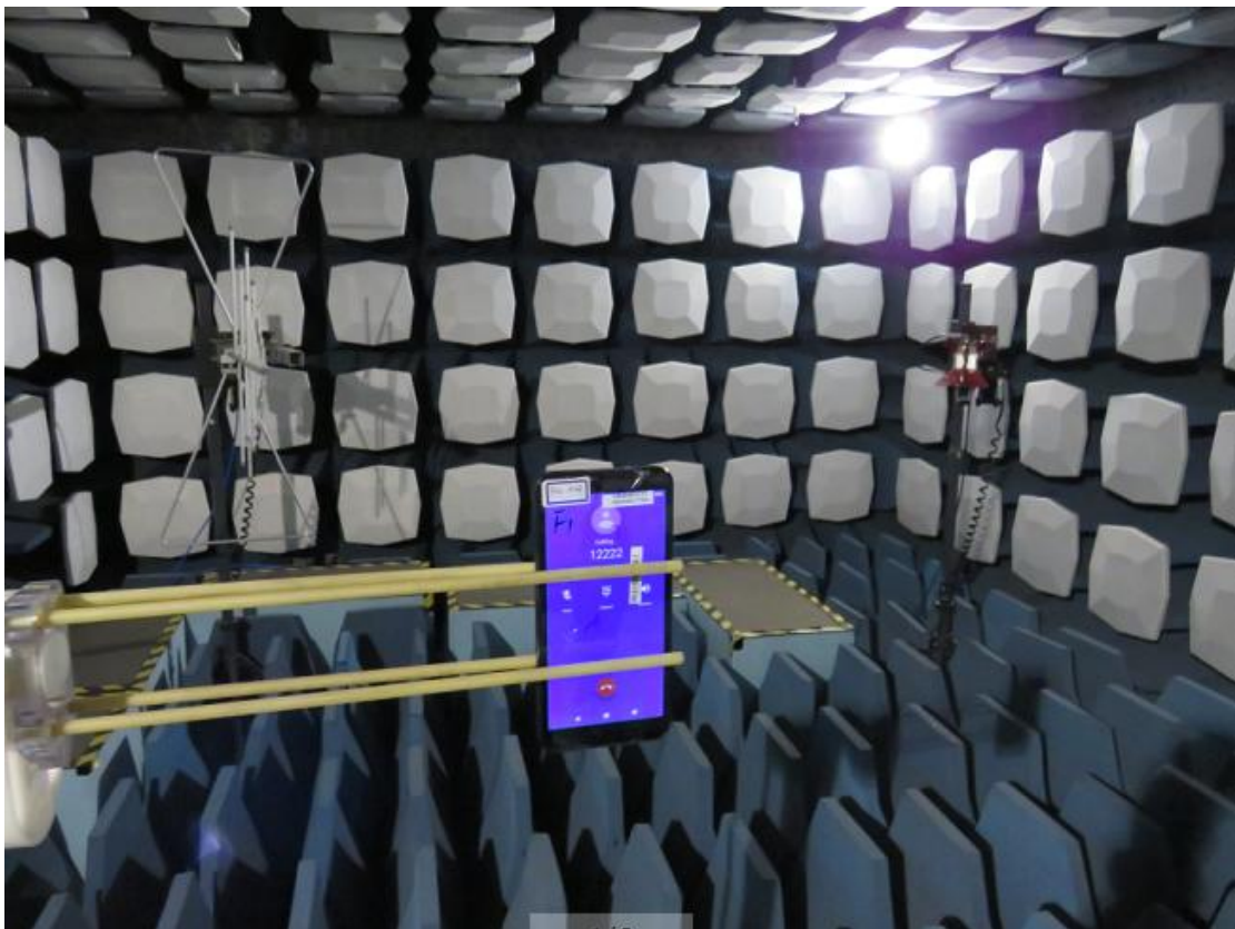
Radiated Spurious Emission and Output Power
