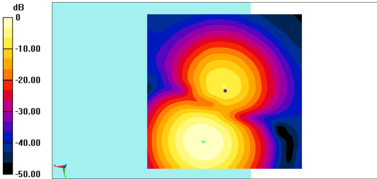
Fig B.2 T-Coil LTEB2
