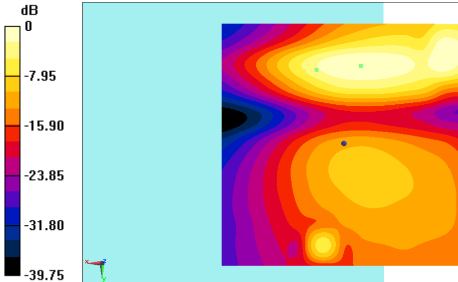
Fig B.1 T-Coil LTEB2
