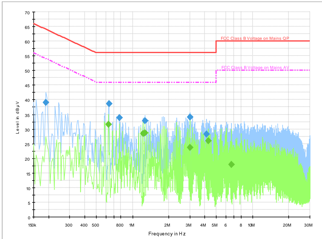
Fig.B.9.2 AC Powerline Conducted Emission-Idle, TN-050120U9
