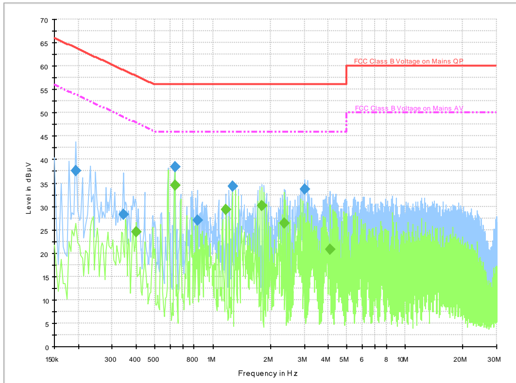
Fig.B.9.1 AC Powerline Conducted Emission- Bluetooth, TN-050120U9
