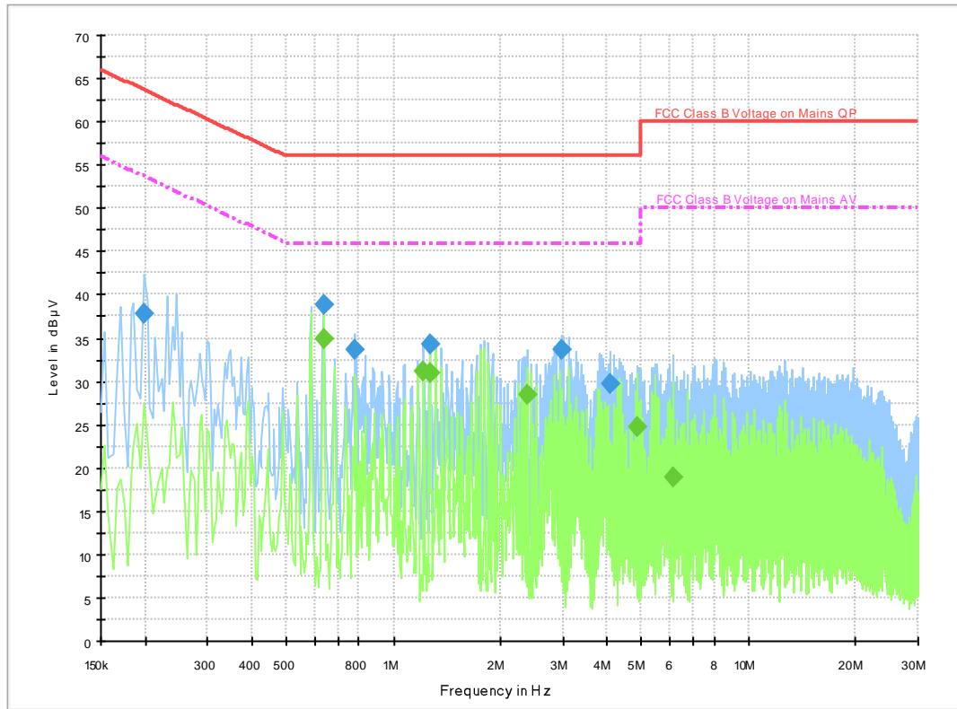
Fig.B.9.3 AC Powerline Conducted Emission- Bluetooth, TN-050120U8
