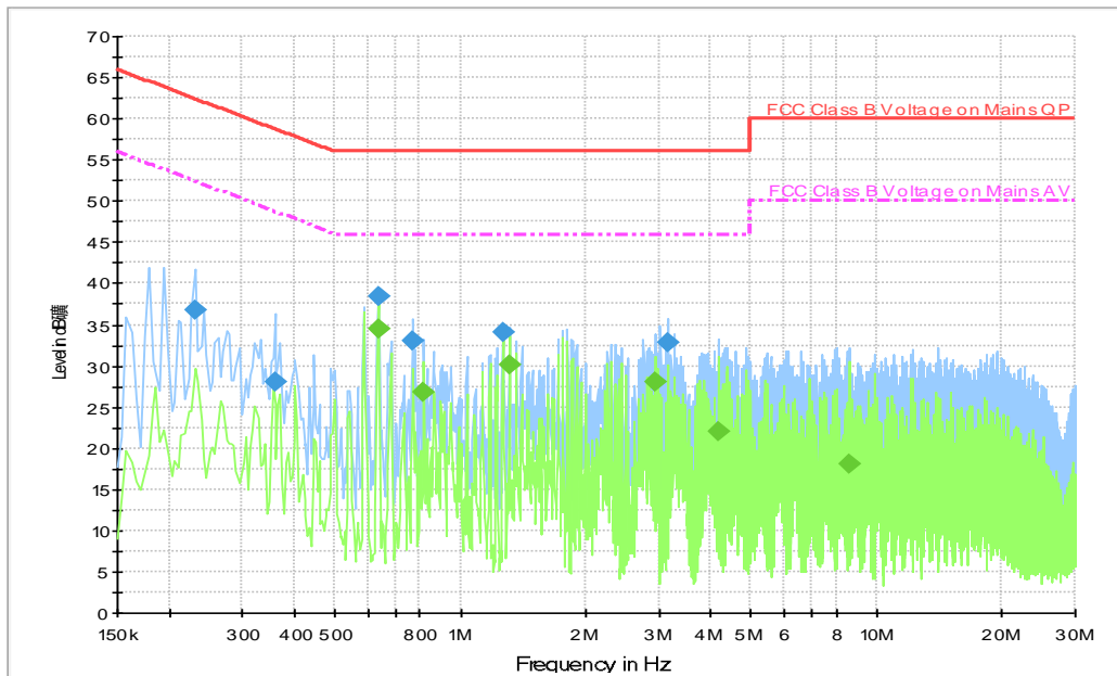
Fig.A.7.3 AC Powerline Conducted Emission-802.11b, TN-050120U8
