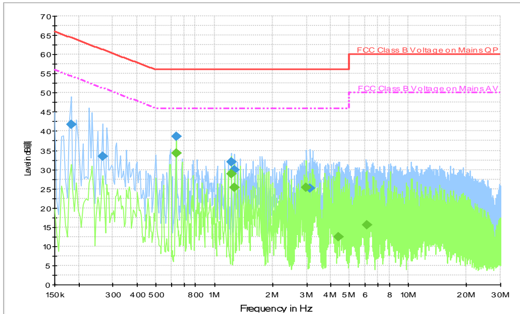
Fig.A.7.1 AC Powerline Conducted Emission-802.11b, TN-050120U9
