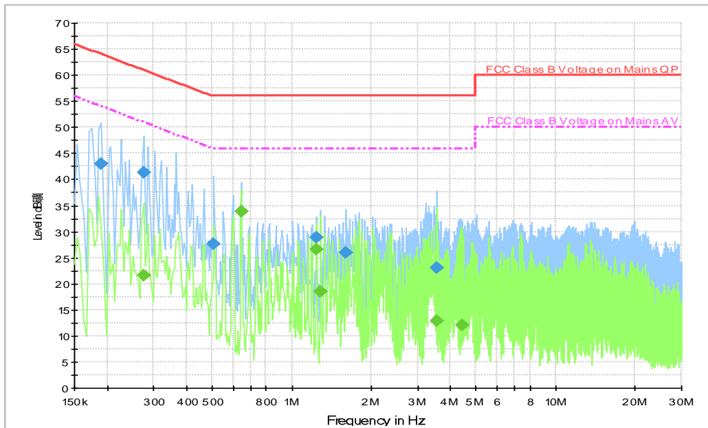
Fig.A.7.2 AC Powerline Conducted Emission-Idle, TN-050120U9
