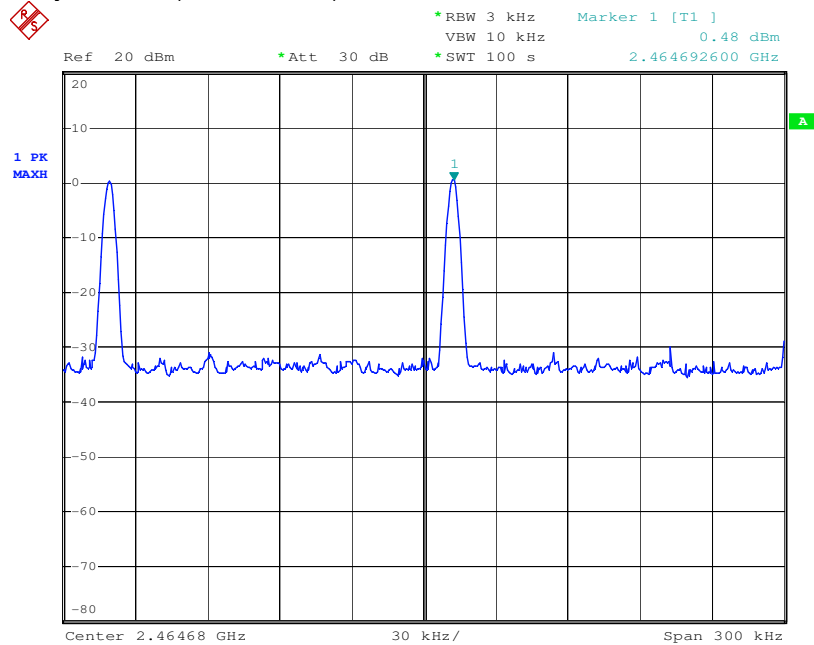
Power Spectral Density Test Plot(CH 2464MHz)
