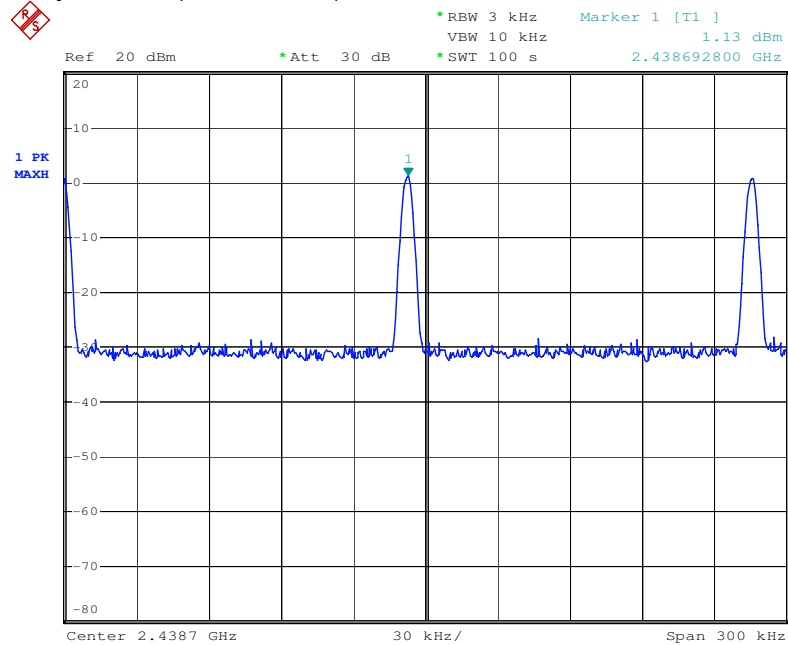
Power Spectral Density Test Plot(CH 2438MHz)
