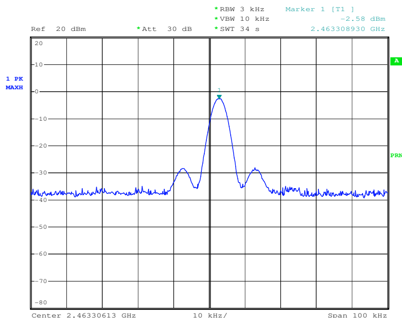
Power Spectral Density Test Plot(CH-High)
