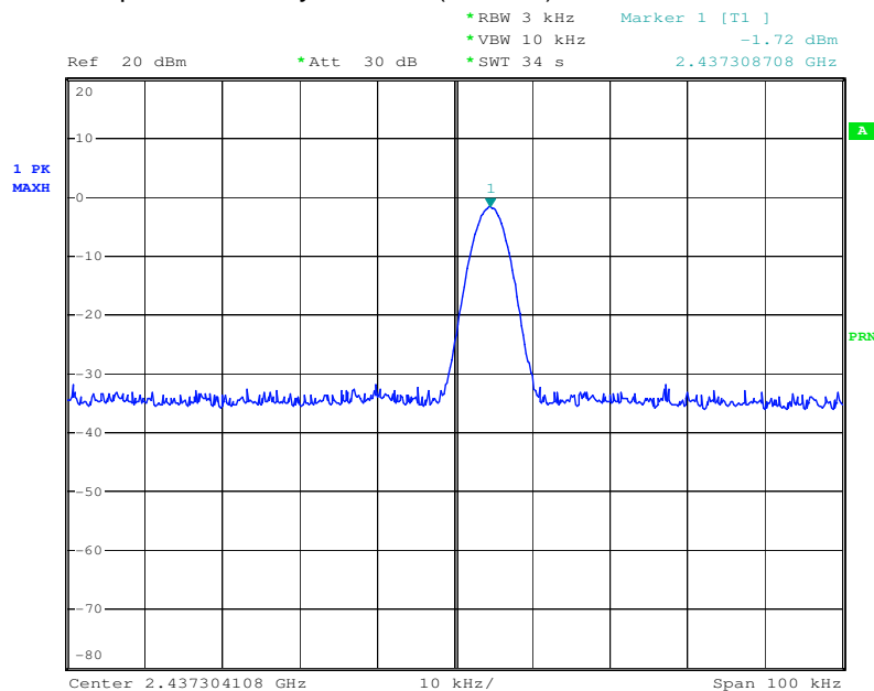
Power Spectral Density Test Plot(CH-Mid)
