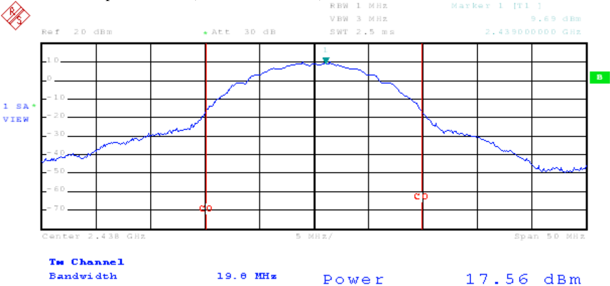
Peak Power Output Data Plot(CH Mid 2438MHz)
