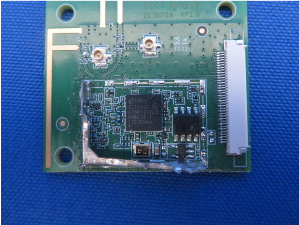
(1) DECT Modular Photo (with External Antenna connector)
