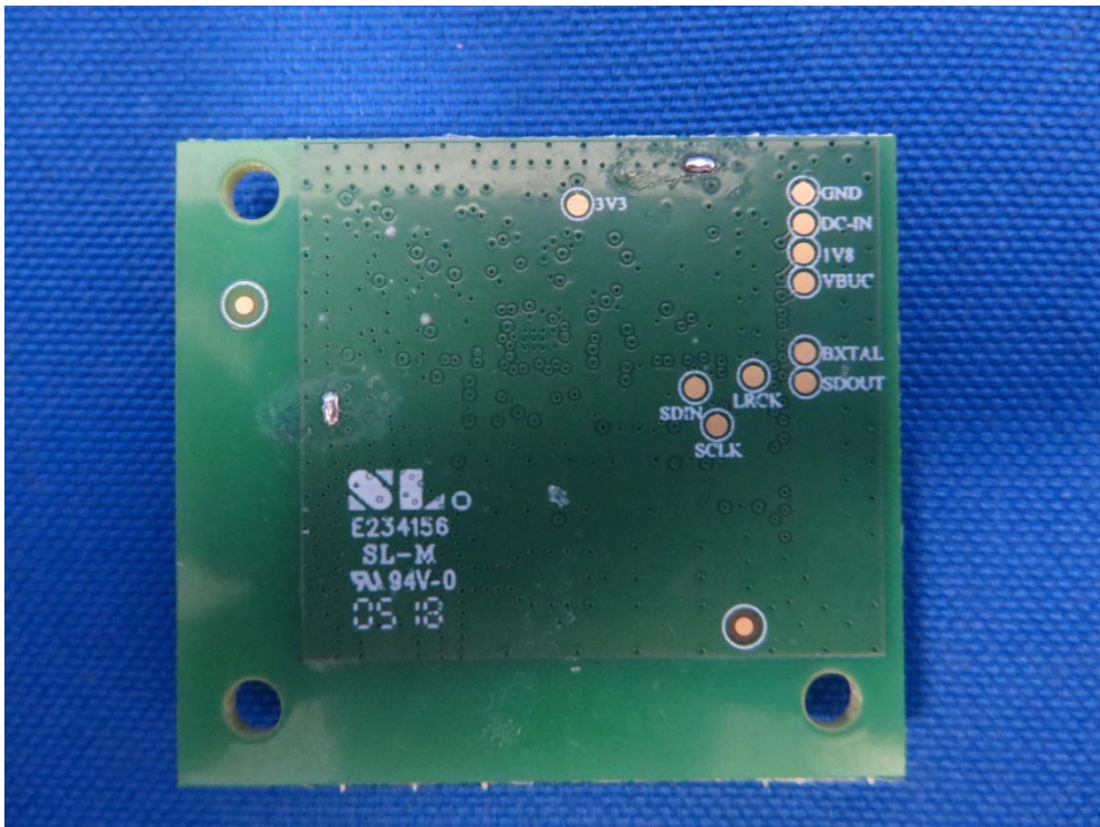
(2) DECT Modular Photo (with External Antenna connector)
