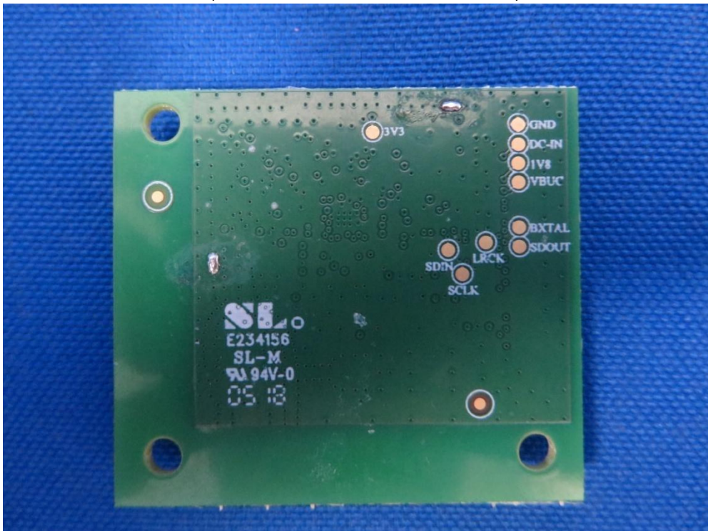
(4) DECT Modular Photo (with External Antenna connector)
