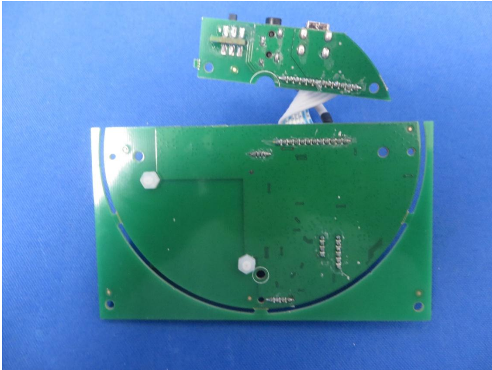
(2) DECT Modular & Test Fixture Photo (with External Antenna connector)
