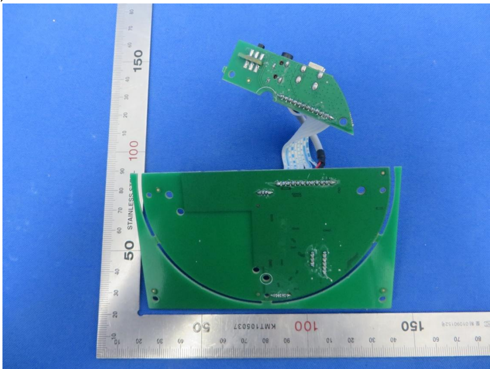
(10) Test Fixture Photo
