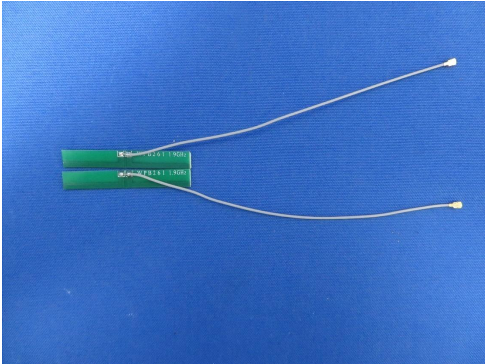
(11) EUT Photo (Monopole Antenna)
