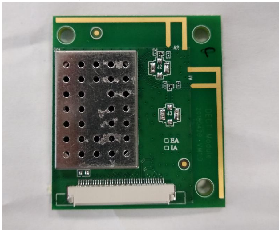
(7) DECT Modular Photo (without External Antenna connector)
