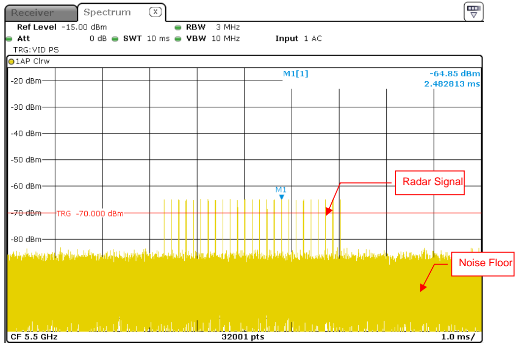
Radar Signal 2
