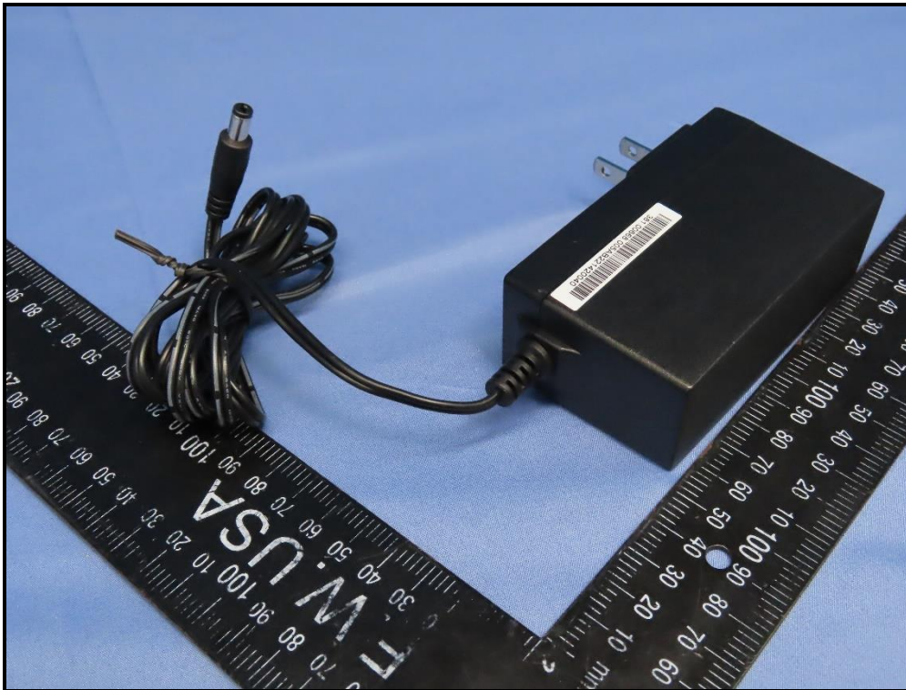
Adapter (Brand: I.T.E, Model: MU48AY120400-A1)
