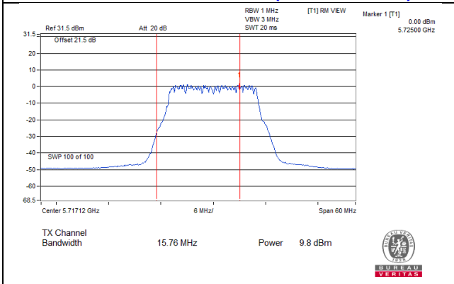
802.11a_Chain 3 / CH144 (U-NII-2C Band)
