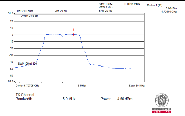
802.11a_Chain 1 / CH144 (U-NII-3 Band)
