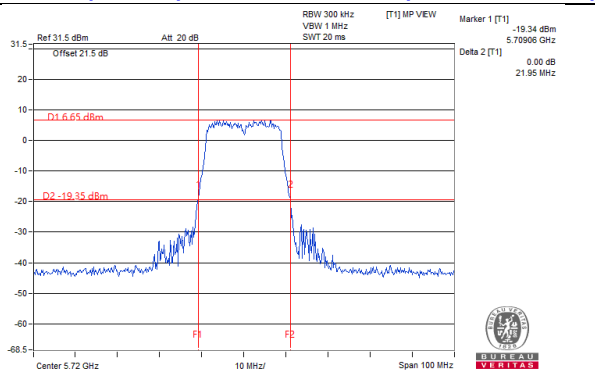
802.11ac (VHT20)_Chain 3 / CH144 (U-NII-2C Band)
