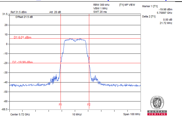
802.11a_Chain 2 / CH144 (U-NII-2C Band)
