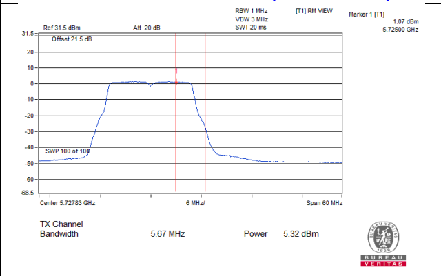
802.11a_Chain 3 / CH144 (U-NII-3 Band)
