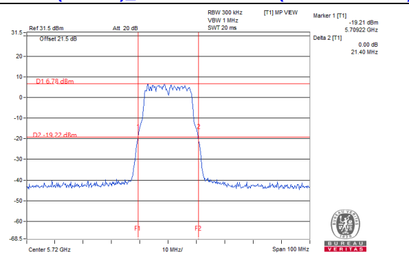
802.11ac (VHT20)_Chain 2 / CH144 (U-NII-2C Band)
