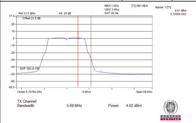
802.11a_Chain 2 / CH144 (U-NII-3 Band)
