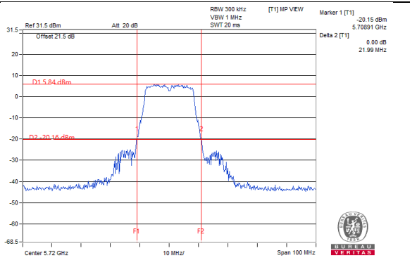
802.11a_Chain 1 / CH144 (U-NII-2C Band)
