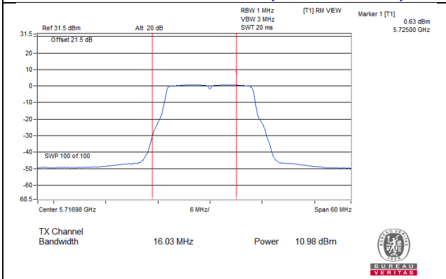
802.11a_Chain 2 / CH144 (U-NII-2C Band)
