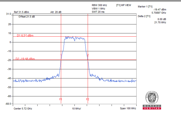
802.11ac (VHT20)_Chain 1 / CH144 (U-NII-2C Band)
