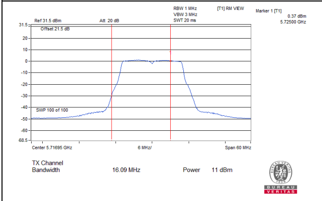
802.11a_Chain 1 / CH144 (U-NII-2C Band)
