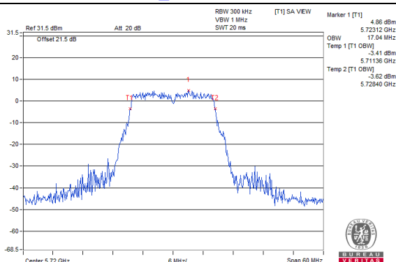
802.11a_Chain 1 / CH144
