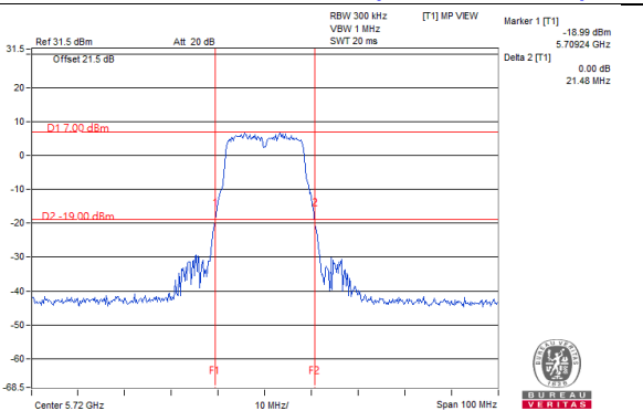
802.11a_Chain 3 / CH144 (U-NII-2C Band)
