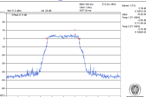
802.11a_Chain 3 / CH144
