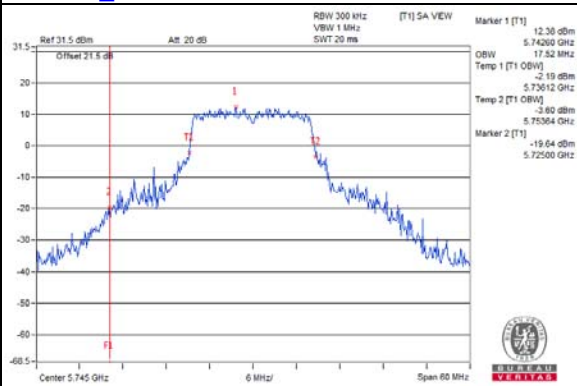
802.11a_Chain 3 / CH149
