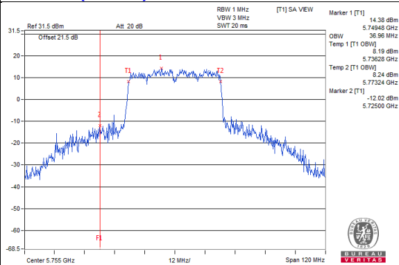
802.11ac(VHT40)_Chain1 / CH151
