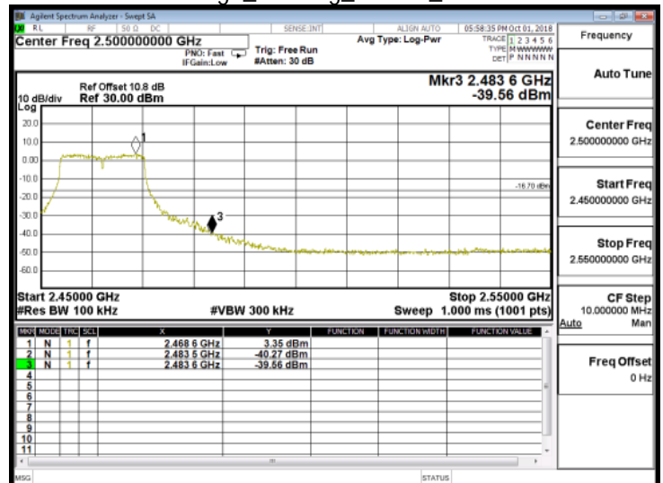
Band Edge_802.11g_Chain0_2462MHz
