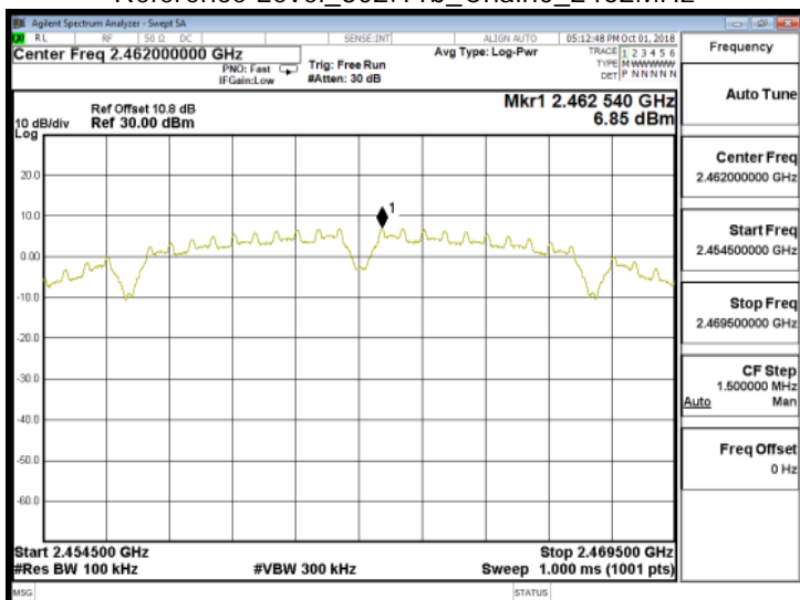
Reference Level_802.11b_Chain0_2462MHz
