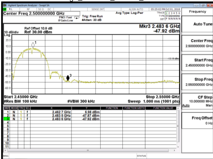
Band Edge_802.11b_Chain0_2462MHz
