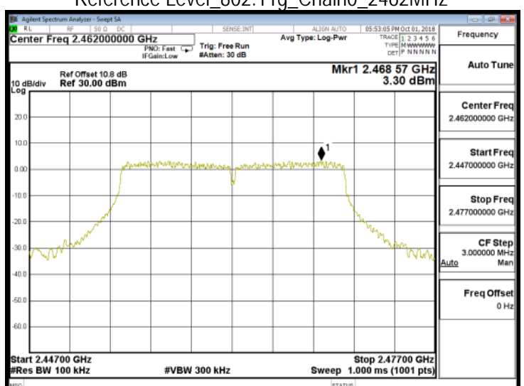
Reference Level_802.11g_Chain0_2462MHz
