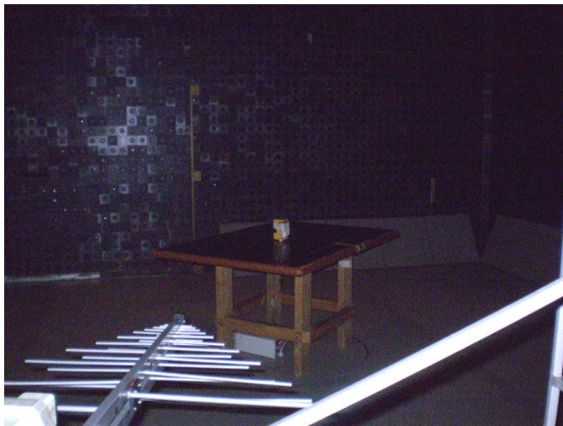
Photograph No.2 Setup for spurious emission measurements in the anechoic chamber from 30 to 1000 MHz
